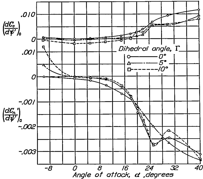
FIGURE 21.—Effect of dihedral of 93 percent semispan of rectangular wing on rate of change of cross-wind force and yawing-moment coefficients with angle of yaw.
