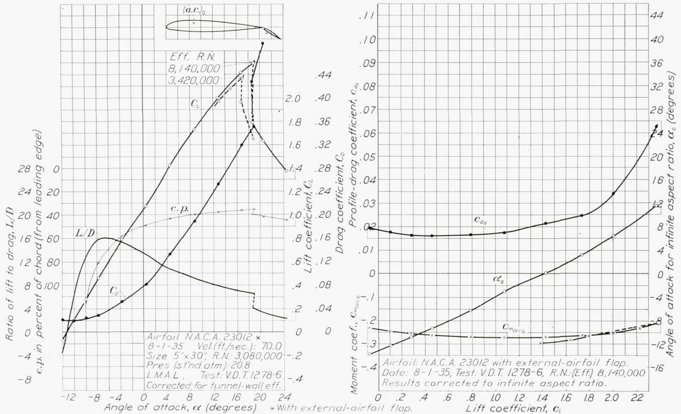
FIGURE 17.—The N. A. C. A. 23012 airfoil with 0.20c w N. A. C. A. 23012 external-airfoil flap. Flap angle, 30°. The airfoil is the same as used for variable-density tunnel test 1272 (fig. 14) except the flap setting. The value of c_{m(a.c.)_0} is computed about the aerodynamic center as determined for test 1273.
