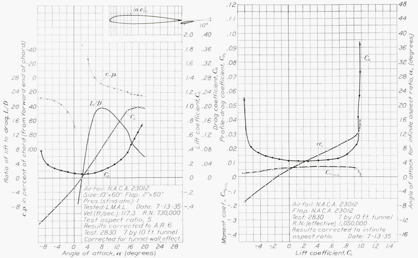
FIGURE 5.—The N. A. C. A. 23012 airfoil with 0.20c w N. A. C. A. 23012 external-airfoil flap. Flap angle, -10°. The airfoil is the same as used for test 2831-a (fig. 6), except the flap setting. The value of C m(a.c.) 0 is computed about the aerodynamic center used for test 2831-a.
