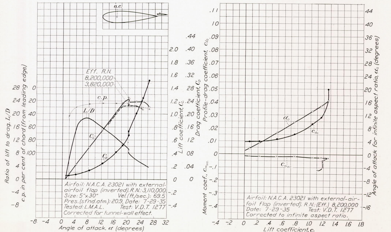
FIGURE 20.—The N. A. C. A. 23021 airfoil with 0.20 c_w N. A. C. A. 23012 external-airfoil flap. Flap angle, -3^\circ (inverted). The airfoil is the same as used for variable-density tunnel test 1274 (fig. 19) except inverted; a. c. from leading edge, 0.217c; a. c. above main wing chord, -0.01c .
