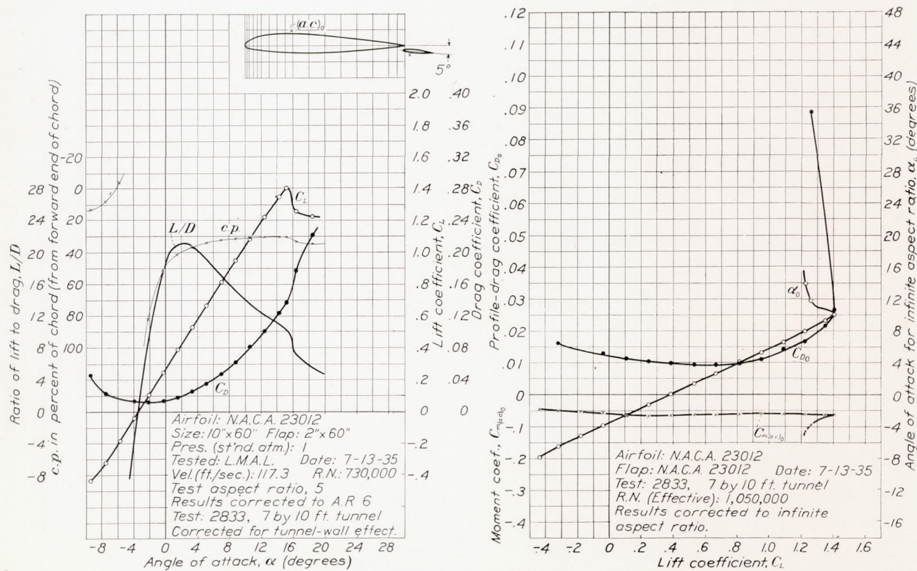
FIGURE 8.—The N. A. C. A. 23012 airfoil with 0.20c w N. A. C. A. 23012 external-airfoil flap. Flap angle, 5°. The airfoil is the same as used for test 2831-a (fig. 6), except the flap setting. The value of C m(a.c.) 0 is computed about the aerodynamic center used for test 2831-a.
