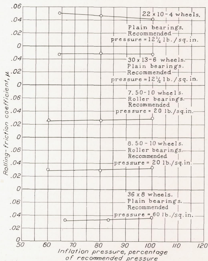
FIGURE 7.—Variation of rolling-friction coefficient with inflation pressure; firm turf surface; load per wheel, 940 pounds.
