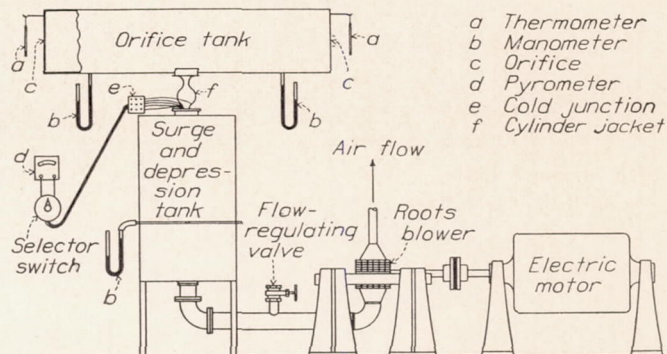
(b) Equipment used to test the 0.166-1.22-0.035, 0.137-1.22-0.035, 0.112-1.22-0.035, 0.083-1.22-0.035, and 0.057-1.22-0.035 cylinders.
