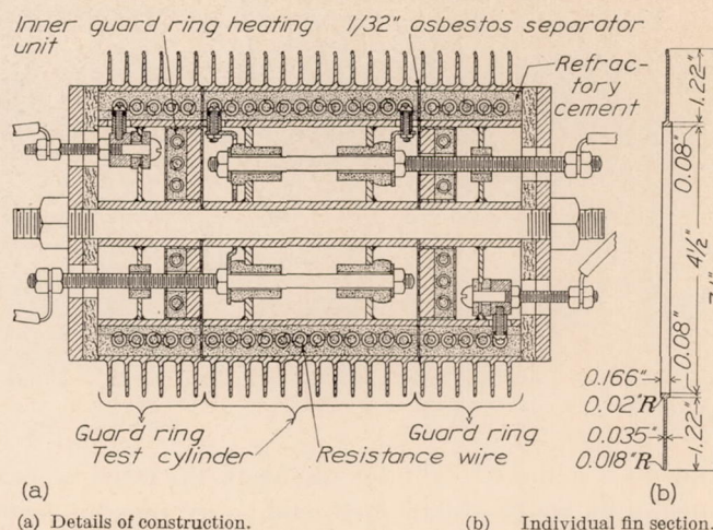
FIGURE 1.—Construction of test unit.
