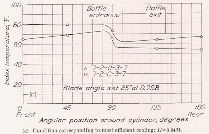
FIGURE 22.—Temperature distribution around the electrically heated cylinder.
