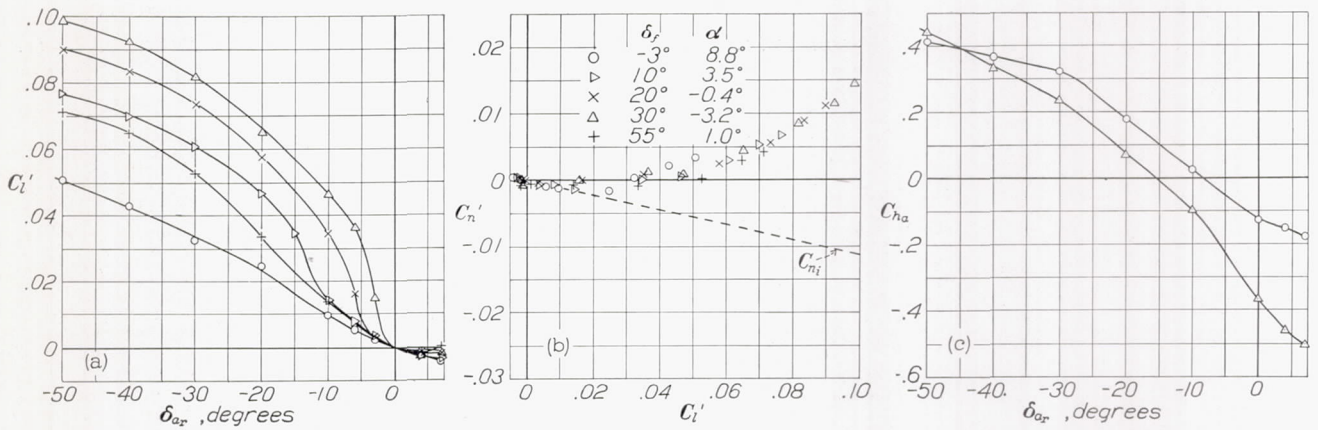
(a) Variation of rolling-moment coefficient with deflection of right aileron. Left aileron, 0^\circ . (b) Variation of yawing-moment coefficient with rolling-moment coefficient. (c) Variation of aileron hinge-moment coefficient with aileron deflection.
