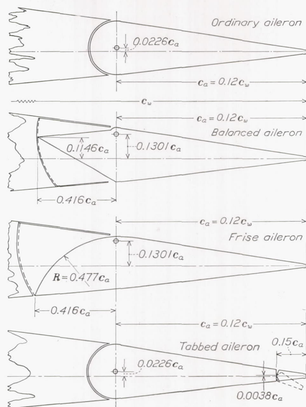
FIGURE 3.—Various balanced ailerons tested on the wide-chord N. A. C. A. 23012 airfoil with and without a 0.20 c_w N. A. C. A. 23012 external-airfoil flap.
