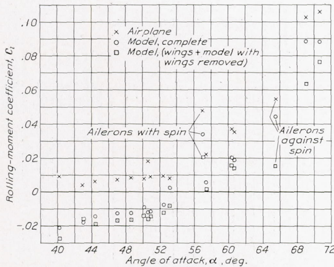
FIGURE 29.—Variation of rolling-moment coefficient C_l (body axes) of airplane and model with angle of attack.
