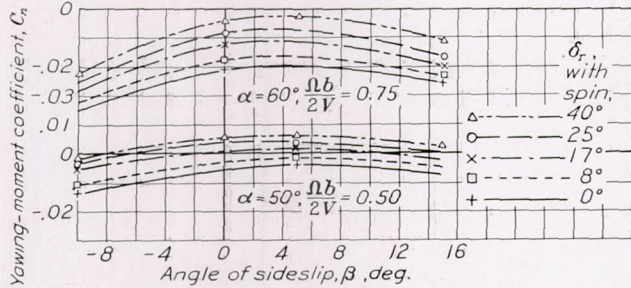
FIGURE 22.—Variation of yawing-moment coefficient C_n (body axes) with rudder setting. \delta_a=0^\circ ; \delta_e=23^\circ 41' up.
