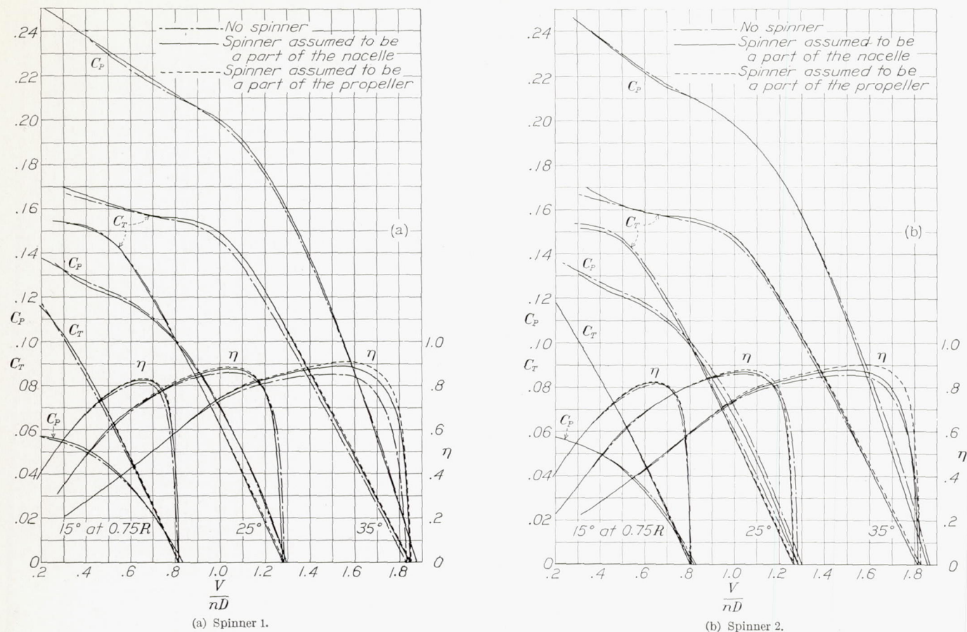
FIGURE 42.—Effect of spinner on propeller characteristics. Propeller 5868-9, 3 blades, liquid-cooled engine nacelle.
