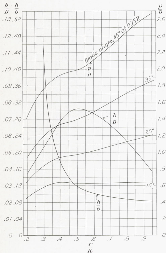
FIGURE 7.—Blade-form curves for propeller 5868-9.
