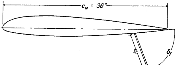
FIGURE 1.—Section of N. A. C. A. 23012 airfoil with split flaps. c_f = 0.10c_w, 0.20c_w, 0.30c_w, and 0.40c_w .
