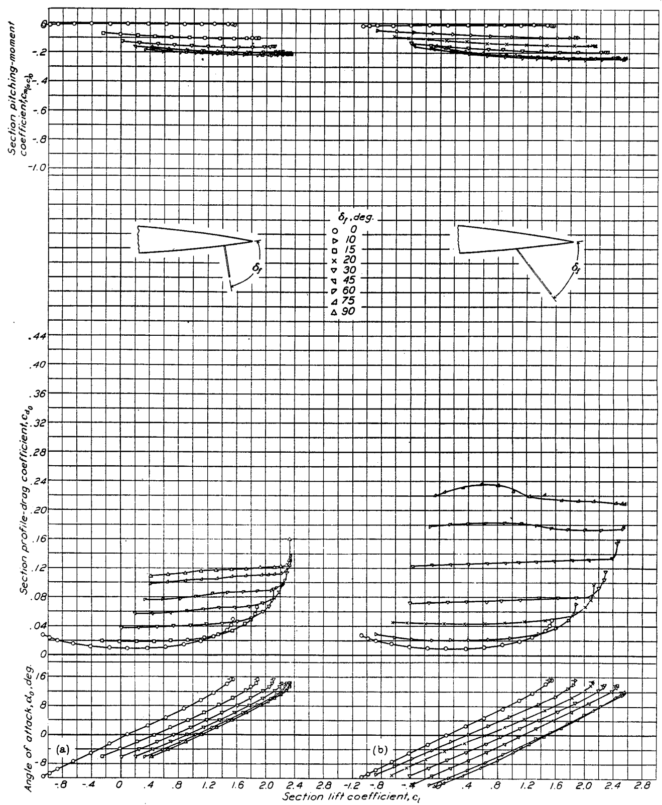
(a) The 0.10 c_w split flap. (b) The 0.20 c_w split flap
