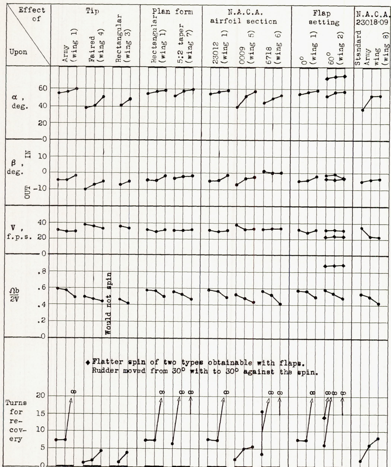
FIGURE 15.—The effect of various wings on the spin characteristics. (Wing has rectangular plan form. Army tips, N. A. C. A. 23012 section, except as noted.) Center-of-gravity location at 15, 25, and 35 percent mean chord, plotted left to right; tail C; rudder 30° with; elevators 20° down.
