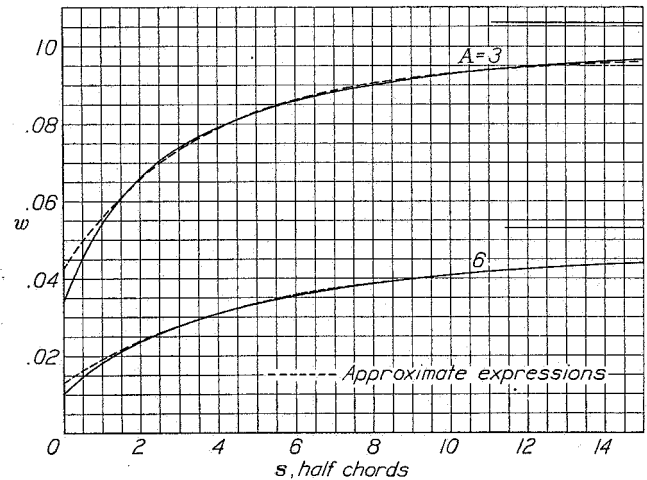
FIGURE 7.—Downwash functions, w_i(s) .
