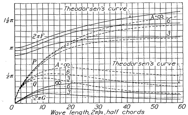
FIGURE 11.—Oscillating-lift functions, \bar{C}_{L_\alpha}(in) = 2\pi(F + iG) and \bar{C}_{L_\beta}(in) = P + iQ .
