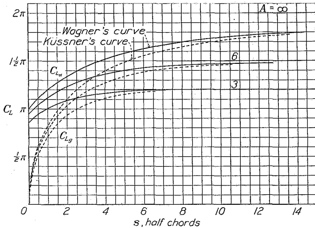
FIGURE 9.—Indicial lift functions, C_{L_\alpha}(s) and C_{L_\beta}(s) .
