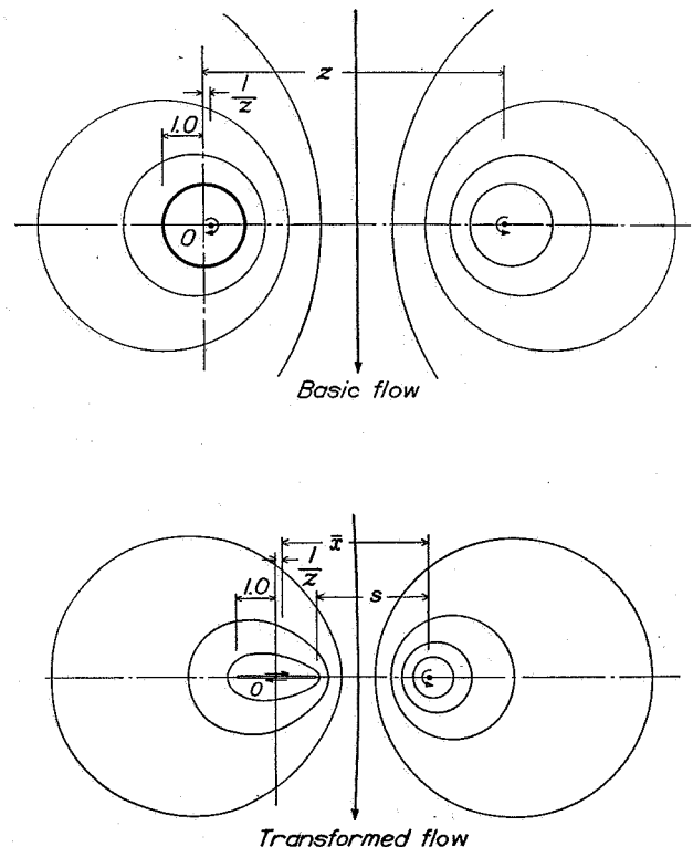
FIGURE 3.—Element of circulatory flow.
