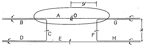
FIGURE 5.—Superposition of vortices to obtain finite loop.
