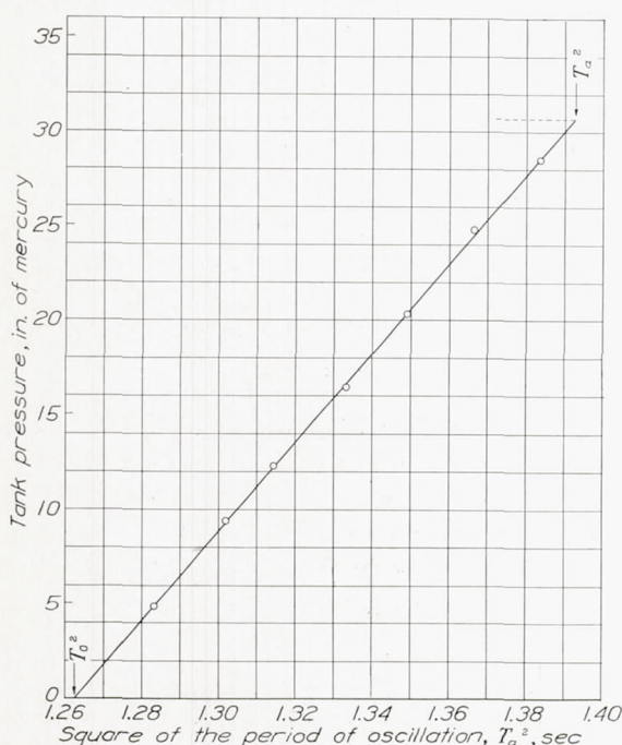
FIGURE 11.—Variation of T_0^2 with tank pressure for plate of aspect ratio 8. (1940 NACA tests.)
