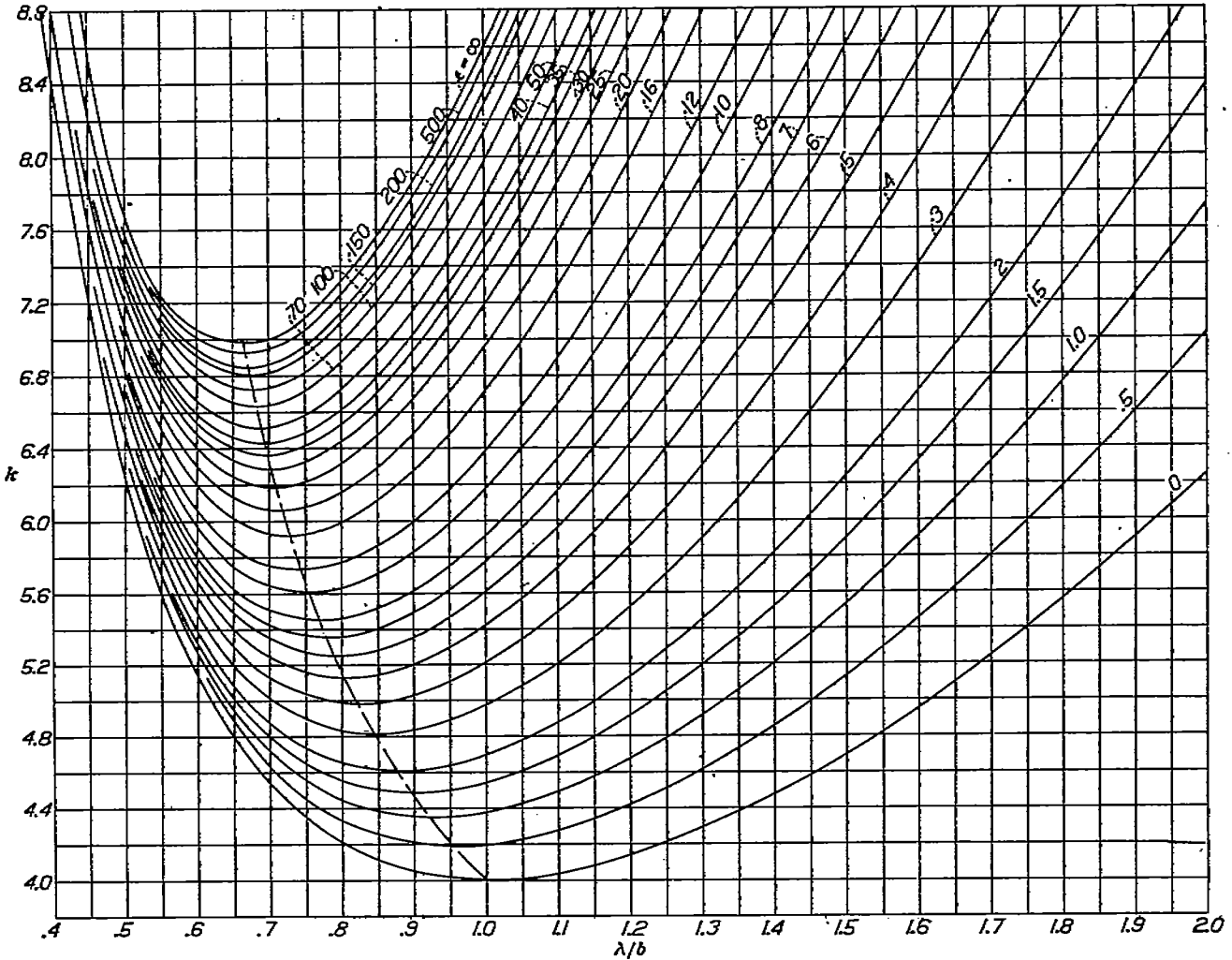
FIGURE 3.—General design chart giving values of k for equal restraint coefficients \epsilon on each side edge of the plate. f_{cr} = \frac{k\pi^2 EI^2}{12(1-\mu^2)bt^3}
