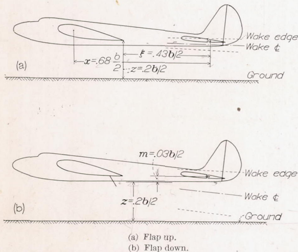
FIGURE 12.—Illustration for the specimen calculations of downwash and wake.
