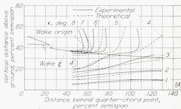
(d) With full-span 0.20c split flap deflected 60^\circ ; C_L , 1.6; z/\bar{c} , 1.18.
