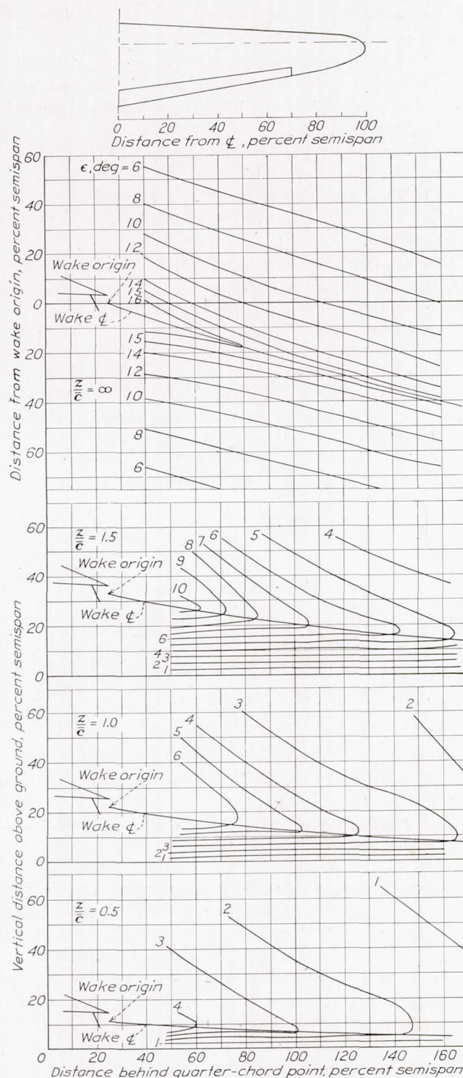
FIGURE 10.—Theoretical downwash-angle contours and wake positions for various distances from ground. A, 9; taper ratio, 3:1. 0.7-span flap; CL_{up} , 1.2; CL_f , 1.2.
