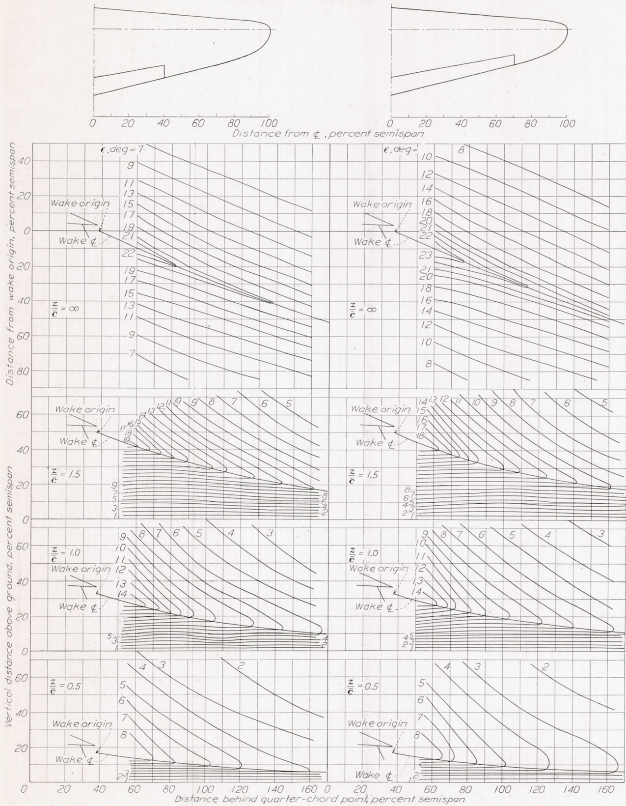
0.4-span flap; CL_{u0} , 1.2; CL_F , 0.6 0.7 span flap; CL_{u0} , 1.2; CL_F , 1.2 FIGURE 8.—Theoretical downwash-angle contours and wake positions for various distances from ground. A, 6; taper ratio, 3:1.
