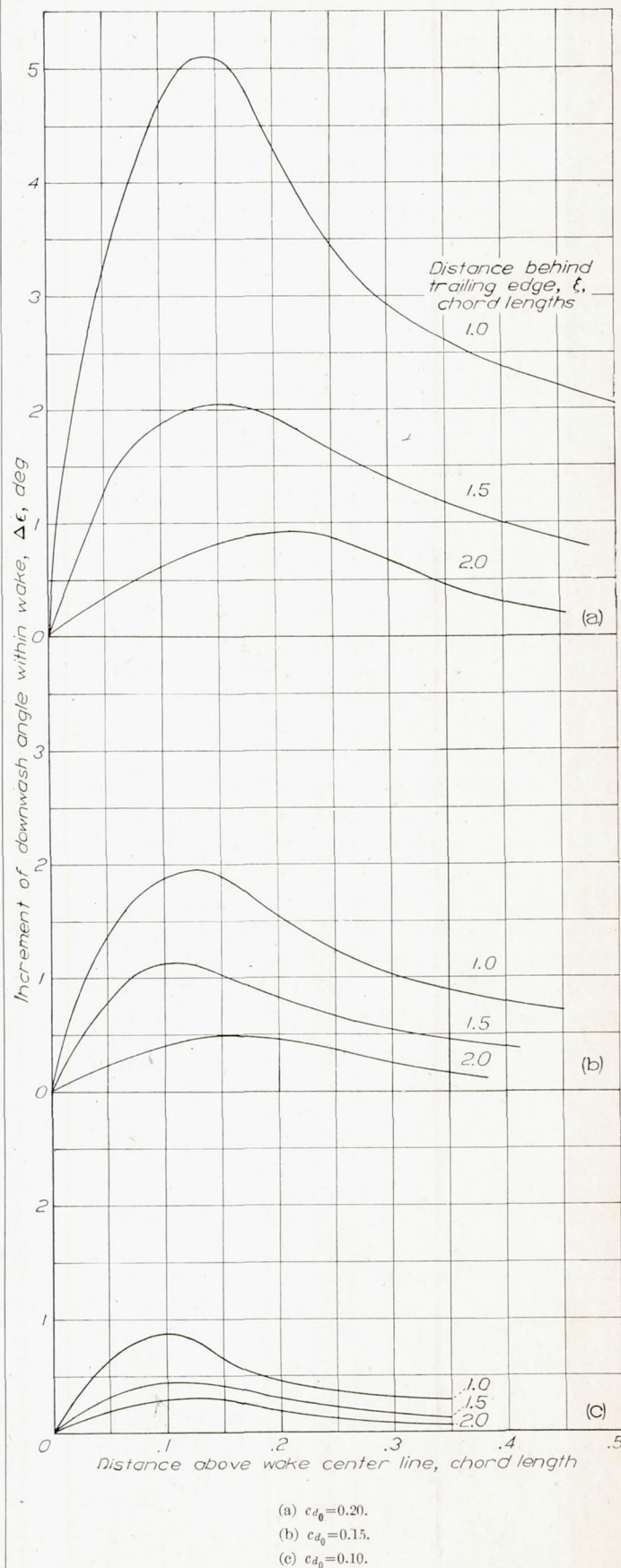
FIGURE 2.—Wake effect on downwash. The effects are equal but of opposite sign below the wake center.
