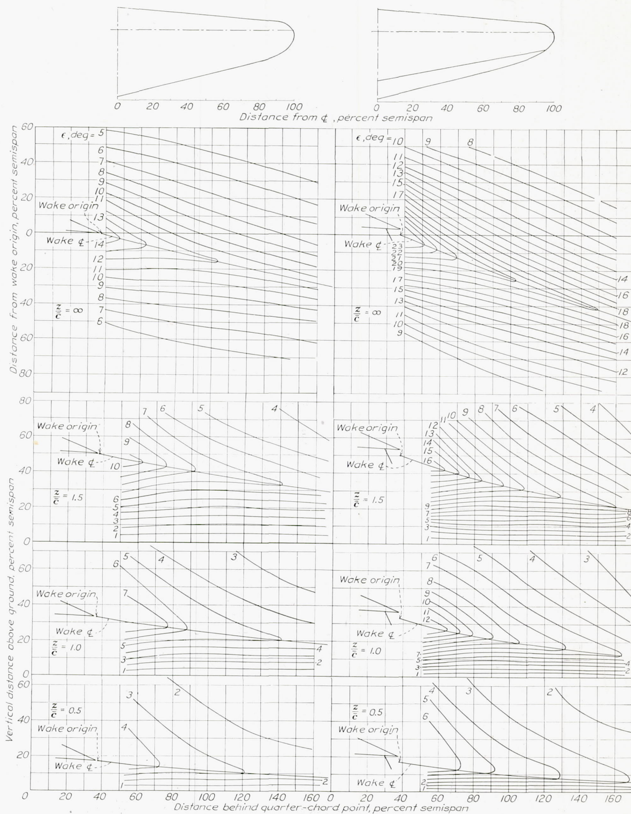
Plain wing; C_L , 1.5 Full-span flap; C_L , 2.5 FIGURE 7.—Theoretical downwash-angle contours and wake positions for various distances from ground. A , 6; taper ratio, 3:1.
