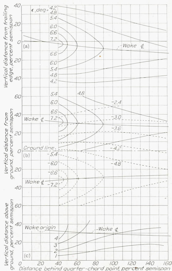
(a) Normal downwash field.
