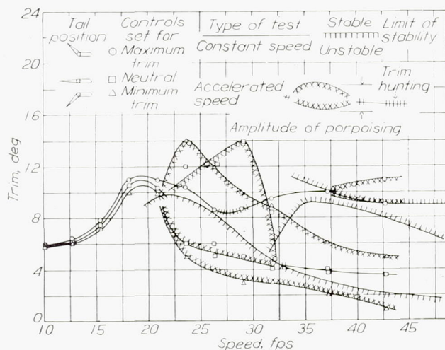
FIGURE 12.—Model 101BC. Stability characteristics obtained during accelerated and constant-speed runs. Load at rest, \Delta_s = 76.5 pounds; mass moving vertically, 76.5 pounds.
