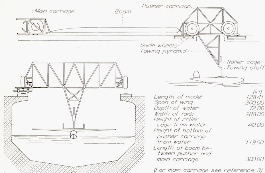
FIGURE 1.—General arrangement of pusher carriage for towing dynamic models.
