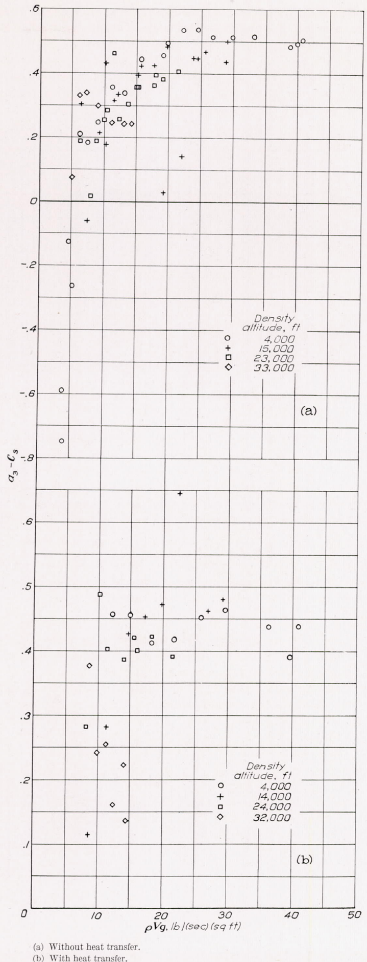
FIGURE 13.—Variation of exit coefficient with cooling-air weight flow.
