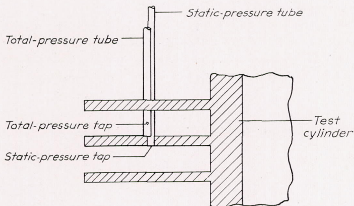
FIGURE 7.—Sketch showing method of installing pressure tubes between fins.
