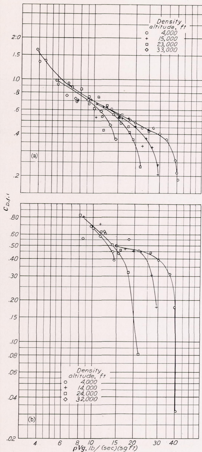
(a) Without heat transfer. (b) With heat transfer. FIGURE 16.—Effect of cooling-air weight flow on friction-drag coefficient calculated by use of assumed exit loss.
