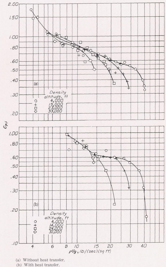
FIGURE 18.—Effect of cooling-air weight flow on pressure-loss coefficient calculated by use of assumed exit loss.
