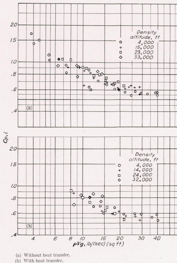
(a) Without heat transfer. (b) With heat transfer. FIGURE 17.—Effect of cooling-air weight flow on pressure-loss coefficient calculated from test data by analytical method.
