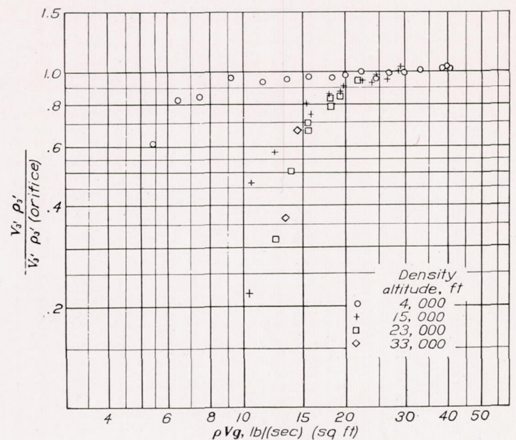
FIGURE 15.—Ratio of mass flow measured at station 3' to mass flow at station 3' obtained from orifice measurements. Tests made without heat transfer.
