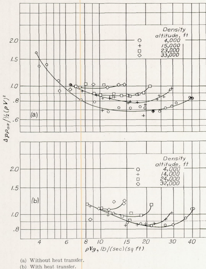
FIGURE 10.—Variation of pressure-loss function with cooling-air weight flow.
