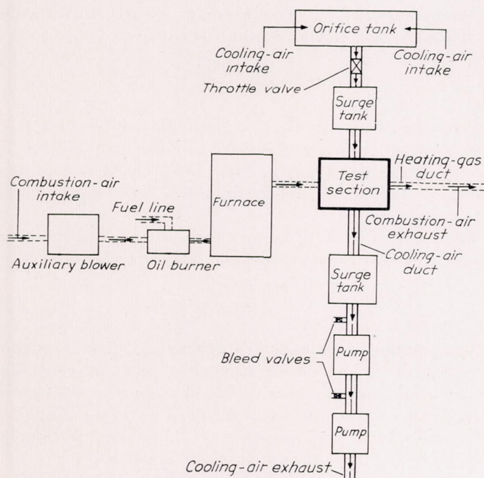
FIGURE 5.—Diagram of test setup.
