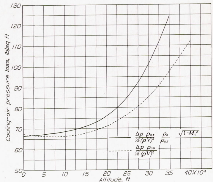
FIGURE 21.—Prediction of cooling-air pressure loss at altitude by use of \frac{\Delta p_{ex,t}}{\frac{1}{2}(\rho V)^2} \frac{\rho_0}{\rho_{0,t}} \sqrt{1-M_0^2} assumed a function of Reynolds number, and by use of \frac{\Delta p_{av}}{\frac{1}{2}(\rho V)^2} , assumed a function of mass flow.
