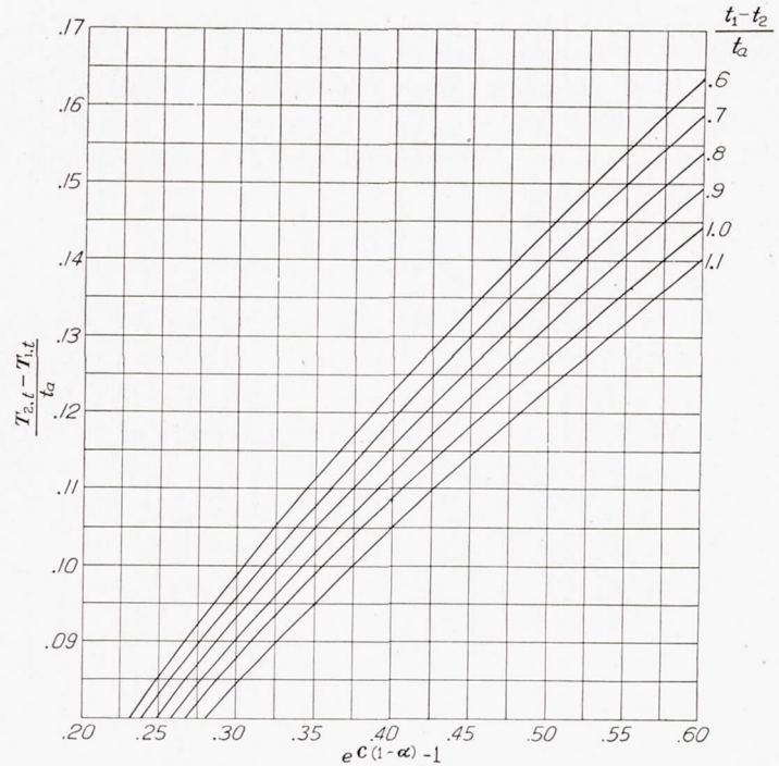
FIGURE 22.—Determination of \frac{T_{2,t} - T_{1,t}}{t_a} \alpha = \frac{5}{9} .
