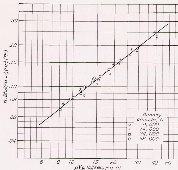
FIGURE 8.—Variation of surface heat-transfer coefficient with cooling-air weight flow.
