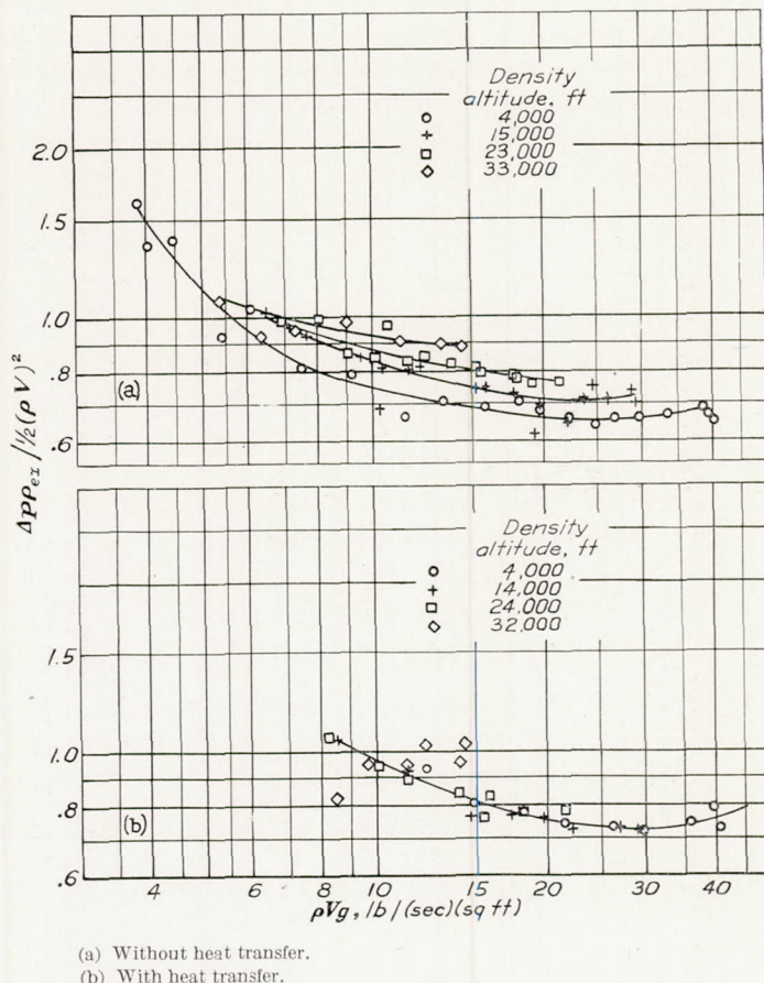
FIGURE 11.—Variation of pressure-loss function with cooling-air weight flow.
