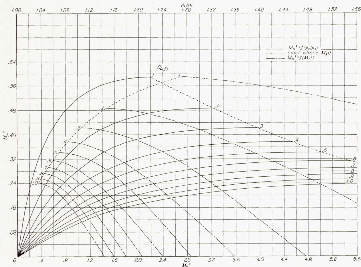
FIGURE 3.—Determination of ratio of density at station 2 to density at station 3. Parameters refer to values of C_{D,f,i} .
