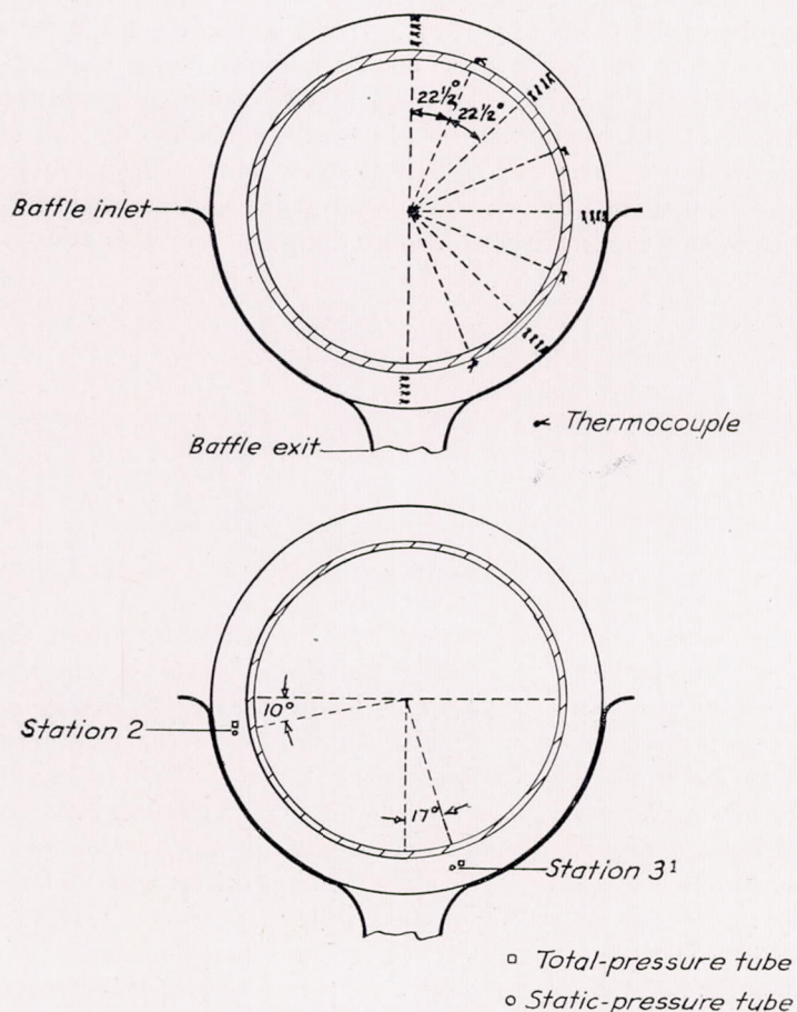
FIGURE 6.—Location of thermocouples and pressure tubes on test cylinder
