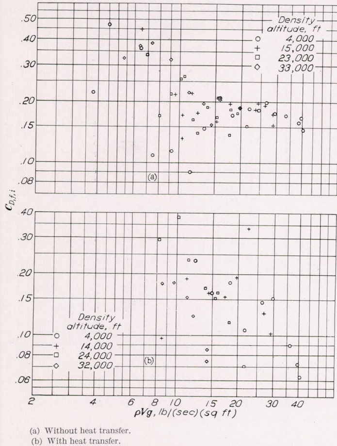
FIGURE 12.—Variation of baffle-channel drag coefficient with cooling-air weight flow. Drag coefficient calculated from test data.
