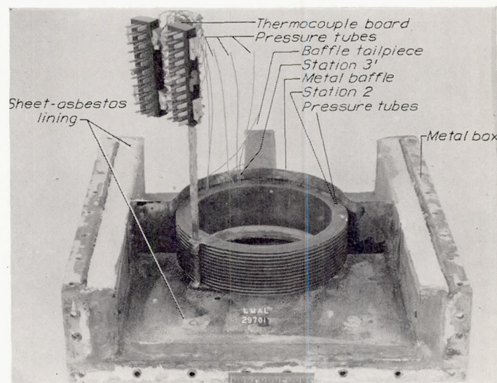
FIGURE 4.—Test unit showing test cylinder, baffles, tailpiece, insulated metal box, pressure tubes, and thermocouples.
