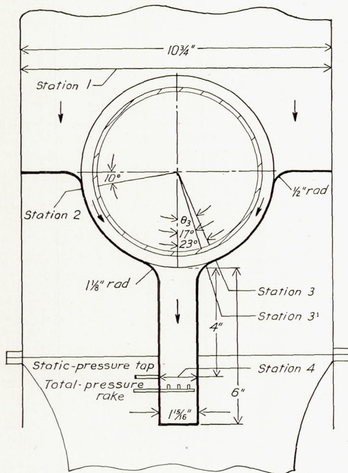
FIGURE 1.—Finned cylinder, baffles, tailpiece, and measuring-station locations used in tests.
