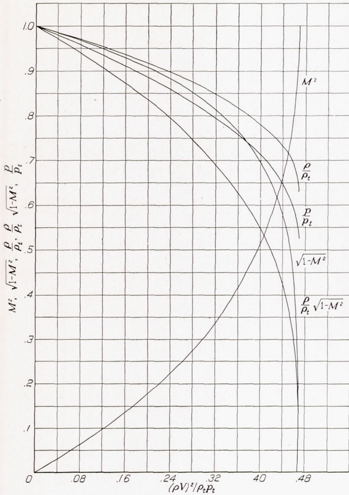
FIGURE 2.—Relation between stagnation state and static state of air as determined by mass flow.
