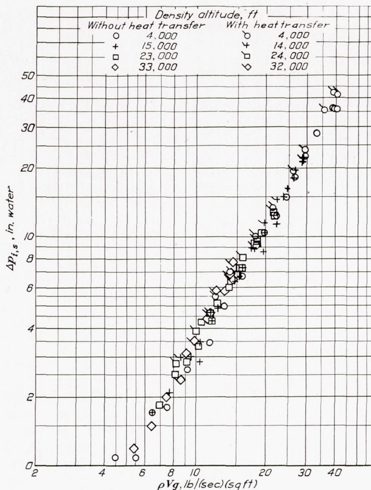
FIGURE 20.—Variation of corrected pressure loss with cooling-air weight flow.
