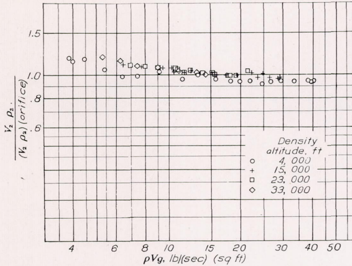
FIGURE 14.—Ratio of mass flow measured at station 2 to mass flow at station 2 obtained from orifice measurements. Tests made without heat transfer.
