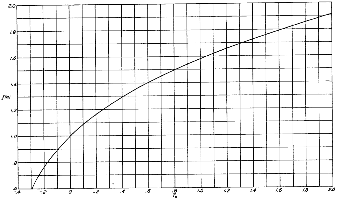
FIGURE 1.—Variation of q -factor f(a) with T_c . T_c = \frac{C_T}{(\sqrt{n}D)^2} .
