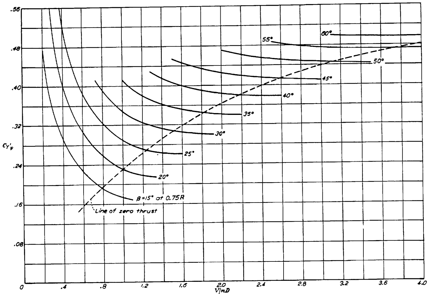
FIGURE 8.—Side-force derivative for single-rotating Hamilton Standard propeller 3155-6 with spinner. Six blades; \sigma = 0.182 .
