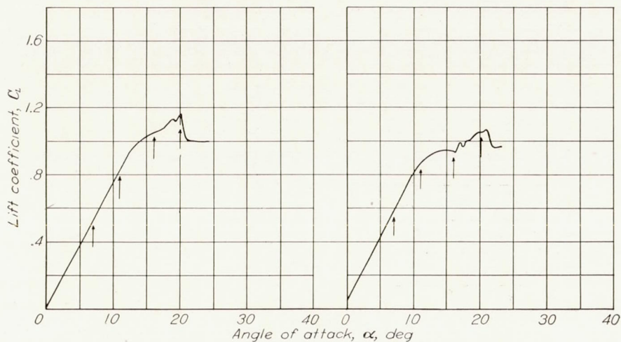
FIGURE 37.—Effect of wing-duct-outlet location on the stalling characteristics of airplane 16. Propeller removed; \delta_f = 0^\circ ; approximate test velocity, 60 miles per hour.
