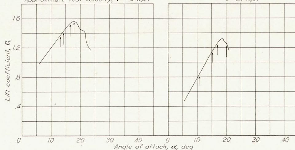
FIGURE 39.—Effect of airspeed-head location on stalling characteristics. Propellers removed.
