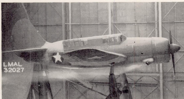
(g) Airplane 7 in service condition.
