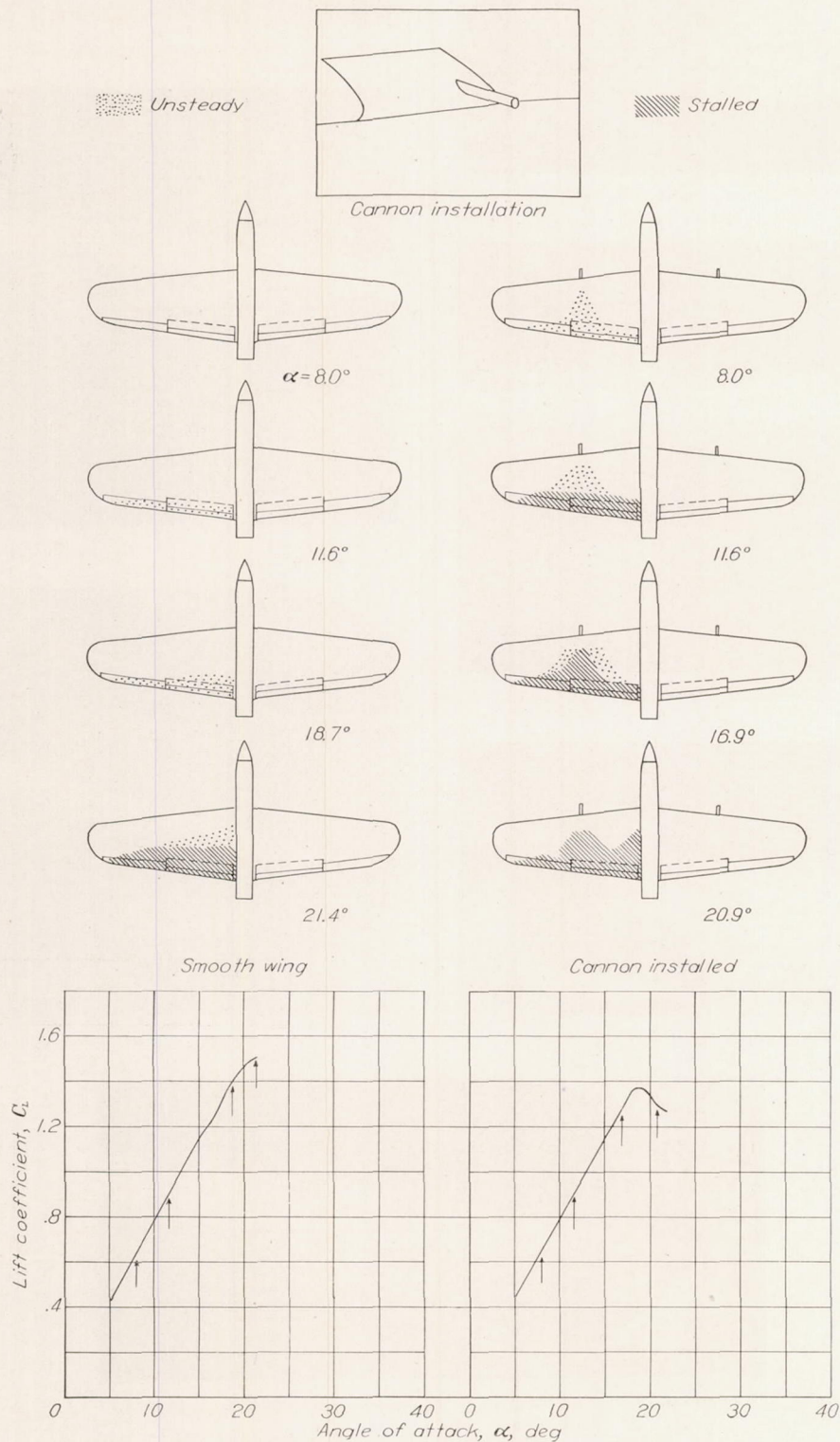
FIGURE 26.—Effect on stall and maximum lift of installing a 37-millimeter-cannon mock-up on the leading edge of the wing of airplane 4. \delta_f=0^\circ ; approximate test velocity, 60 miles per hour. Tufts on left wing only.
