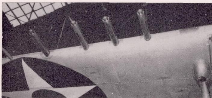
FIGURE 22.—Ten-inch barrel extension in low position on right wing. Airplane 11.
