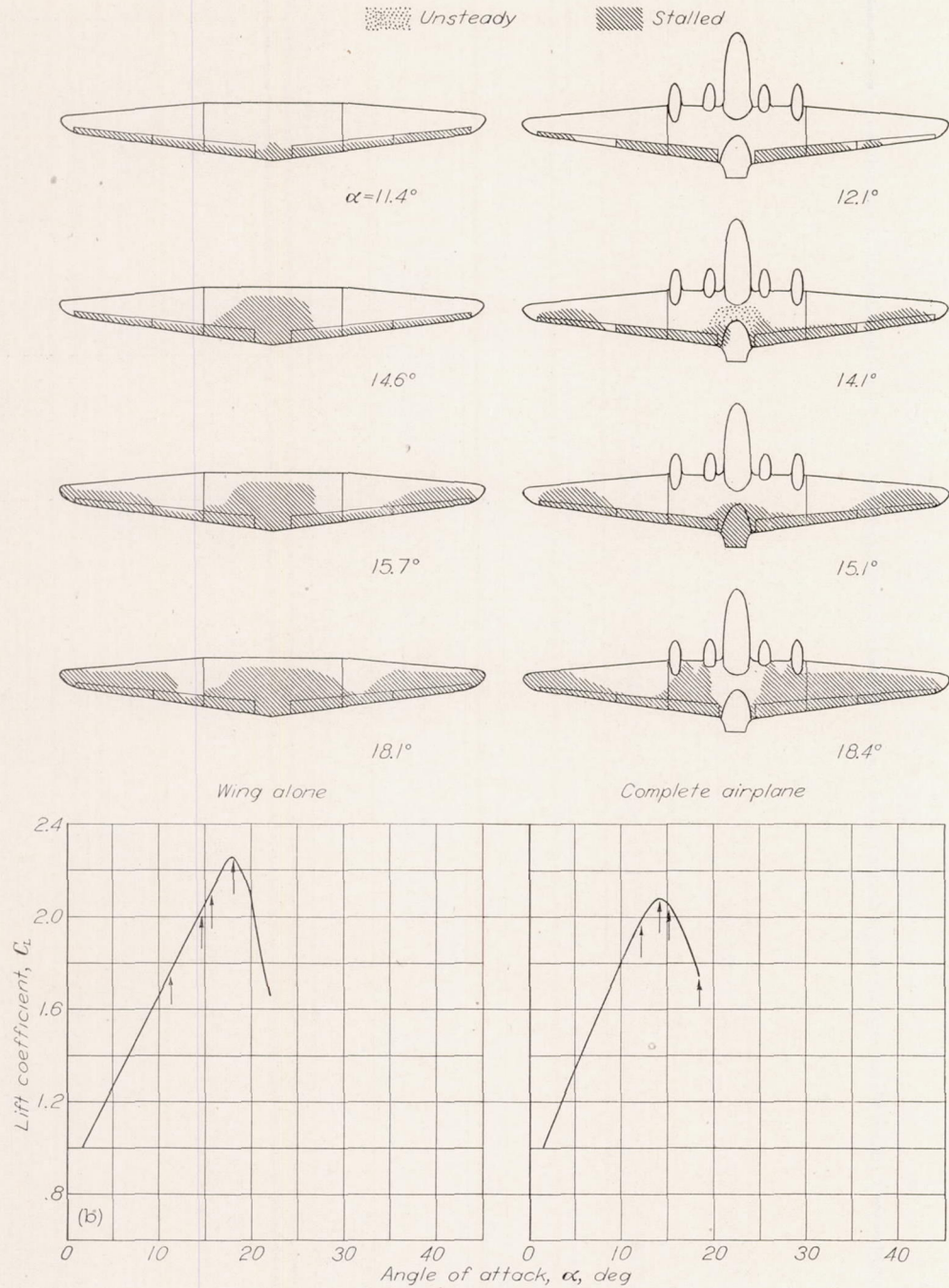
(b) Flaps deflected 55°. FIGURE 7.—Concluded.
