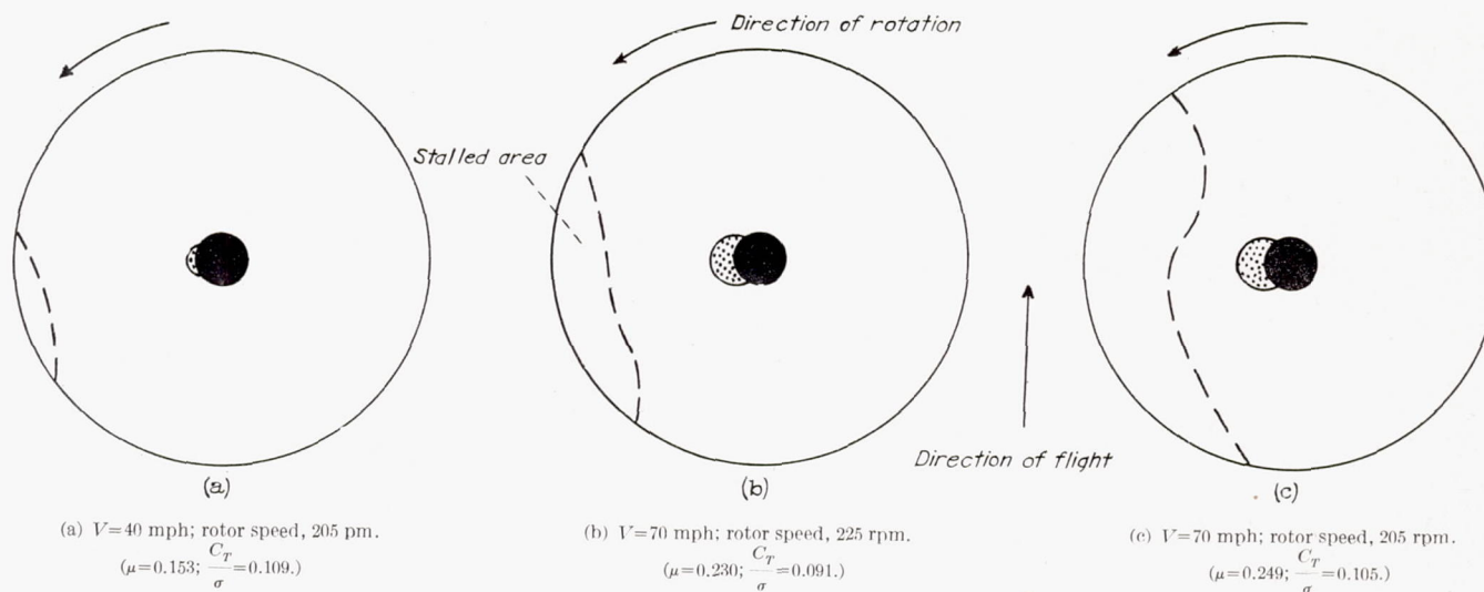
FIGURE 1.—Theoretical stall boundaries for representative helicopter conditions. Weight 2580 pounds; radius, 19 feet; parasite-drag area, 23 square feet; stalling angle of attack, 12^\circ .
