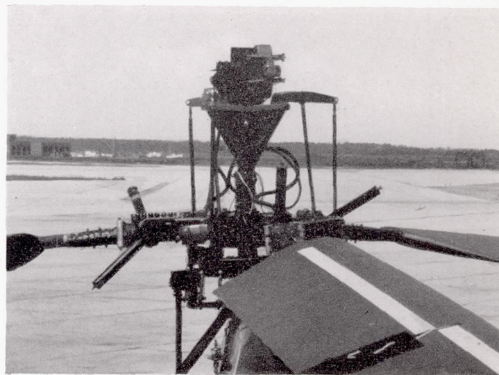
FIGURE 2.—Camera installation on helicopter rotor hub.
