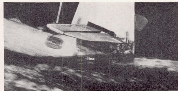
FIGURE 23.—Flow of water around afterbody and tail extension. Model 180-2; gross load, 94.3 pounds (165,000 lb, full size); \delta_a=0^\circ ; \delta_T=30^\circ ; center of gravity, 28 percent mean aerodynamic chord.
