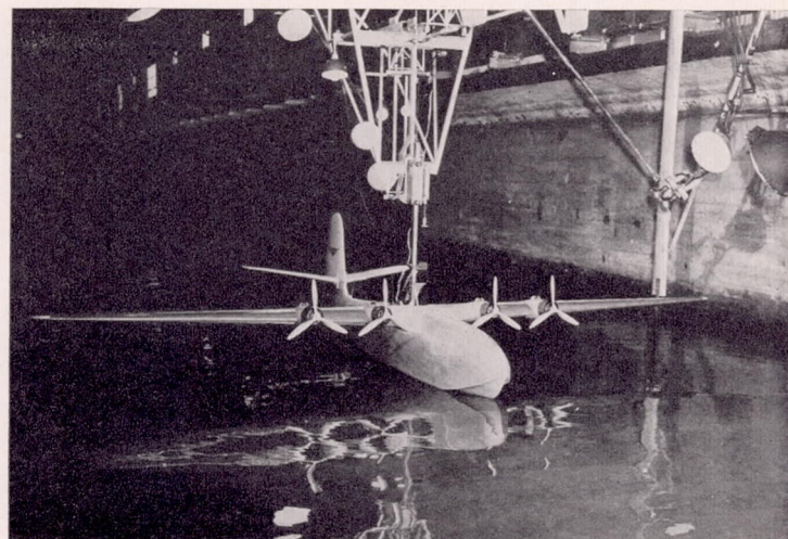
FIGURE 5.—Model 180 and towing apparatus.
