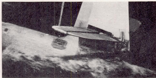
FIGURE 22.—Modifications on tail extension for spray control.
