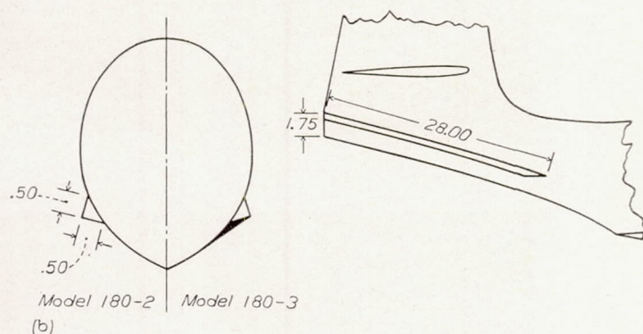
(b) Sketch of breaker strip. Langley tank models 180-2 and 180-3. (All dimensions are in inches.)
