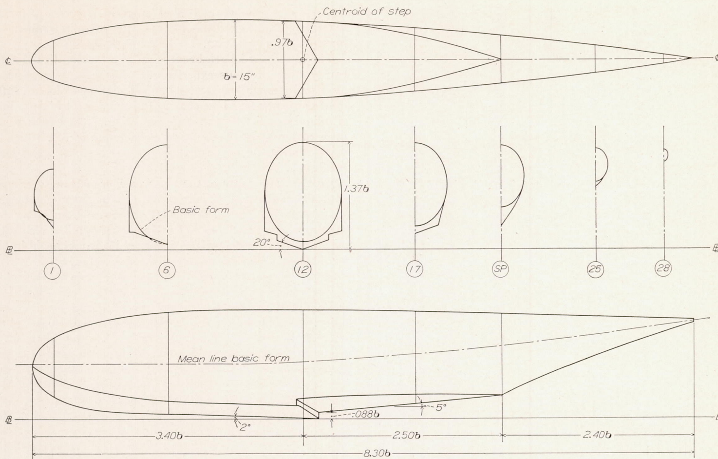
FIGURE 3.—Lines of hull. Model 180.
