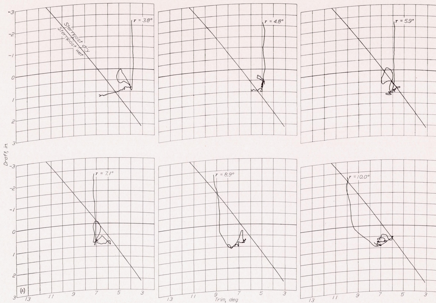
FIGURE 10.—Variation of trim and draft during landing. Model 180-1; gross load 94.3 pounds (165,000 lb, full size); without power; \delta_f = 55^\circ .
