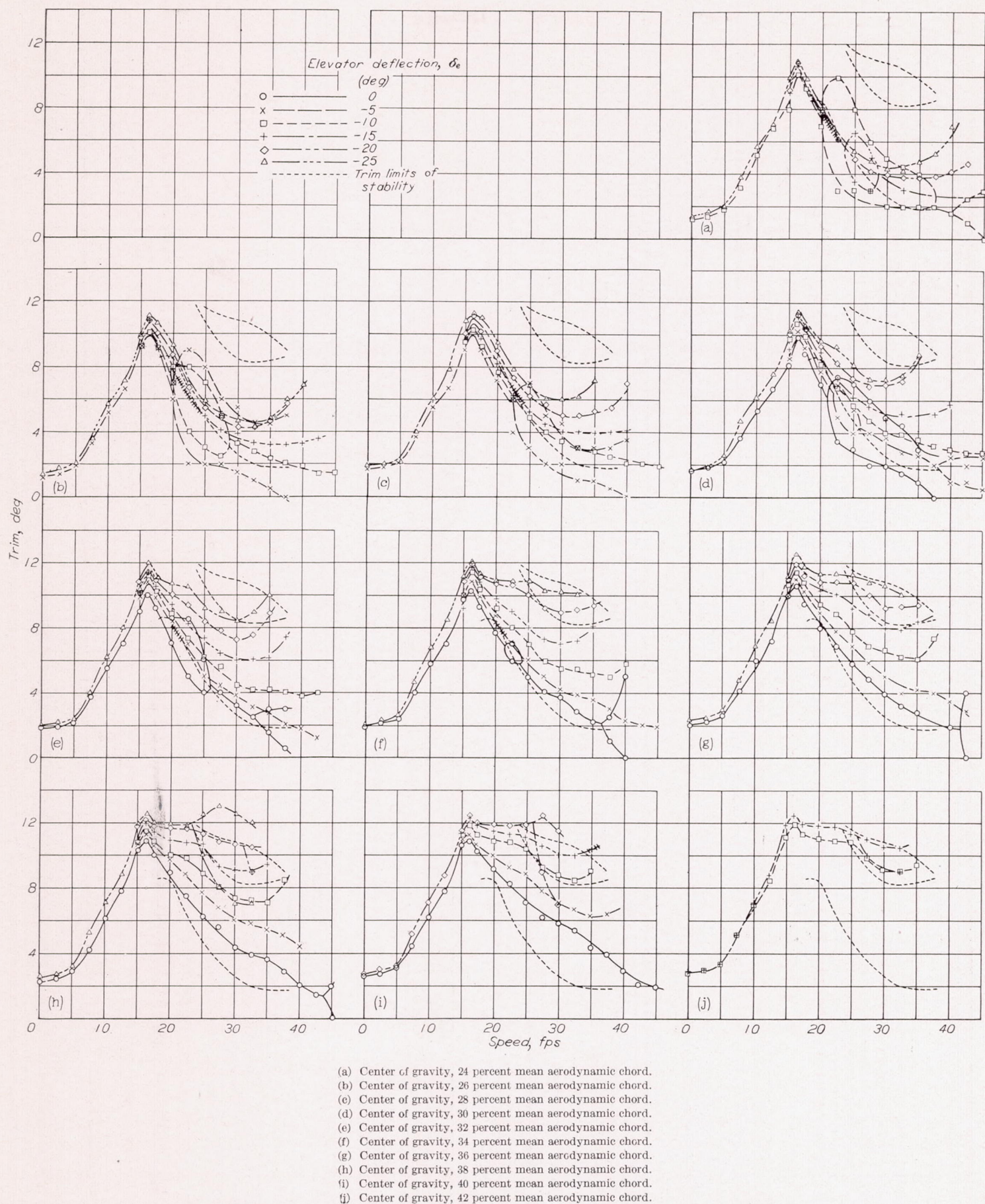
FIGURE 15.—Variation of trim with speed. Model 180-1; gross load, 105.7 pounds (185,000 lb, full size); \delta_f=30^\circ ; full power.
