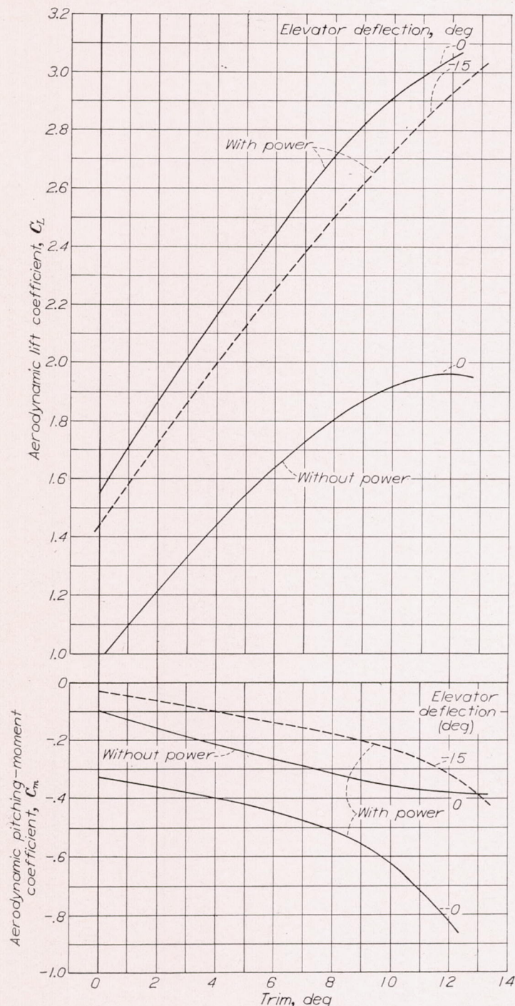
FIGURE 8.—Variation of aerodynamic lift and pitching-moment coefficients with trim. Model 180; \delta_f=30^\circ ; center of gravity, 24 percent mean aerodynamic chord; V=35 feet per second.
