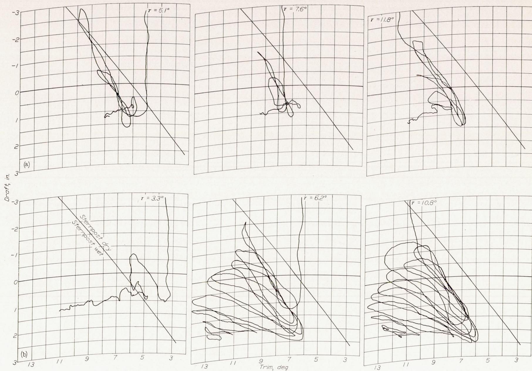
FIGURE 9.—Variation of trim and draft during landing. Model 180; gross load, 94.3 pounds (165,000 lb, full size); without power; \delta_f = 55^\circ .
