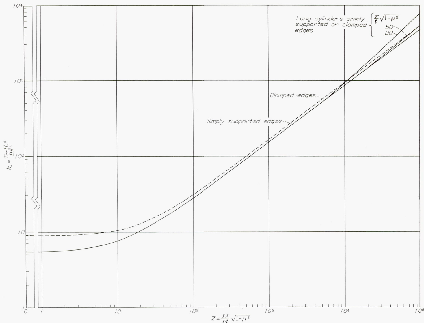
FIGURE 7.—Critical-shear-stress coefficients for cylinders in torsion. (Fig. 1 of reference 14.)
