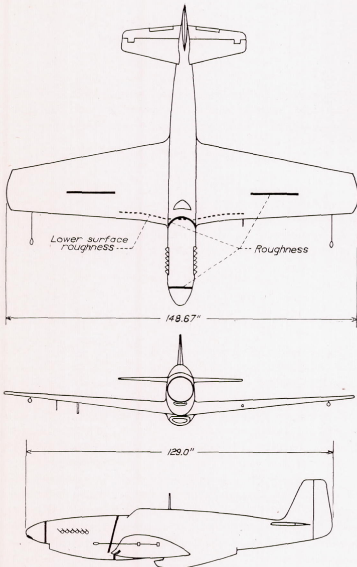
FIGURE 16.—Three-view drawing of the \frac{1}{3} -scale model of the test airplane.
