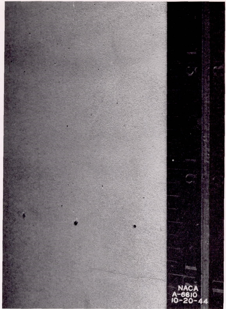
FIGURE 17.—Surface roughness on wing leading edge of the \frac{1}{3} -scale model of the test airplane.
