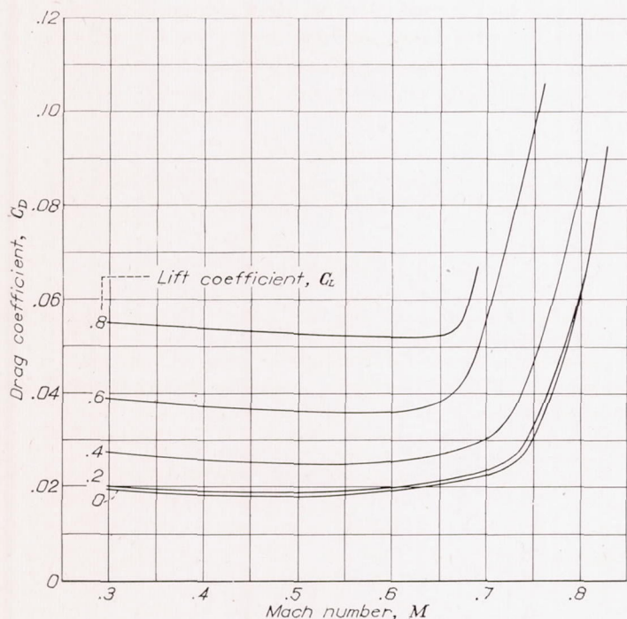
FIGURE 21.—Variation of drag coefficient with Mach number at several values of lift coefficient for the \frac{1}{3} -scale model of the test airplane
