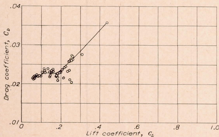
FIGURE 12.—Variation of drag coefficient with lift coefficient below 0.64 Mach number during a dive from 25,000 feet, propeller off, most dust on airplane, flight 108.
