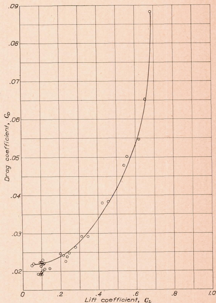
FIGURE 14.—Variation of drag coefficient with lift coefficient below 0.64 Mach number during a dive from 28,000 feet, propeller off, medium dustiness, flight 110.
