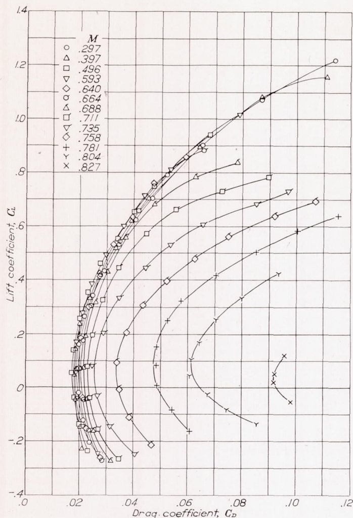
FIGURE 20.—Variation of drag coefficient with lift coefficient at several Mach numbers for the \frac{1}{3} -scale model of the test airplane.
