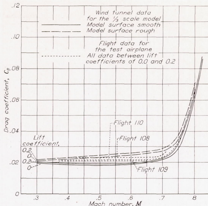
FIGURE 22.—Comparison of drag coefficients of the \frac{1}{3} -scale model with smooth and rough wing surfaces with the drag coefficients of the test airplane.
