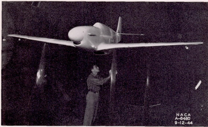
FIGURE 15.—The \frac{1}{3} -scale model of the test airplane mounted in the Ames 16-foot high-speed wind tunnel.
