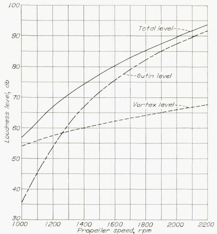
FIGURE 3.—Theoretical loudness level, five-blade propeller. Diameter, 8 feet; speed, 130 miles per hour; horsepower, 185; distance, 300 feet. Interpolated from data of reference 8.
