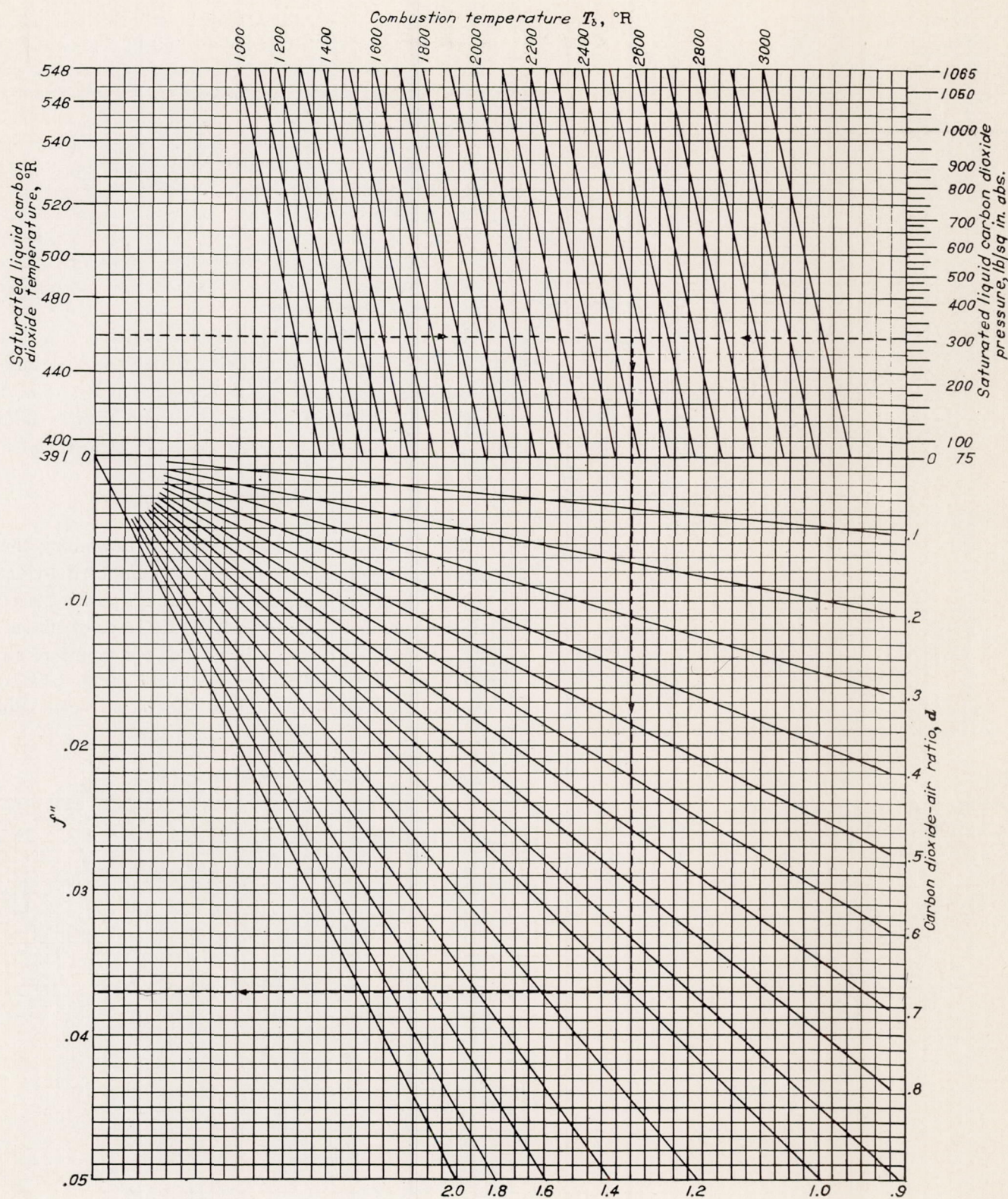
FIGURE 11.—Fuel-air-ratio increment \Delta f for addition of saturated liquid carbon dioxide to fuel-air mixture. \Delta f = K_m K_h f'' .
