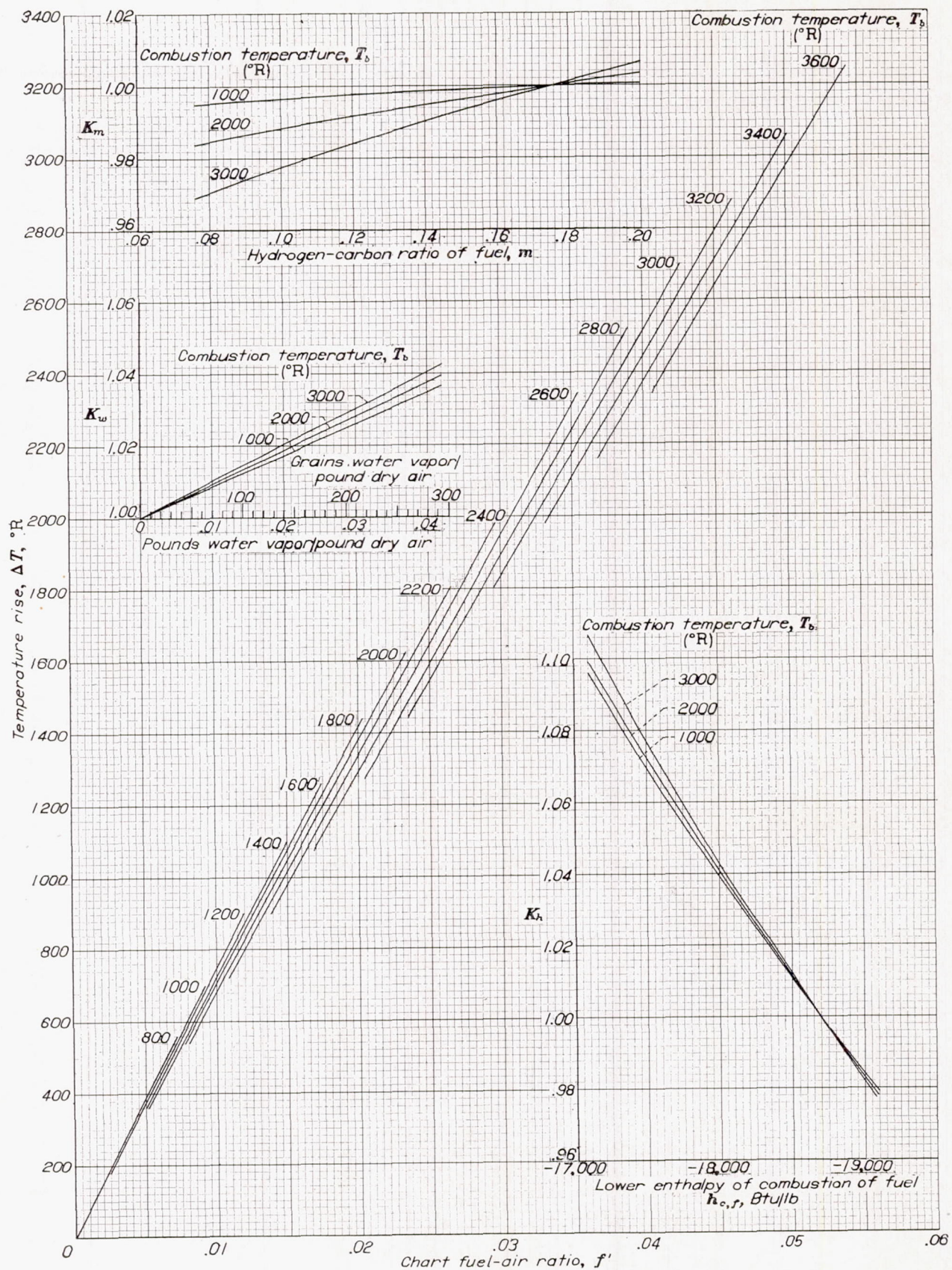
FIGURE 2.—Fuel-air ratio f for ideal constant-pressure combustion as function of combustion temperature. f = K_m K_h K_w f' .
