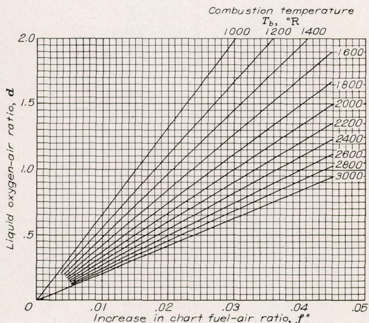
FIGURE 13.—Fuel-air-ratio increment \Delta f for addition of liquid oxygen to fuel-air mixture. \Delta f = K_m K_h f'' .
