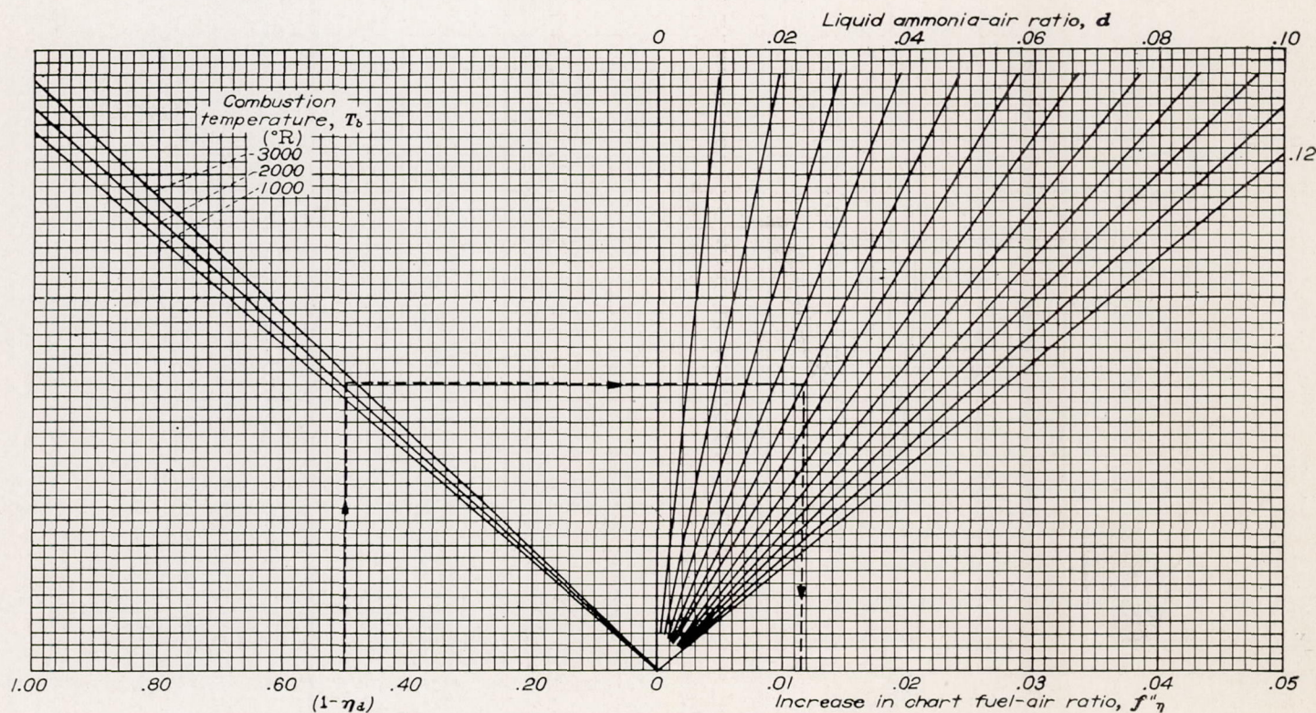
FIGURE 10.—Fuel-air-ratio increment \Delta f due to incomplete combustion of ammonia. \Delta f = K_m K_h f'' \eta .
