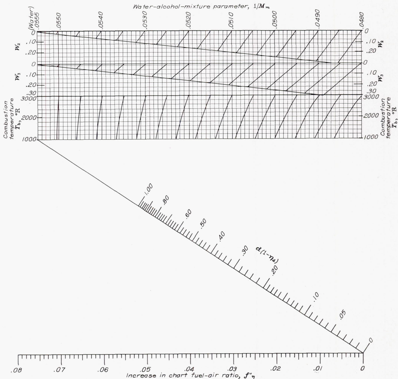
FIGURE 8.—Fuel-air-ratio increment \Delta f due to incomplete combustion of water-alcohol mixtures containing 75-percent water by weight or more. \Delta f = K_m K_h f'' \eta .
