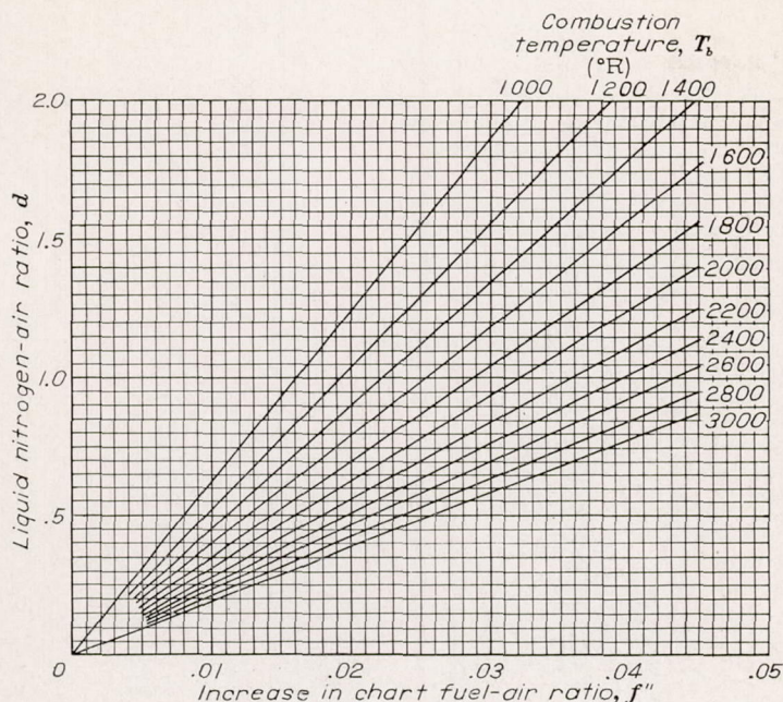
FIGURE 12.—Fuel-air-ratio increment \Delta f for addition of liquid nitrogen to fuel-air mixture. \Delta f = K_m K_h f'' .
