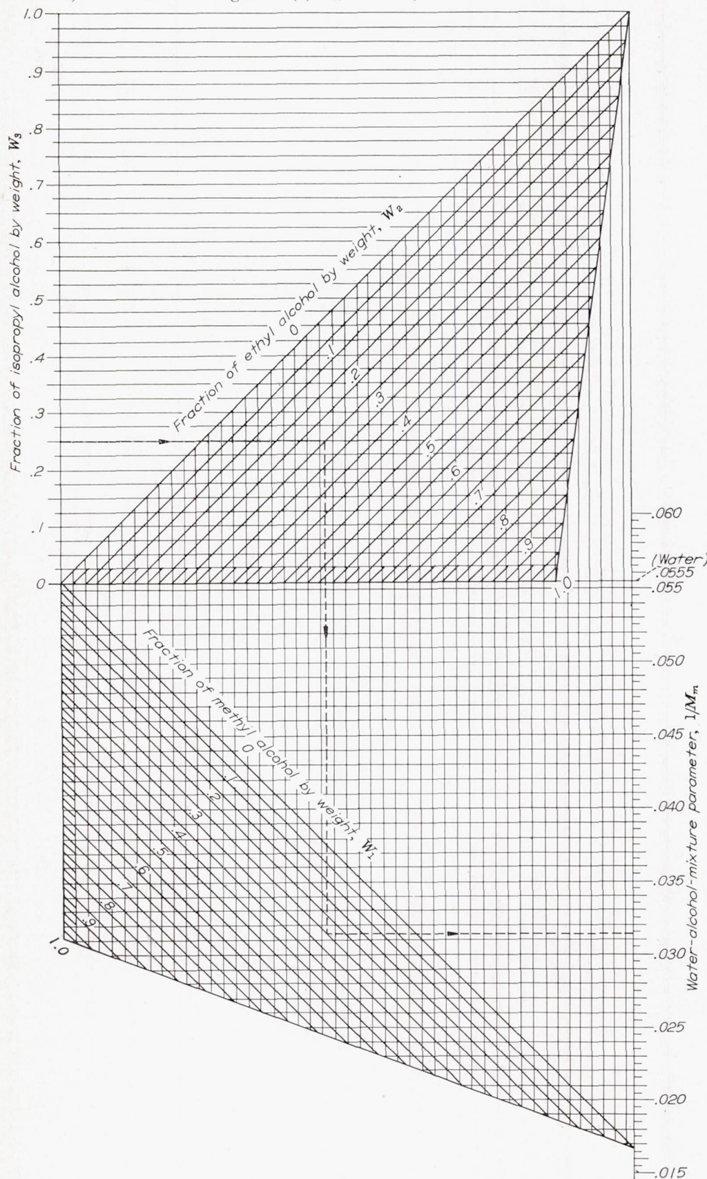
FIGURE 4.—Water-alcohol-mixture parameter as function of mixture composition by weight.
