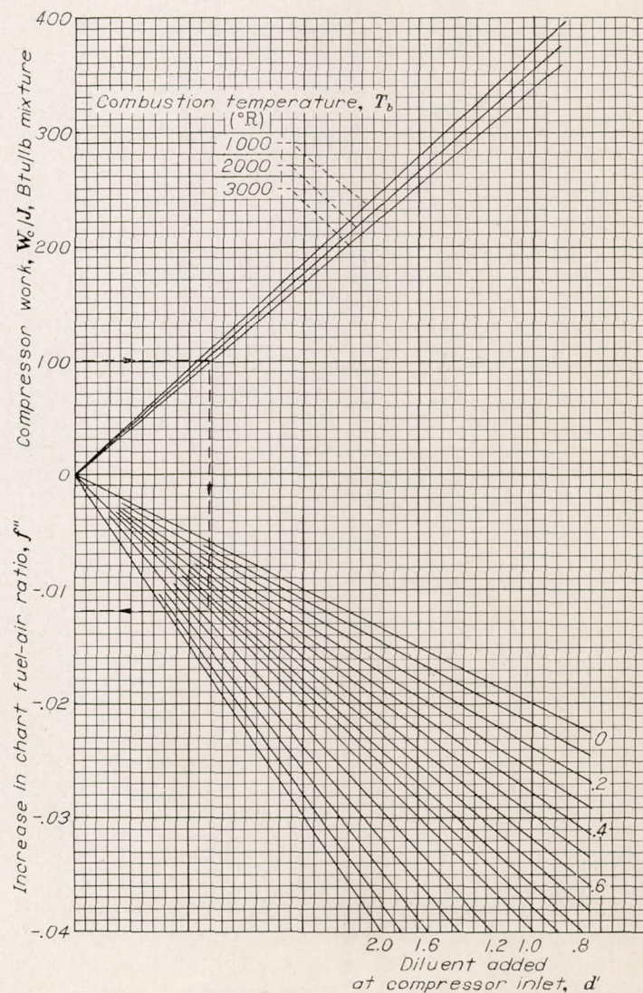
FIGURE 14.—Fuel-air-ratio increment \Delta f for work addition by compressor to diluent-air mixture. \Delta f = K_m K_h f'' .
