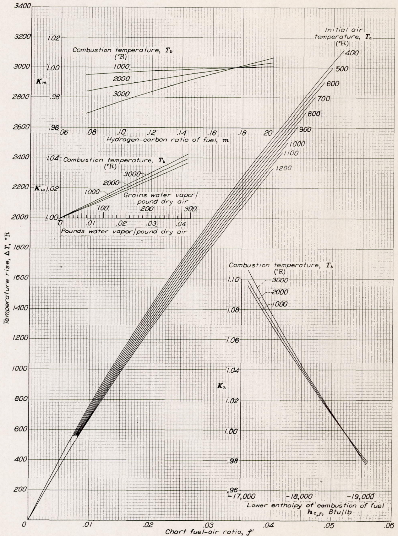
FIGURE 1.—Fuel-air ratio f for ideal constant-pressure combustion as function of initial temperature. f = K_m K_h K_w f' .
