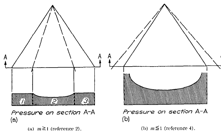
FIGURE 3.—Pressure distributions due to angle of attack.
