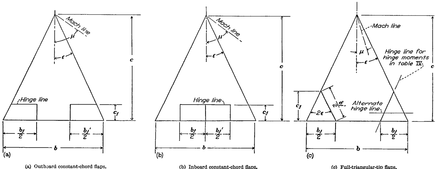
FIGURE 1.—The control-surface configurations investigated.
