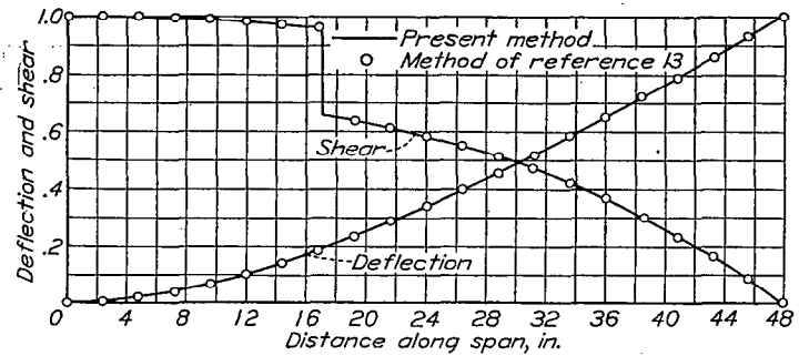
FIGURE 6.—Plots of deflection and shear curves computed from the first uncoupled modes in bending by the differential-equation method and by the 20-station iteration process of reference 13 (referred to unit tip deflection).
