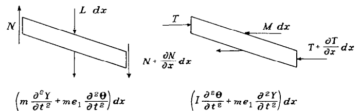
SKETCH 2.
