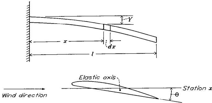
SKETCH 1.
