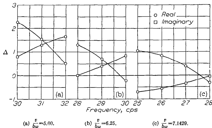
FIGURE 7.—Plots of \Delta against frequency for particular values of reduced speed. l_1 = 17 inches.
