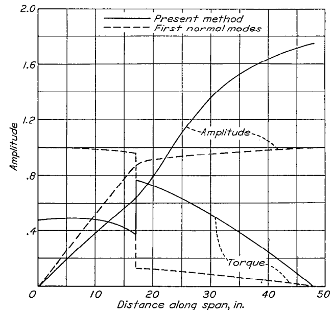
FIGURE 5.—Plots of amplitudes in torsional displacement and torque and the corresponding curves computed for the first uncoupled normal mode in torsion for l_1=17 inches (amplitude and torque referred to unit amplitude at tip in bending).
