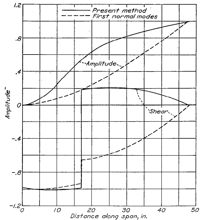
FIGURE 4.—Plots of amplitudes in bending displacement and torque and the corresponding curves computed for the first uncoupled normal mode in bending for l_1=17 inches (amplitude and shear referred to unit amplitude at the tip in bending).
