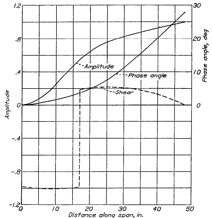
FIGURE 2.—Plot of amplitude and phase angle of displacement and shear curve in bending at flutter for l_1 = 17 inches (amplitude and shear referred to unit amplitude at tip in bending).
