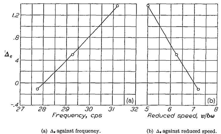
FIGURE 8.—Plots of \Delta_e against frequency and reduced speed. l_1 = 17 inches.
