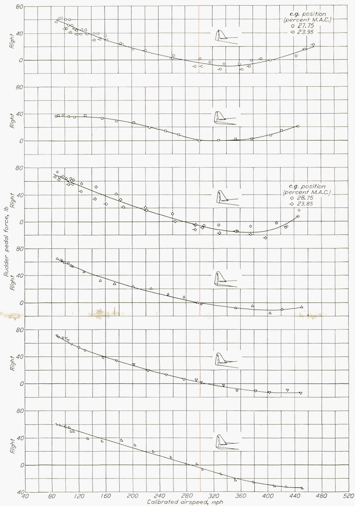
FIGURE 17.—Effect of vertical-tail modifications on the variation of rudder force with speed for constant trim tab setting. Normal rated power (2,600 rpm, 43 in. Hg); altitude, 5,000 feet.
