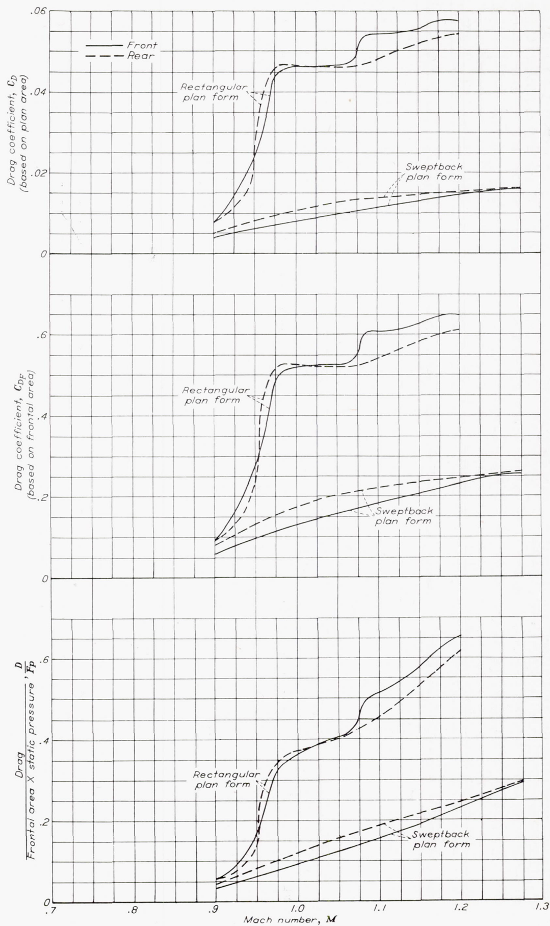
FIGURE 5.—Variation with Mach number of airfoil drag coefficients and D/Fp for airfoils of conventional rectangular plan form and sweptback plan form.
