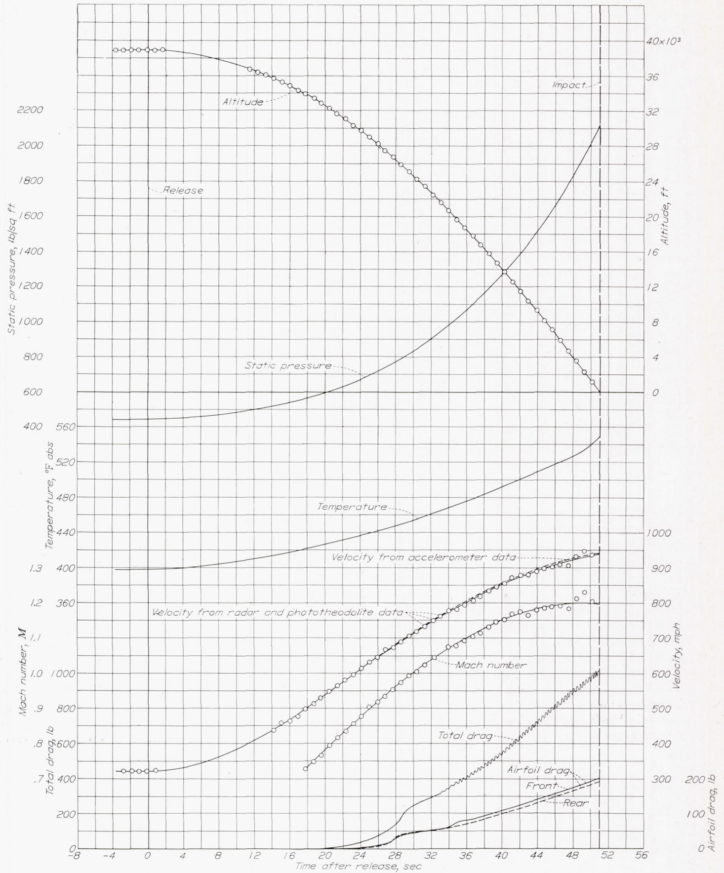
FIGURE 3.—Time history of free fall of 1,235-pound test body equipped with airfoils of conventional rectangular plan form (NACA 65-009 section).
