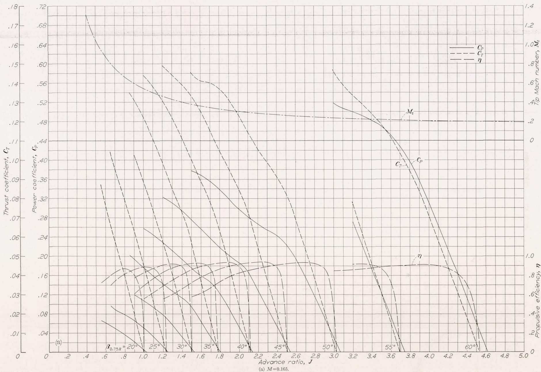
FIGURE 9.—Characteristics for the NACA 4-(3)(08)-045 propeller.
