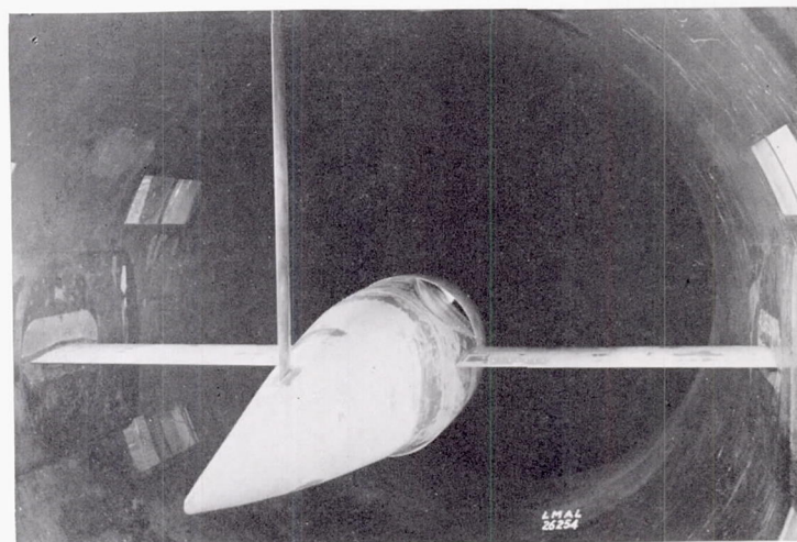
(a) Wing-fuselage model.
