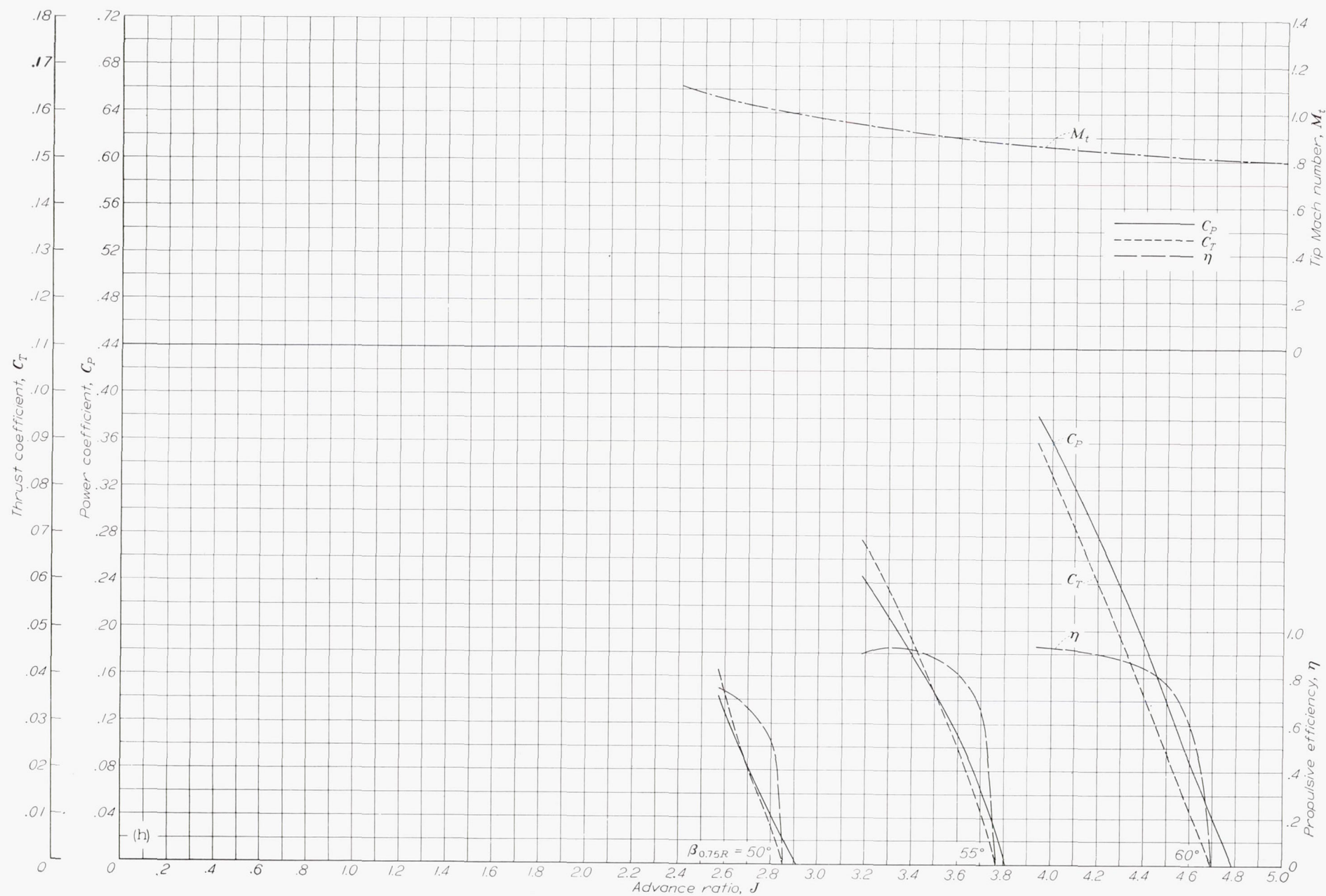
(h) M=0.675 . FIGURE 9.—Continued.
