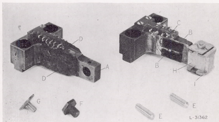
FIGURE 5.—Dynamometer details.
