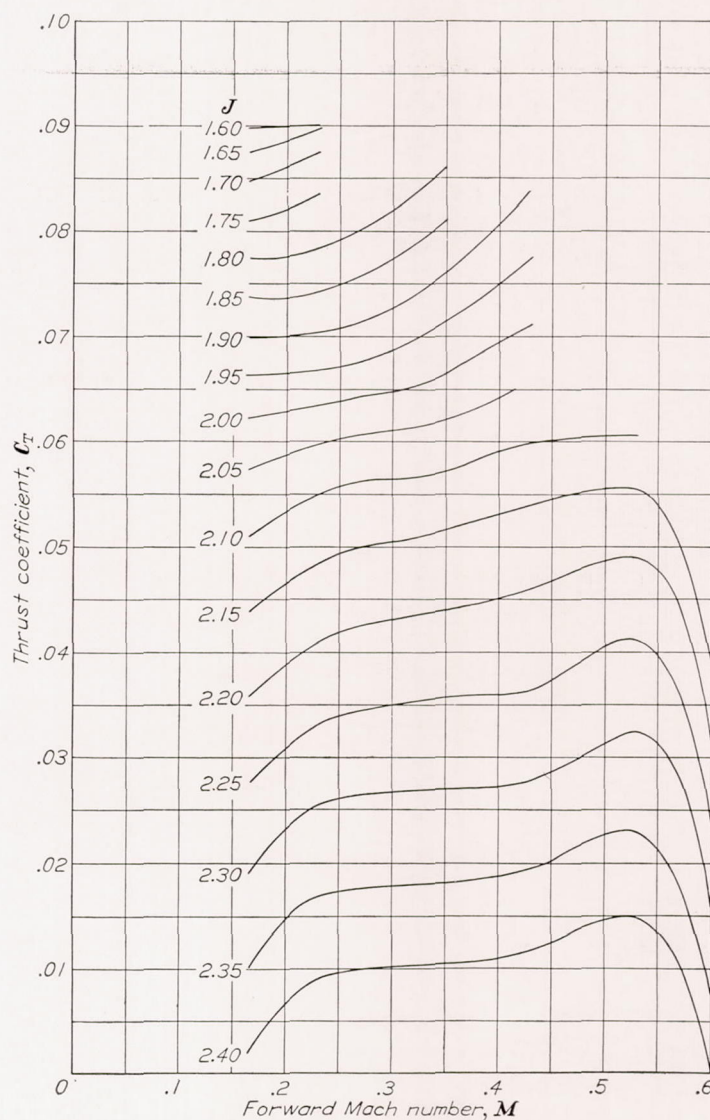
FIGURE 14.—Variation of thrust coefficient with Mach number for constant values of advance ratio for the NACA 4-(3)(08)-03 propeller. \beta_{0.75R}, 45^\circ .
