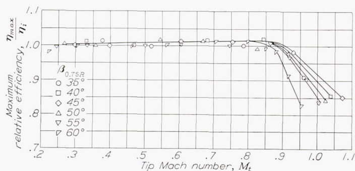
FIGURE 10.—Effect of compressibility on relative maximum efficiency for NACA 4-(3)(08)-03 propeller.
