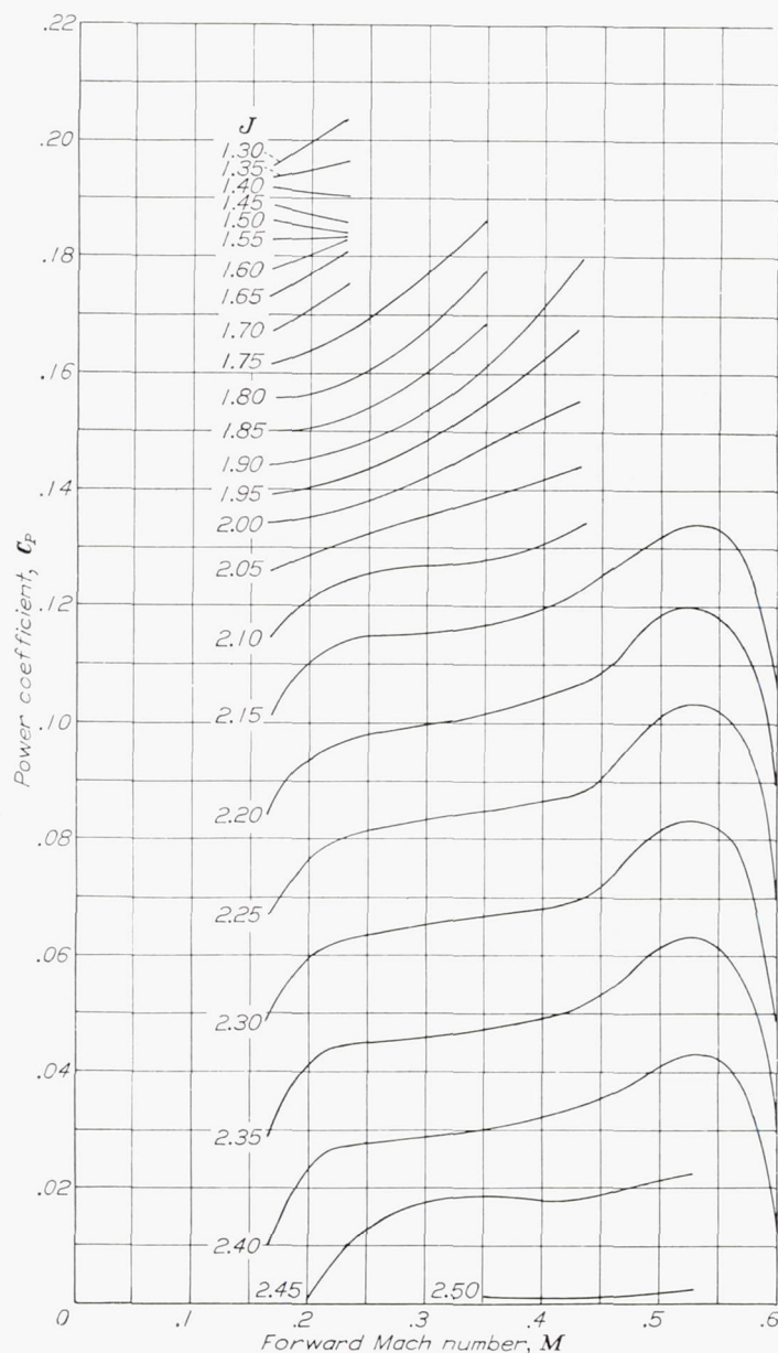
FIGURE 15.—Variation of power coefficient with Mach number for constant values of advance ratio for the NACA 4-(3)(08)-03 propeller. \beta_{0.75R} , 45^\circ .
