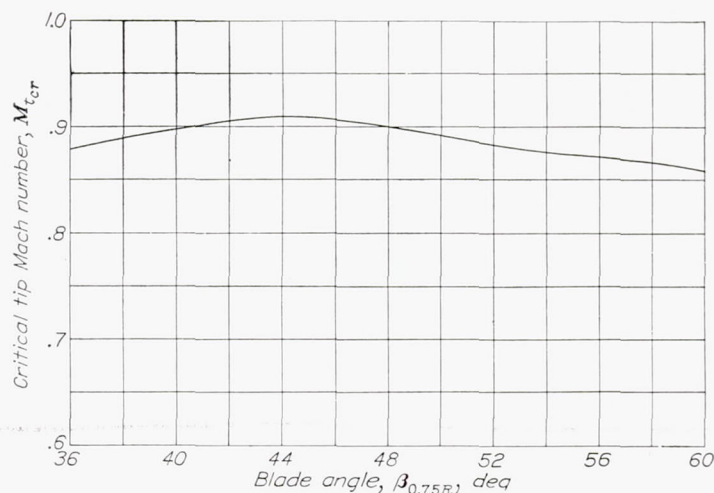
FIGURE 11.—Effect of blade angle on critical tip Mach number for NACA 4-(3)(08)-03 propeller.
