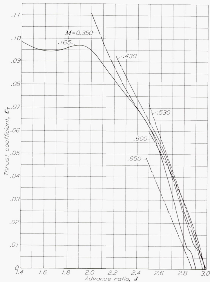
FIGURE 16.—Effects of compressibility on thrust coefficient for the NACA 4-(3)(08)-03 propeller. \beta_{0.75R} , 50^\circ .
