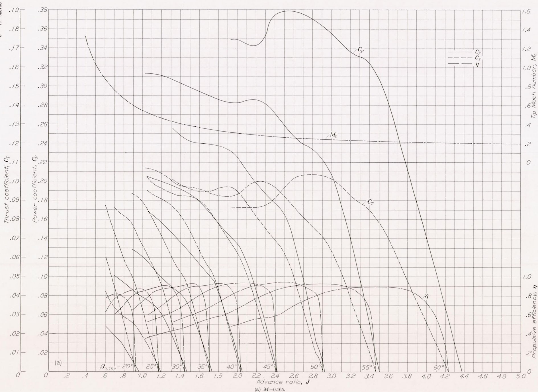
FIGURE 8.—Characteristics for the NACA 4-(3)(08)-03 propeller.
