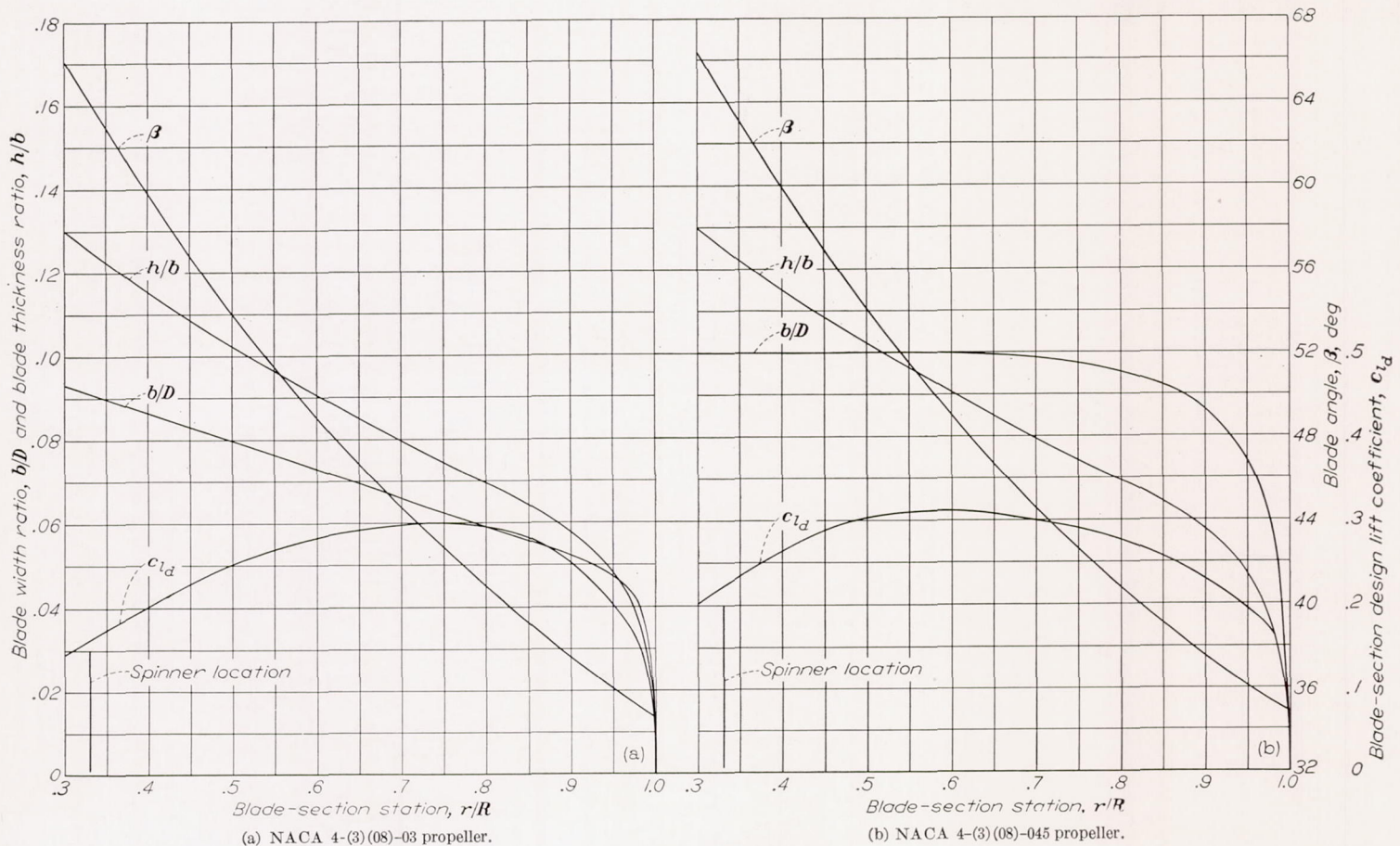
FIGURE 2.—Blade-form curves.
