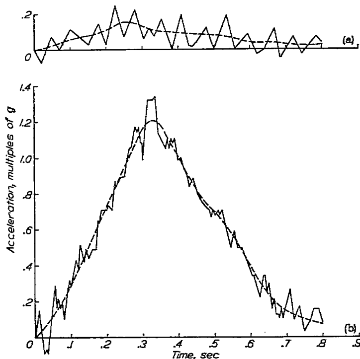
(a) Acceleration parallel to seaplane keel line during impact. (b) Acceleration normal to seaplane keel line during impact.
