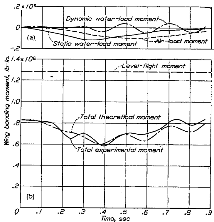
FIGURE 5.—Wing-bending-moment time histories during impact; run 2.
