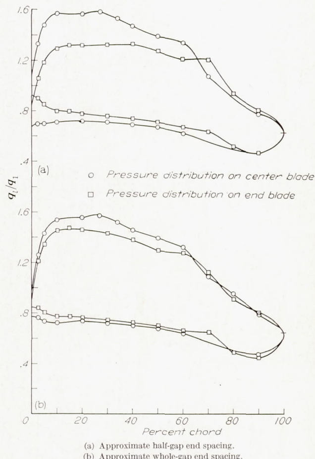
FIGURE 8.—Effect of end gap on the pressure distribution measured on the end blade.
