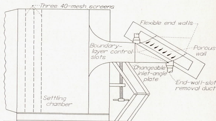
FIGURE 1.—Vertical cross section of two-dimensional low-speed cascade tunnels.
