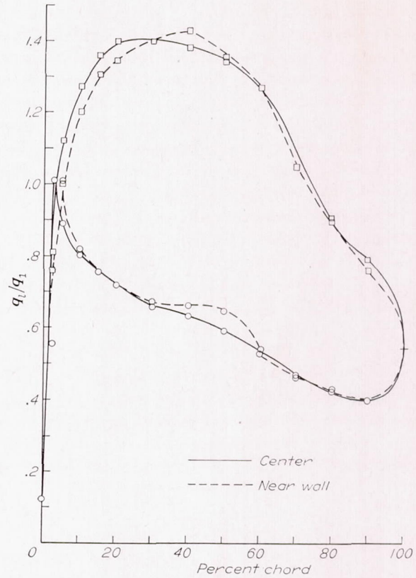
FIGURE 20.—Comparison of pressure distributions at two spanwise locations in the porous-wall cascade of aspect ratio 4, at 60^\circ inlet angle, and with a solidity of 1.
