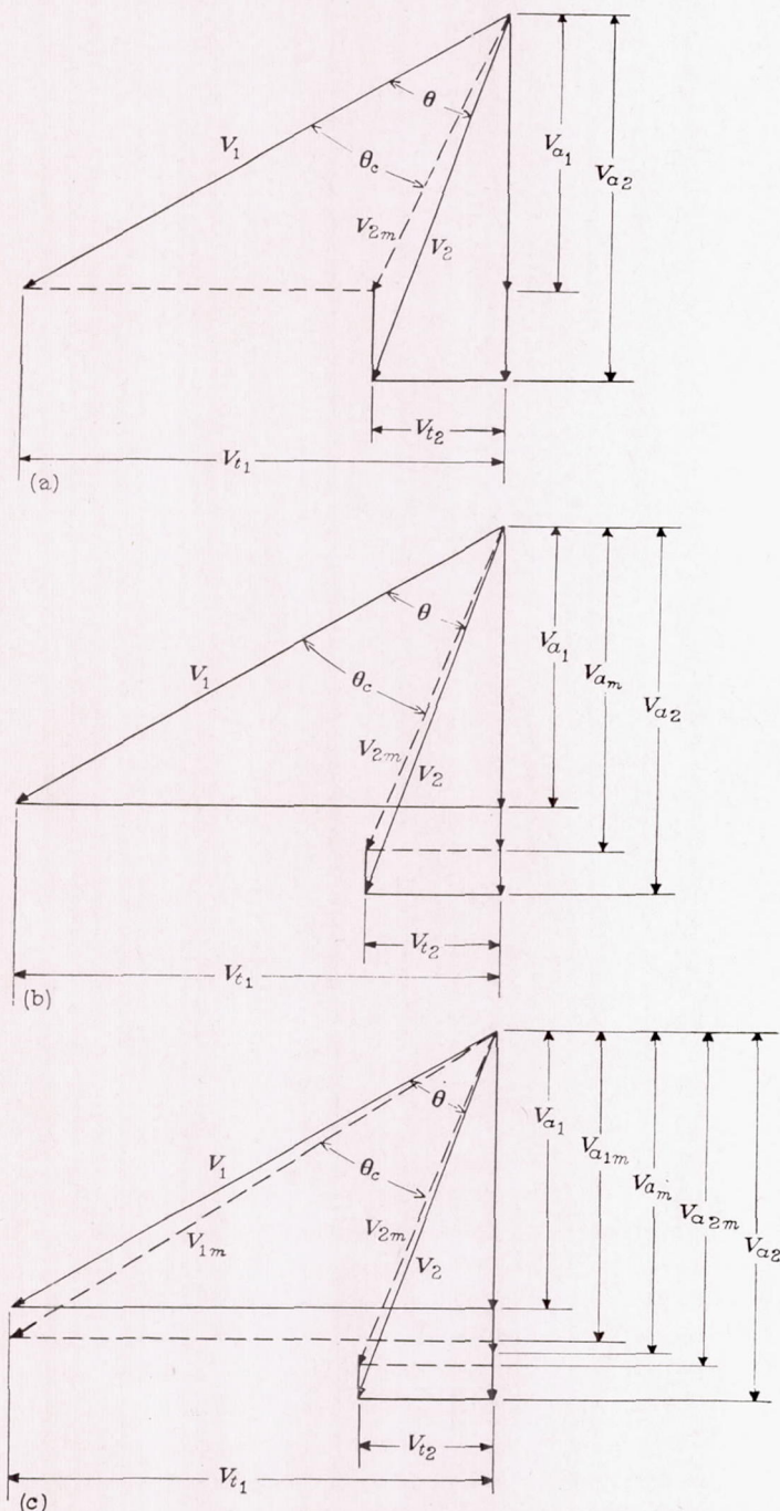
(a) Method I. (b) Method II. (c) Method III. FIGURE 25.—Velocity diagrams illustrating several correction methods.
