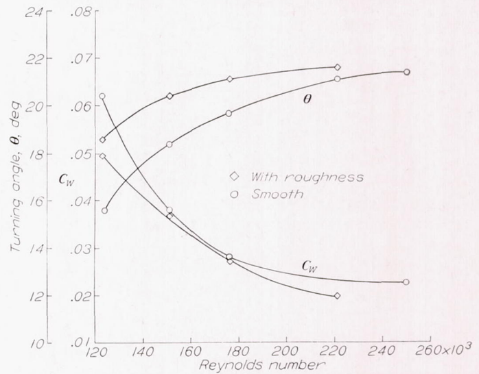
FIGURE 22.—Effect of roughness on cascade performance over a range of Reynolds numbers. Tests were made in 5-inch solid-wall cascade of aspect ratio 2.
