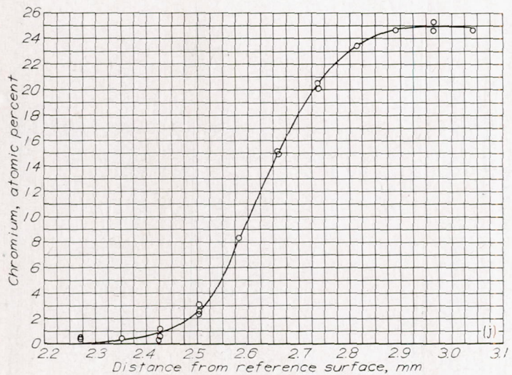
FIGURE 9.—Concluded. Concentration-penetration curves.
