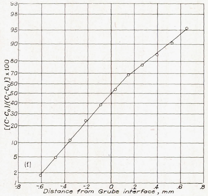
(f) Specimen 5; annealed at 1299° C for 11.05 days.
