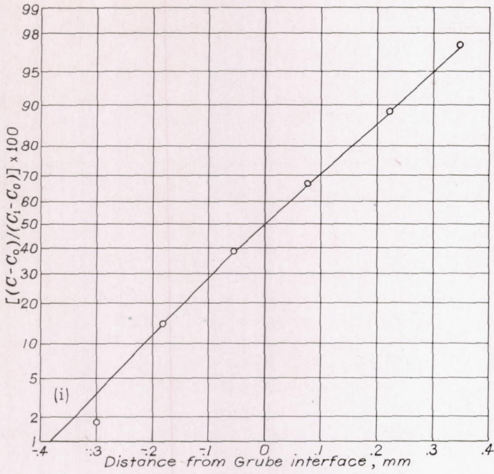
(i) Specimen 7; annealed at 1151° C for 24.91 days.
