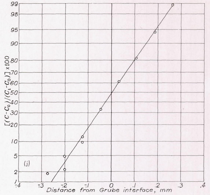
(j) Specimen 8; annealed at 1000° C for 87.7 days.
