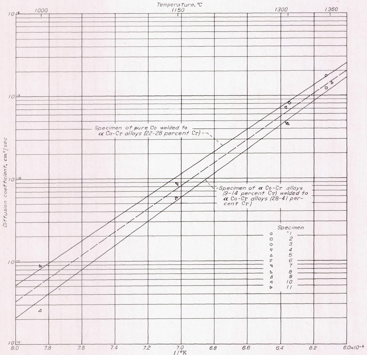
FIGURE 13.—Diffusion coefficients against 1/^\circ\text{K} . Diffusion coefficients were plotted from data for 16-atomic-percent chromium.
