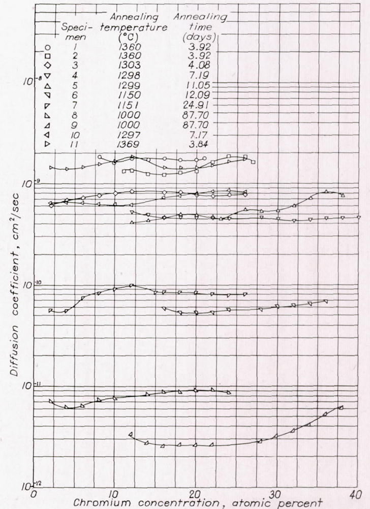
FIGURE 11.—Diffusion coefficients against concentration. (Data to left of 8 atomic percent not plotted for specimen 1 because of quench crack that formed after diffusion took place.)
