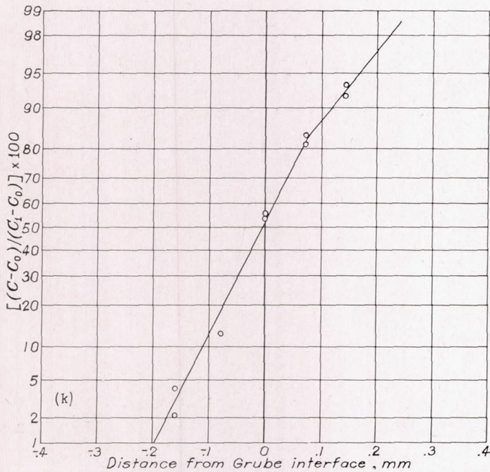
(k) Specimen 9; annealed at 1000° C for 87.7 days.
