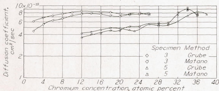
FIGURE 12.—Comparison of diffusion coefficients calculated by the Grube and Matano methods.
