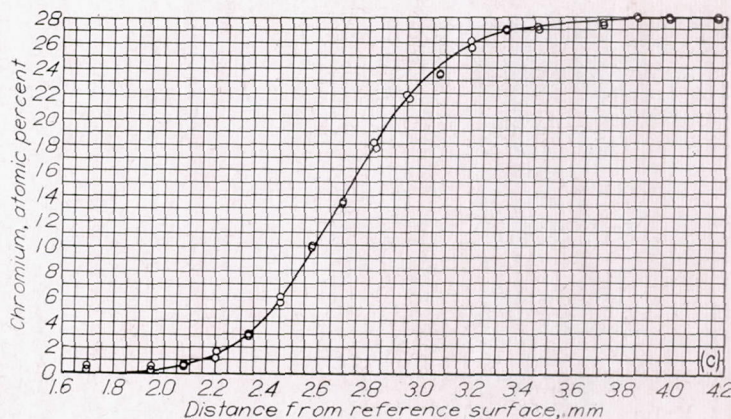
(c) Specimen 11; annealed at 1369° C for 3.321 \times 10^5 seconds (3.84 days).
