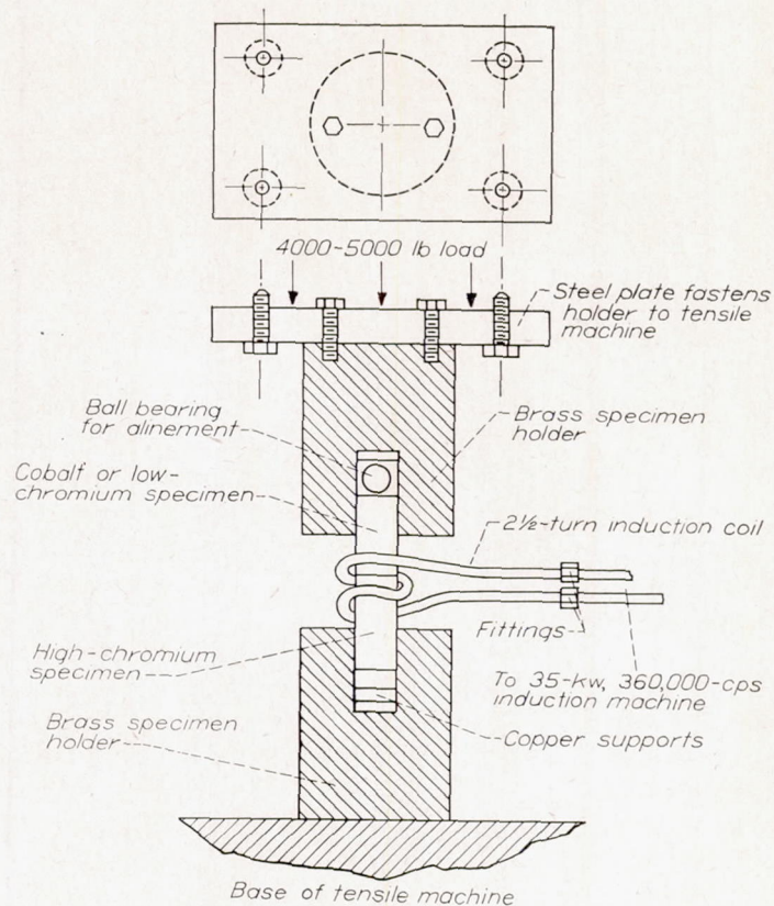
FIGURE 2.—Pressure-welding apparatus.
