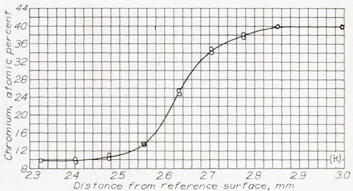
FIGURE 9.—Concluded. Concentration-penetration curves.
