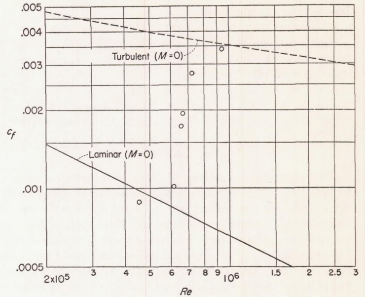
FIGURE 21.—Transition on flat plate. M \approx 0.24 to M \approx 0.6 .
