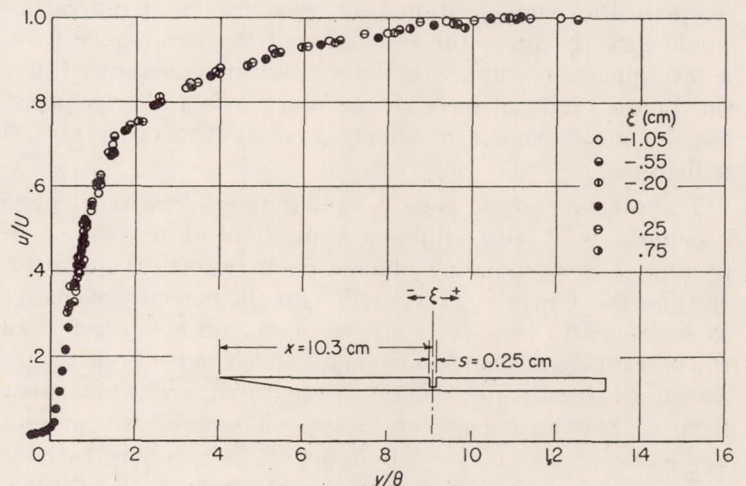
FIGURE 3.—Velocity profiles on flat plate with turbulent boundary layer and slot. Re_s \approx 4 \times 10^4 ; Re_s \approx 1000 .
