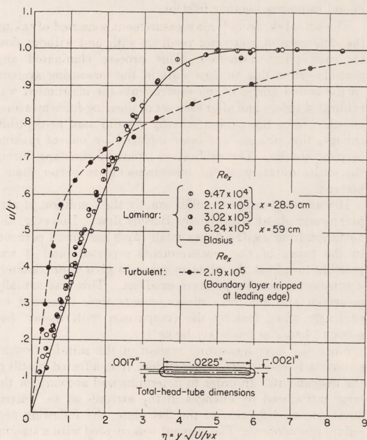
FIGURE 12.—Boundary-layer profiles on flat plate. Incompressible flow.
