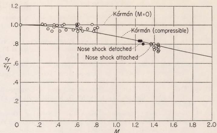
FIGURE 23.—Effect of compressibility on local skin friction on flat plate. Turbulent boundary layer; Reynolds number Re \approx 10^6 .
