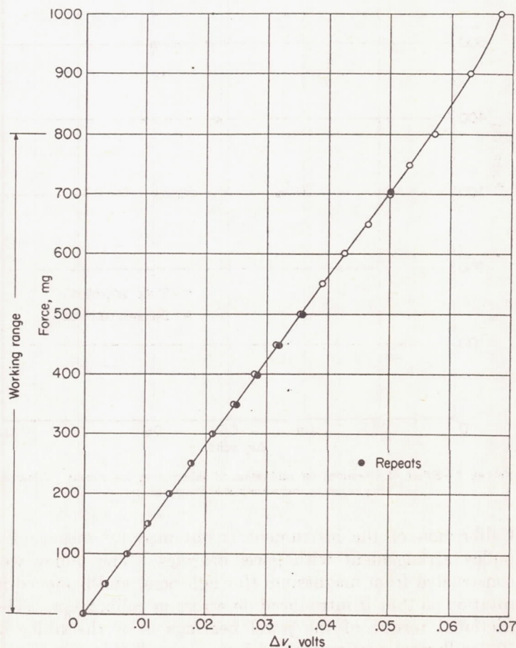
FIGURE 9.—Calibration curve of skin-friction instrument. 0.01-by \frac{1}{4} -inch steel links; \tau_0 = 38.3 \times 10^3 \times \Delta , dynes per square centimeter.
