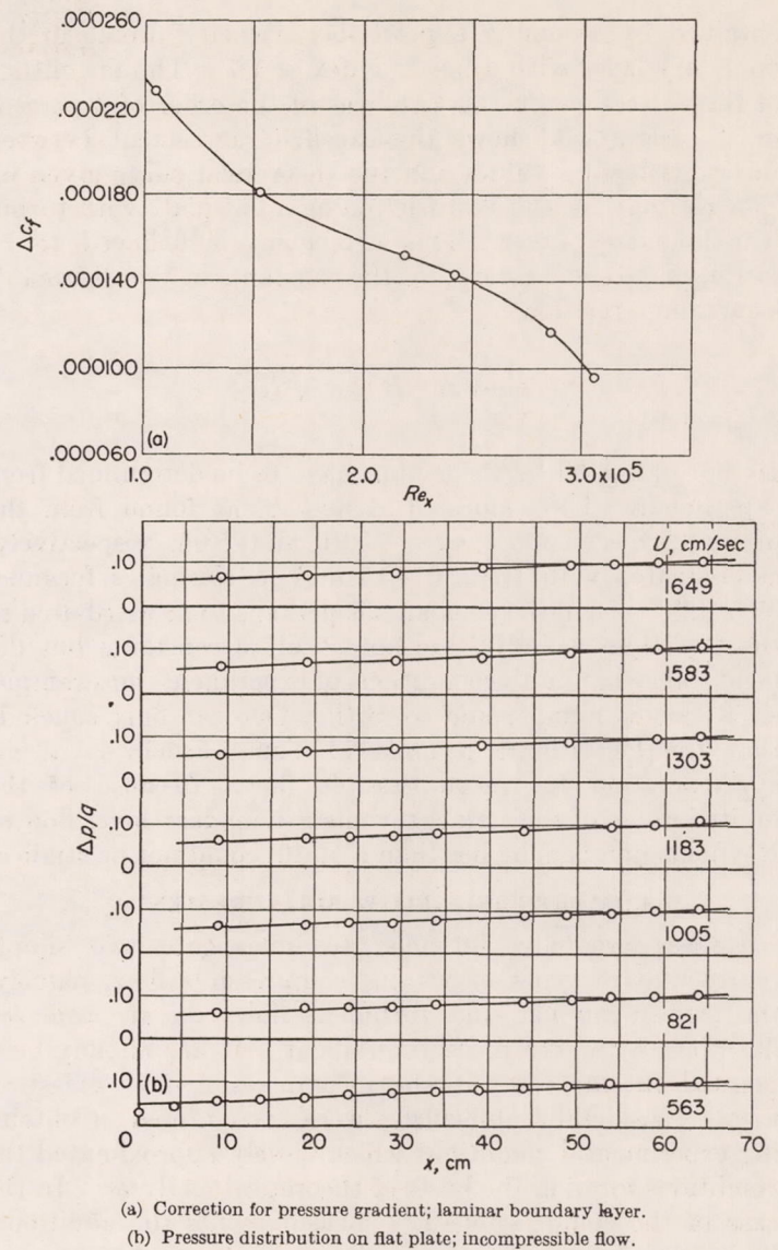
FIGURE 15.—Pressure-gradient measurements.
