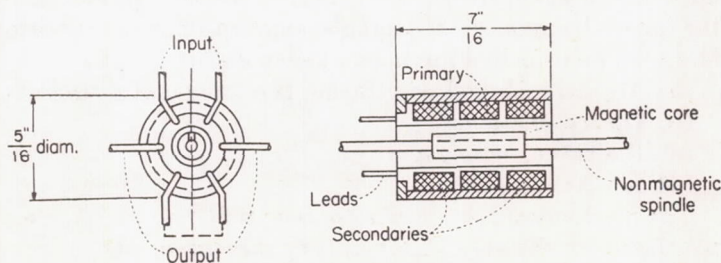
FIGURE 4.—Differential transformer.
