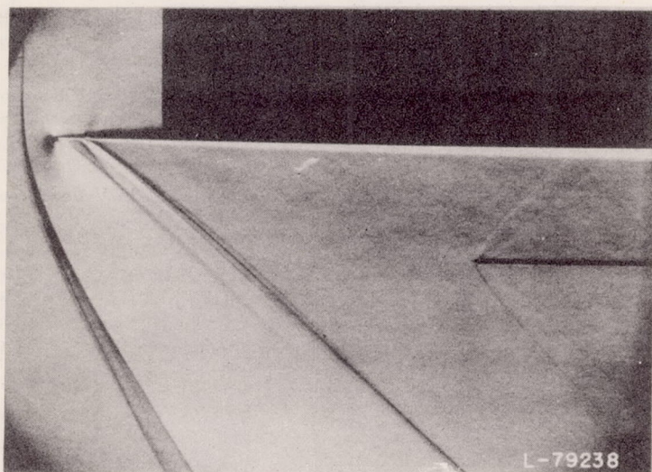
FIGURE 22.—Schlieren photograph of flow past flat plate. With detached bow wave.
