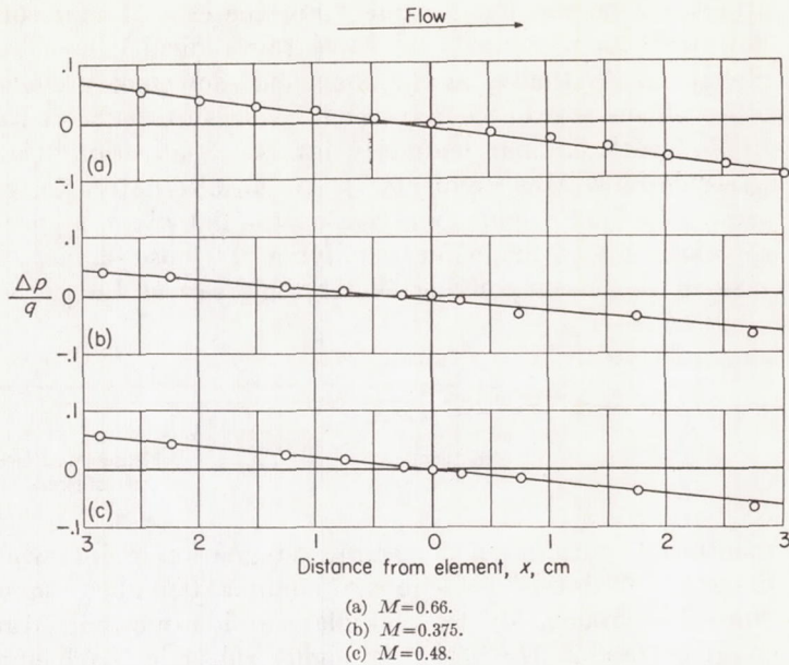
FIGURE 20.—Representative pressure distributions on flat plate with laminar boundary layer. Subsonic flow.
