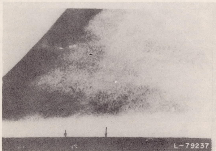
FIGURE 2.—Effect of slots in plate. Turbulent boundary layer; M \approx 1.4 ; flow from left to right; arrows indicate position of slots.
