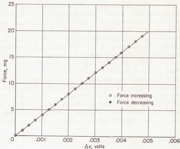
FIGURE 8.—Calibration of skin-friction instrument. Input, 5 volts at 20 kilocycles; 0.0005-by \frac{1}{4} -inch links; \tau_0 = 39.25 \times \Delta , dynes per square centimeter.
