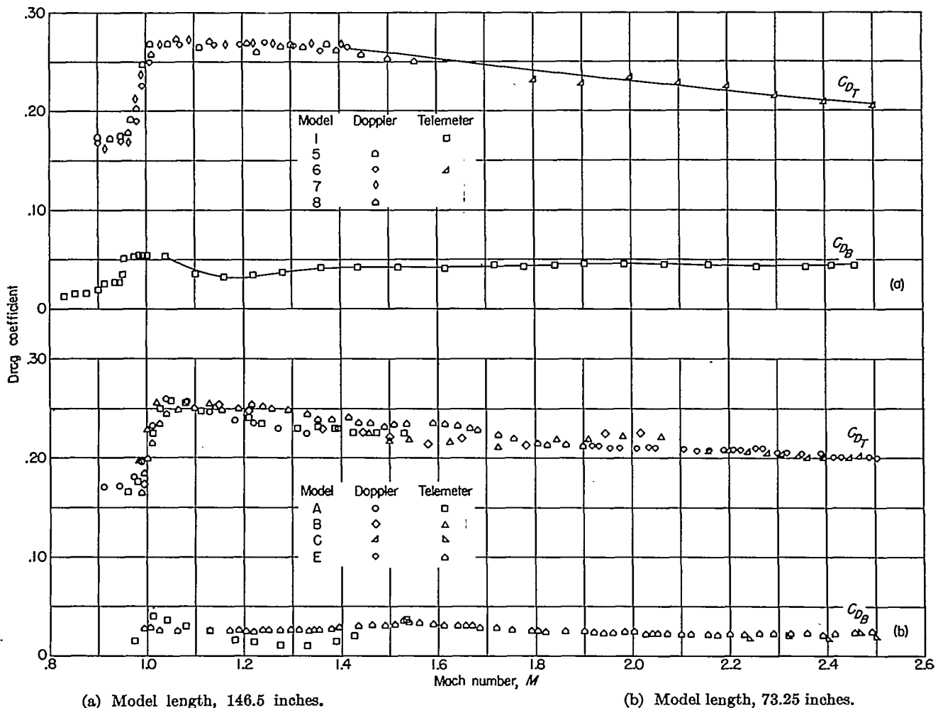
FIGURE 9.—Variation of drag coefficient with Mach number for flight models. \alpha=0^\circ .
