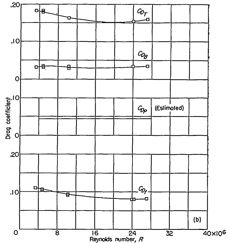
(b) Transition fixed near body nose.
