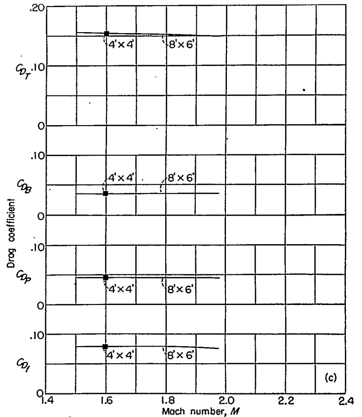
(c) R \approx 30 \times 10^6 . FIGURE 12.—Concluded.
