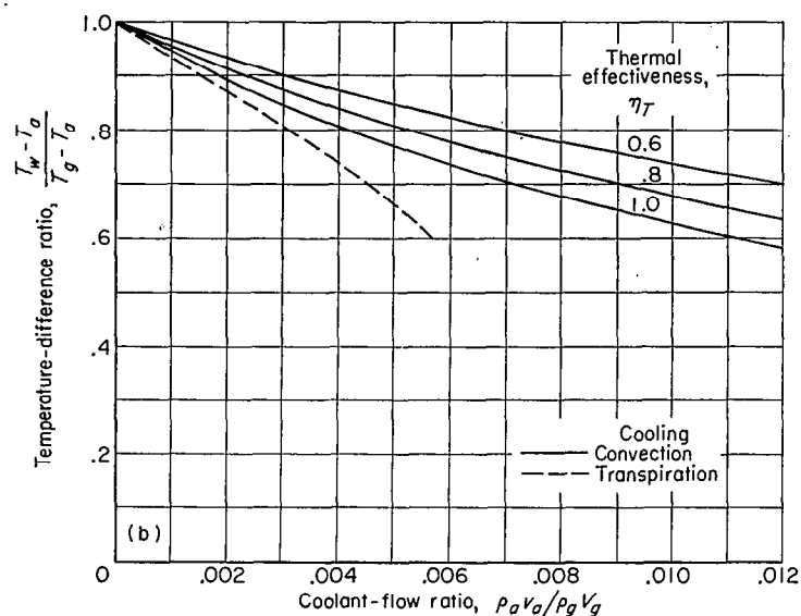
(b) Laminar flow with radiation. Reynolds number, Re_g, 10^4 .
