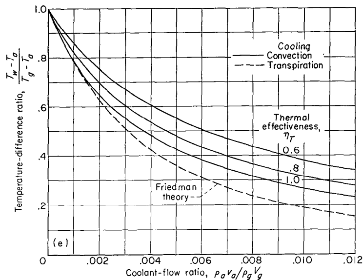
(e) Turbulent flow with radiation. Reynolds number, Re_g , 10^7 . \bar{h}_r/\bar{h}_{g,co}=1 .
