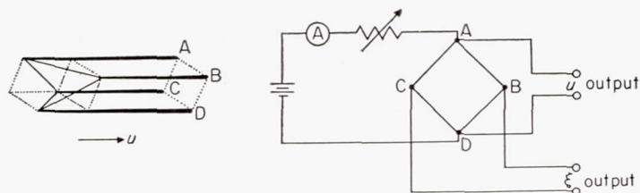
FIGURE 10.—Vorticity meter.
