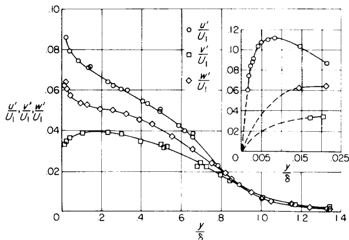
FIGURE 4. Distribution of turbulence intensities.
