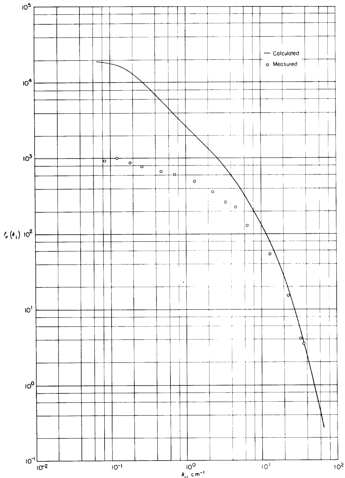
FIGURE 9.—Comparison of measured \bar{v}^2 spectrum with that calculated from measured \bar{u}^2 spectrum using isotropic relation; y/\delta=0.05 .
