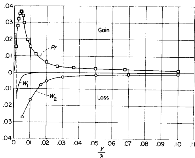
FIGURE 23.—Production and dissipation in region near wall.
