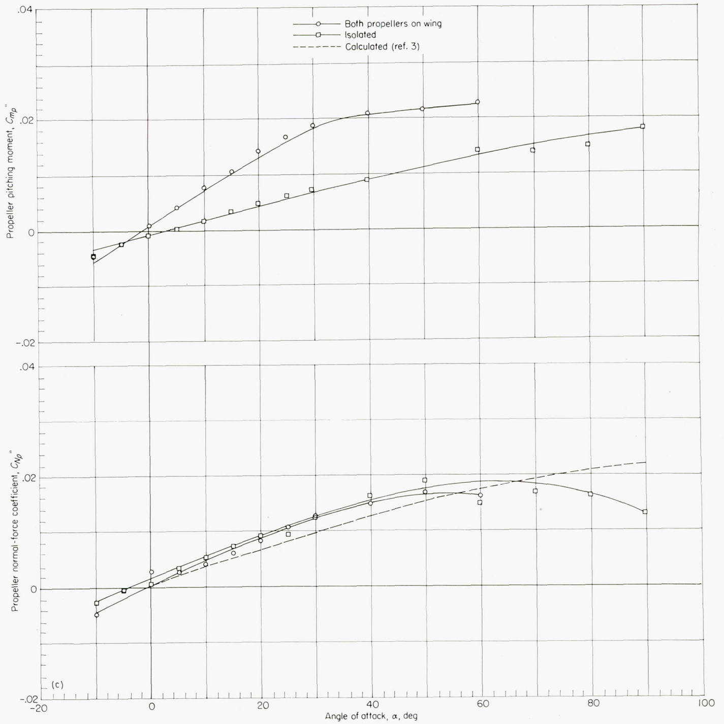
(c) T_c'' = 0.50 . FIGURE 12.—Concluded.
