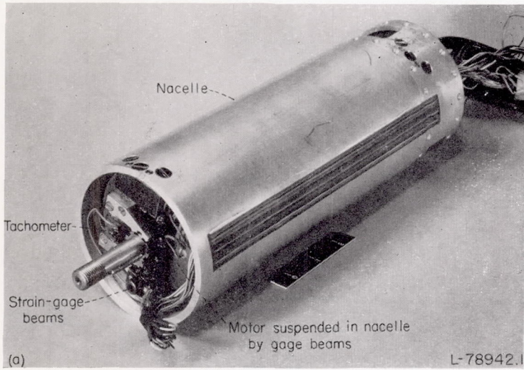
(a) Complete motor balance.
