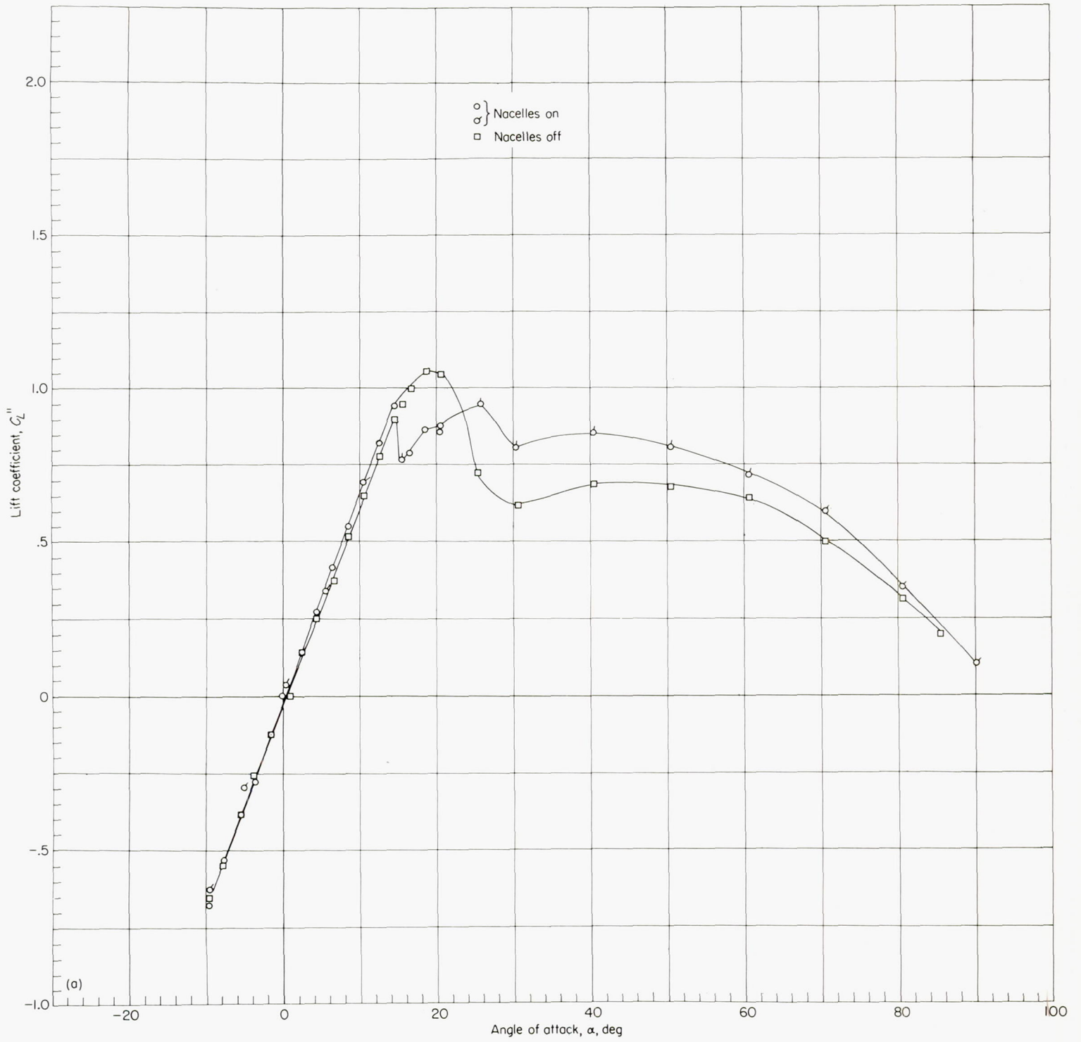
(a) Lift coefficient. FIGURE 20.—Effect of nacelles on aerodynamic characteristics of the model with propellers off. (Flagged symbols indicate check tests.)
