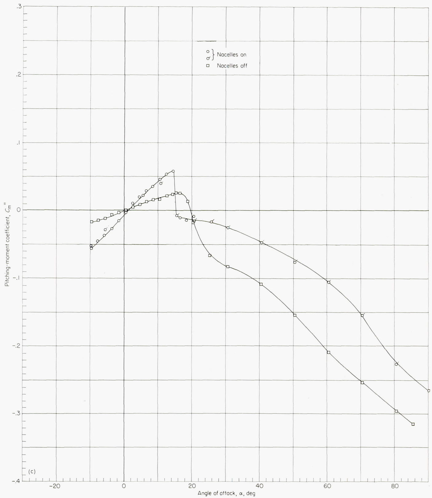
(c) Pitching-moment coefficient.
