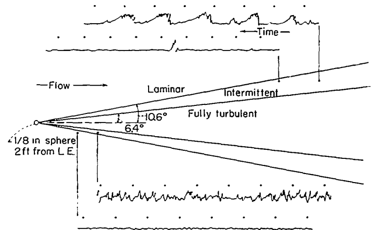
FIGURE 5.—Turbulence wedge produced by three-dimensional roughness element ( \frac{1}{8} -inch sphere) on surface. Time interval between dots, 1/60 second; U_1 = 80 feet per second.
