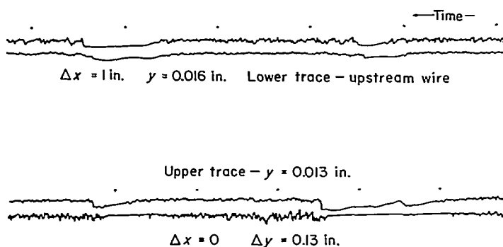
FIGURE 8.—Simultaneous signals from two hot-wires in region of natural transition. Time progression from right to left; time interval between dots, \frac{1}{60} second; upper record, 1-inch separation in x ; lower record, 0.13-inch separation in y
