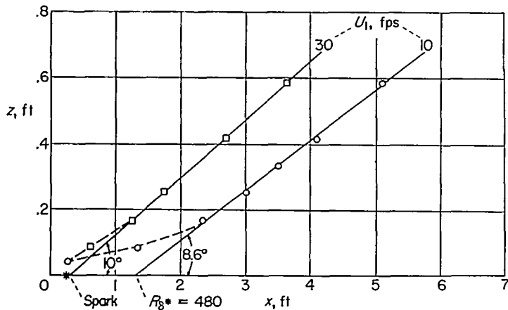
FIGURE 7.—Envelopes of spot growth. R_{B^*} , Reynolds number based on laminar-boundary-layer displacement thickness.
