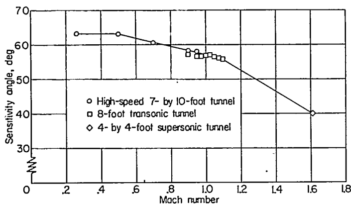
FIGURE 13.—Variation of sensitivity angle with Mach number of shielded tube A r -16.
