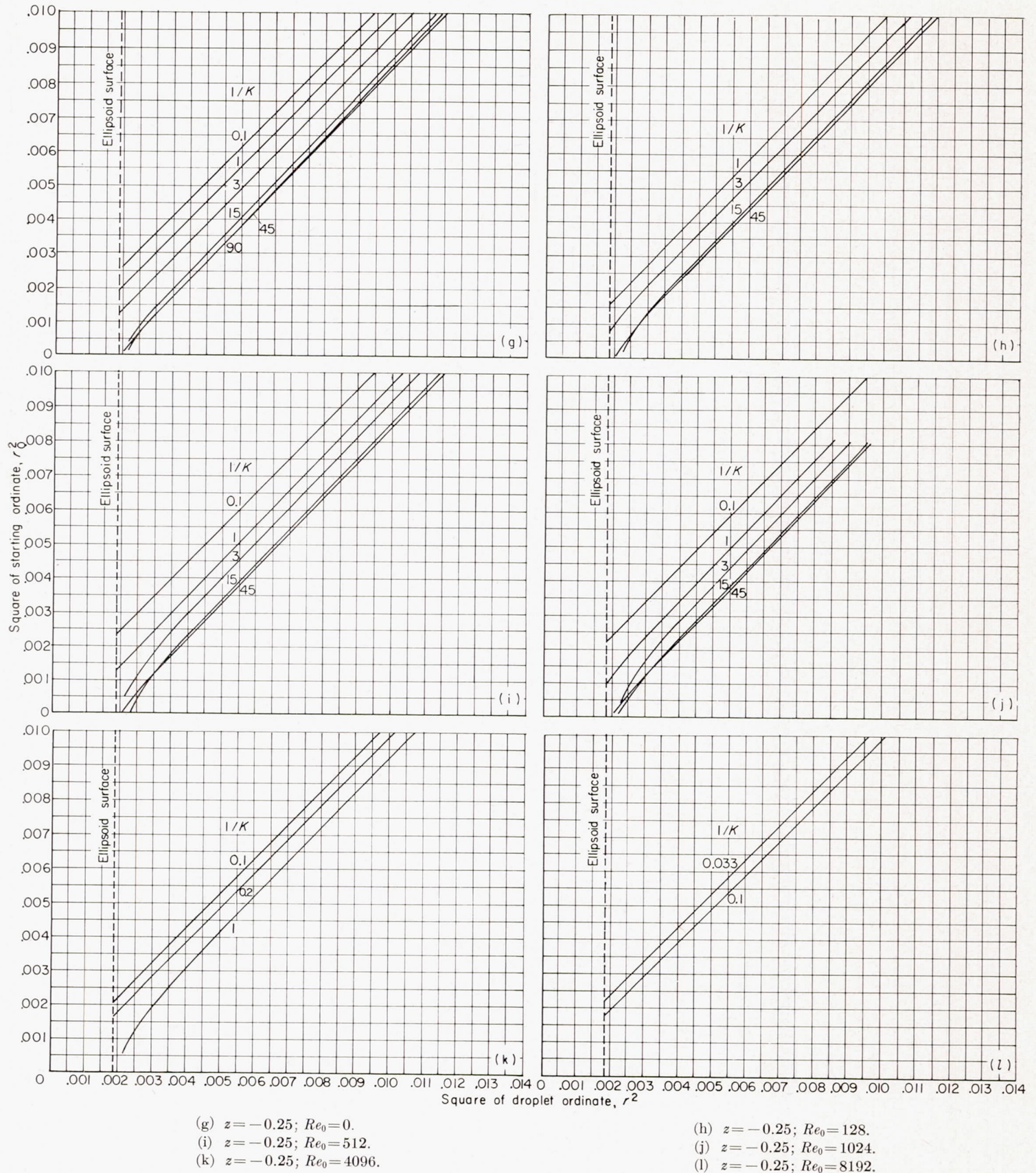
FIGURE 7.—Continued. Square of starting ordinate as function of square of droplet ordinate at constant axial position. Basic ellipsoid, 10 percent thick; inlet velocity ratio, 1.0.
