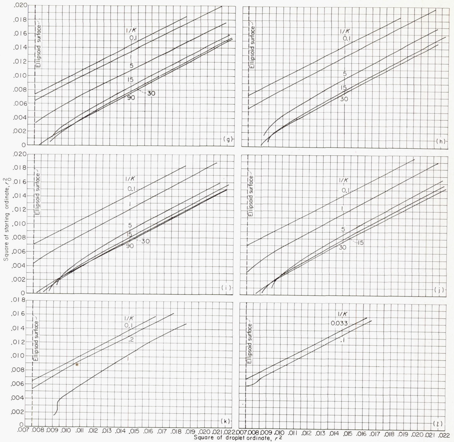
FIGURE 14.—Continued. Square of starting ordinate as function of square of droplet ordinate at constant axial position. Basic ellipsoid, 20 percent thick; inlet velocity ratio, 1.0.
