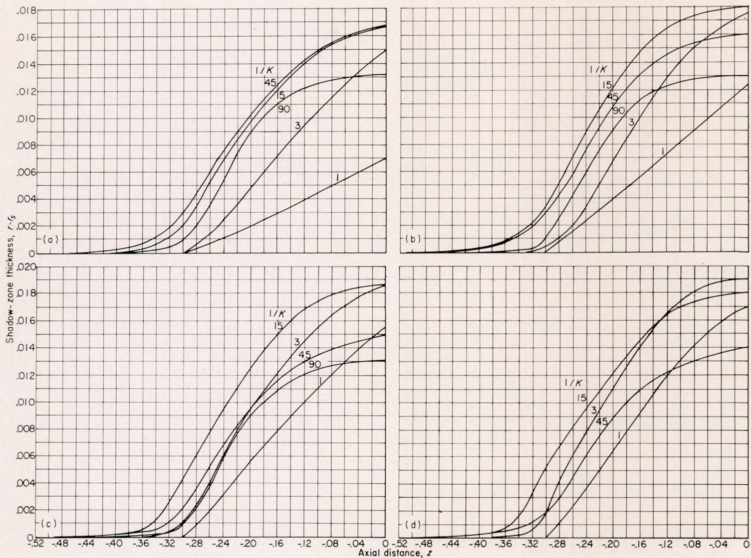
(a) Free-stream Reynolds number, 0. (b) Free-stream Reynolds number, 128. (c) Free-stream Reynolds number, 512. (d) Free-stream Reynolds number, 1024. FIGURE 23.—Thickness of shadow zone along inlet inner wall. Inlet velocity ratio, 0.7; angle of attack, 0^\circ .
