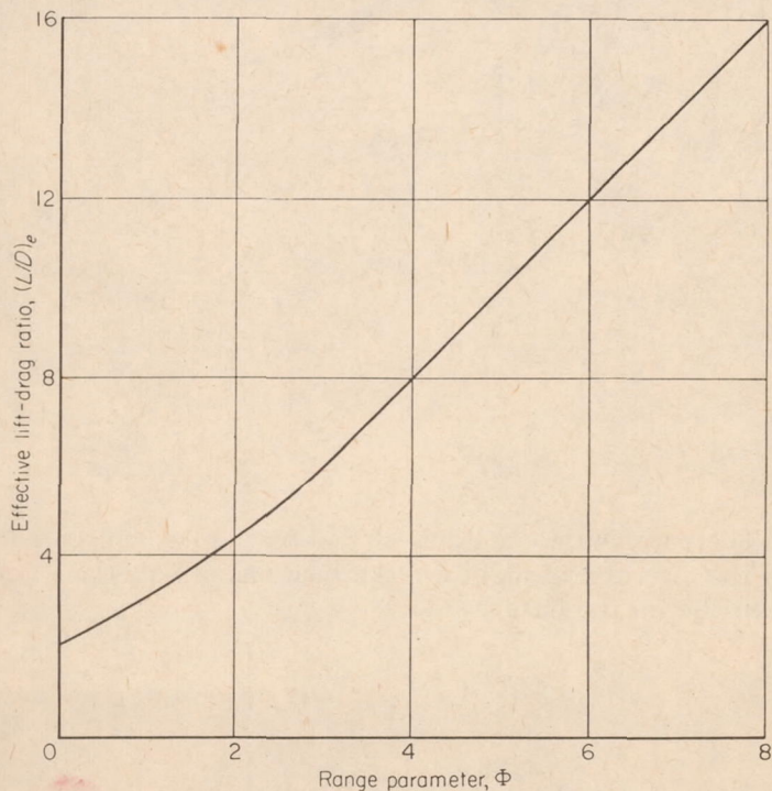
FIGURE 2.—Variation of effective lift-drag ratio with range for optimum ballistic vehicle.
