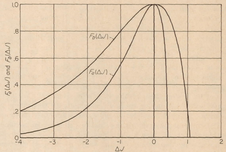
FIGURE 8.—Variations of F_a(\Delta J) and F_b(\Delta J) with \Delta J .
