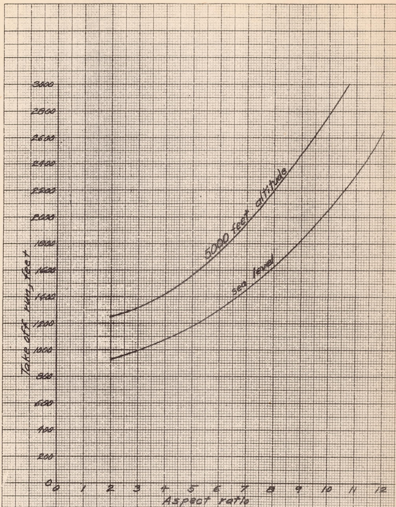
FIGURE 10(b) - EFFECT OF ASPECT RATIO ON TAKE-OFF RUN
