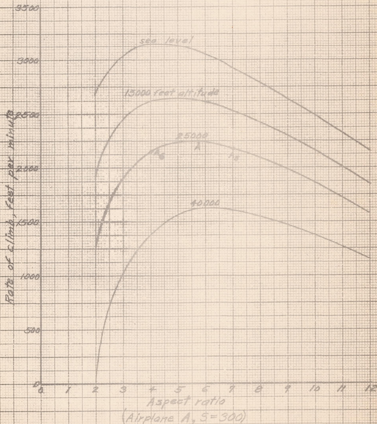
FIGURE 10(C)- EFFECT OF ASPECT RATIO ON RATE OF CLIMB
