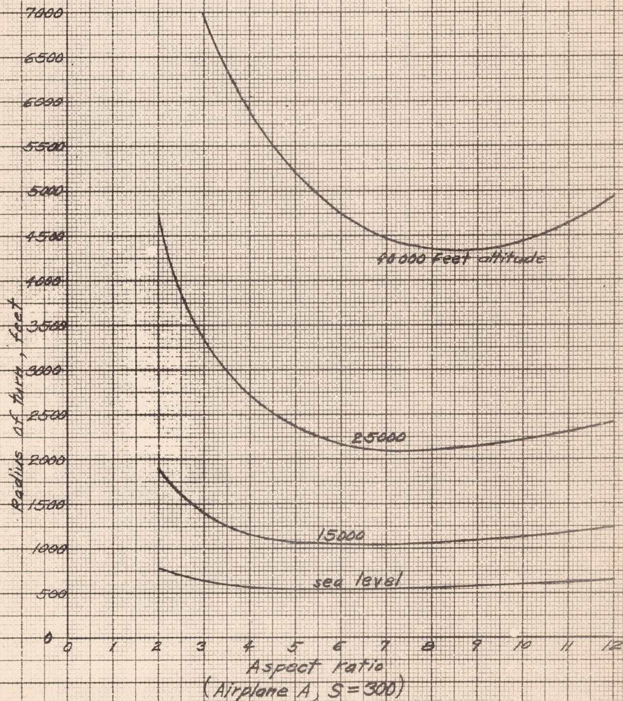
FIGURE 10(e)-EFFECT OF ASPECT RATIO ON RADIUS OF TURN
