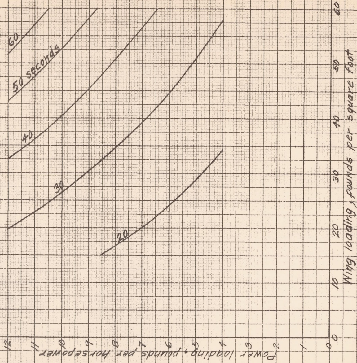
FIGURE 6(b) - TIME TO TURN AT 15,000 FEET ALTITUDE R = 5.75
