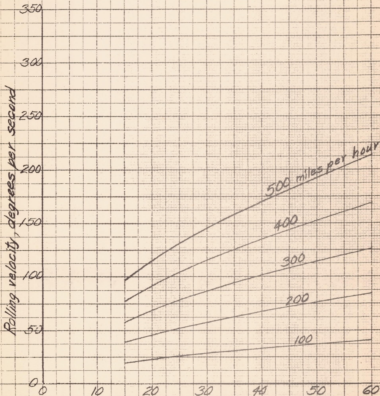
FIGURE 11(f) EFFECT OF WING LOADING ON ROLLING (CONSTANT HELIX)
