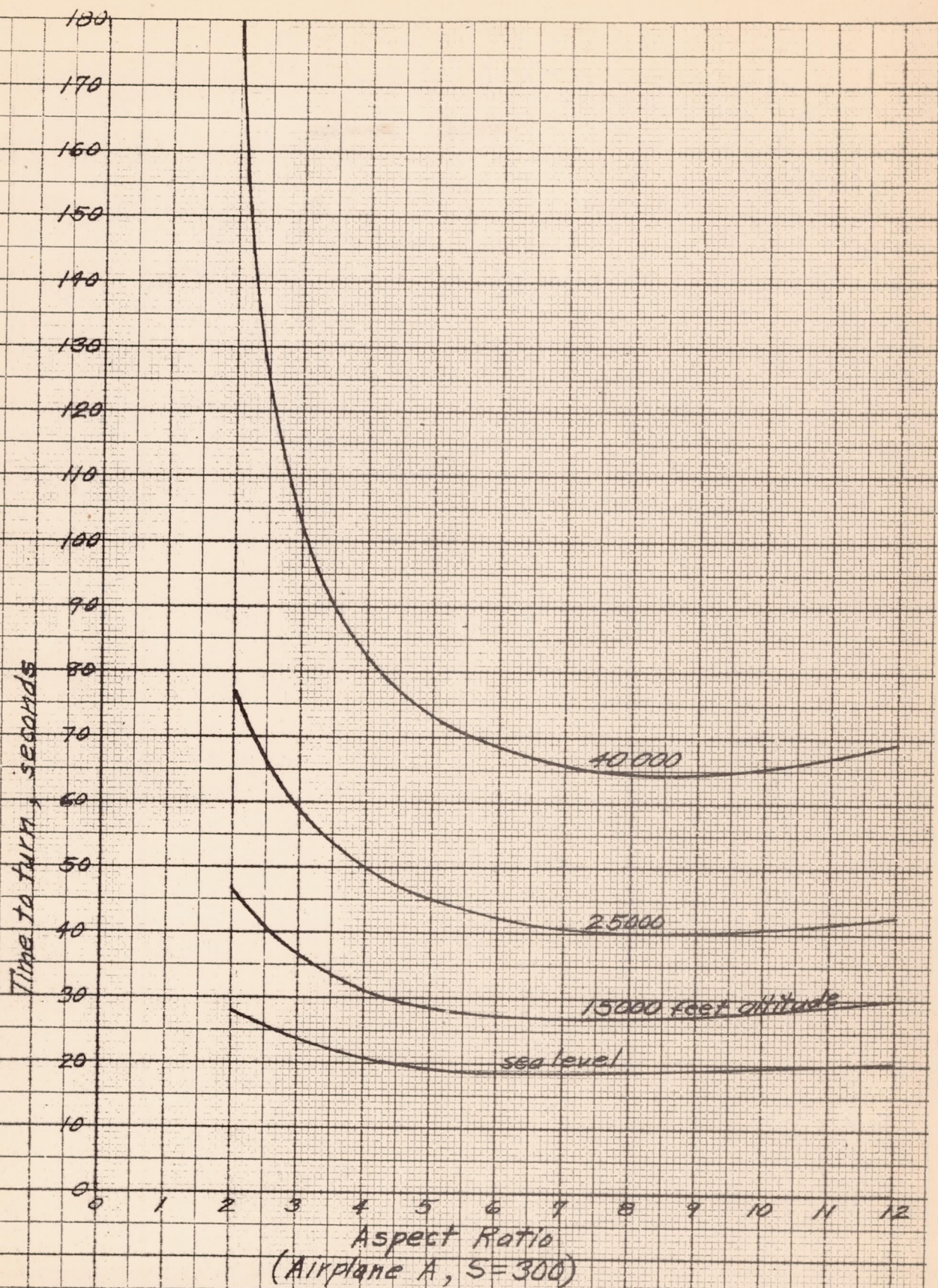
FIGURE 10(f) - EFFECT OF ASPECT RATIO ON TIME TO TURN
