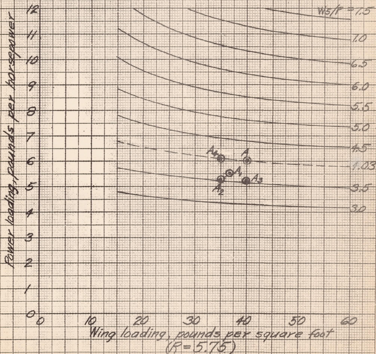
FIGURE 7 - EFFECT OF WING LOADING ON POWER LOADING (CONSTANT LOADS)
