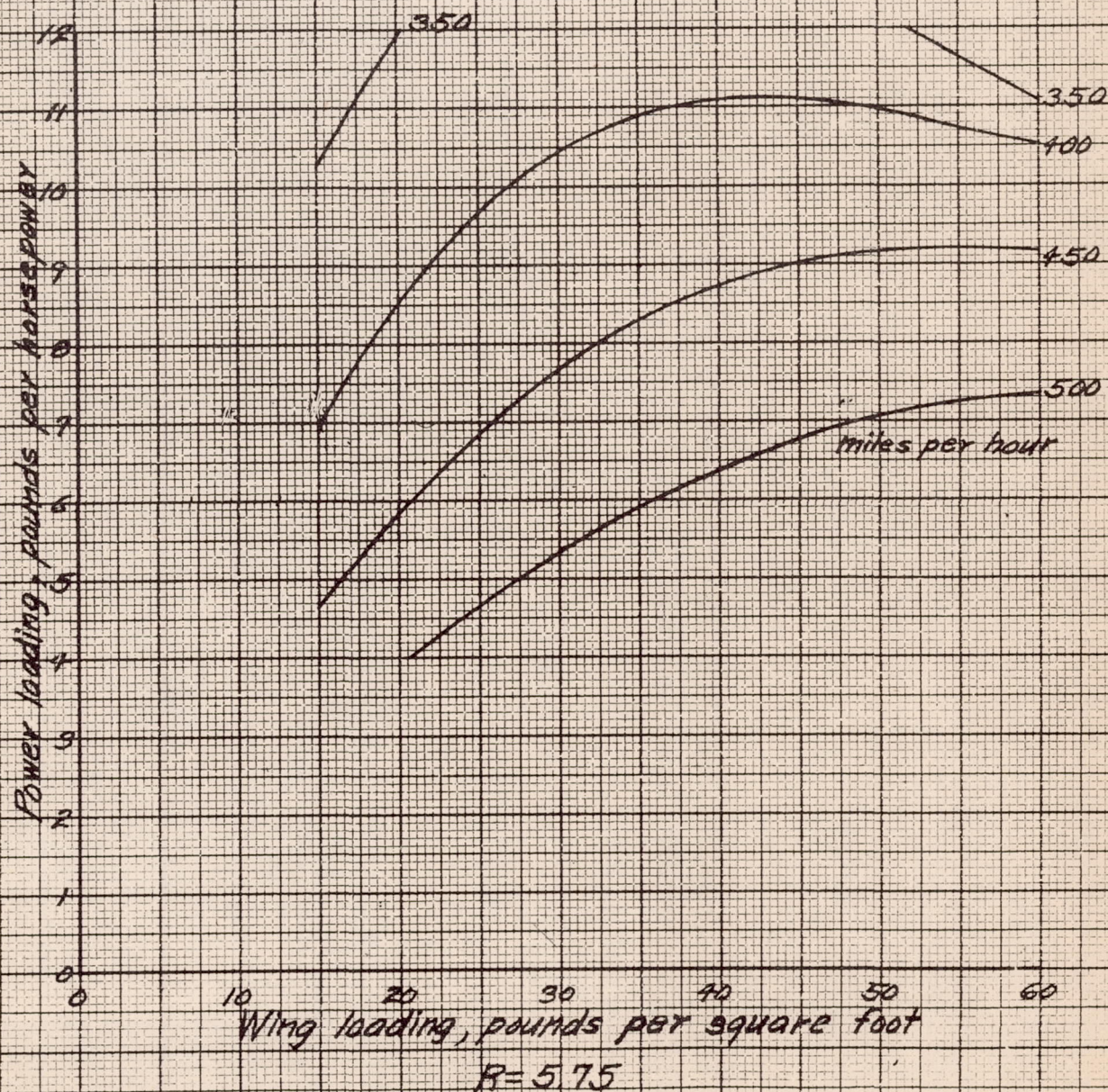
FIGURE 4(d) - HIGH SPEED AT 40,000 FEET ALTITUDE
