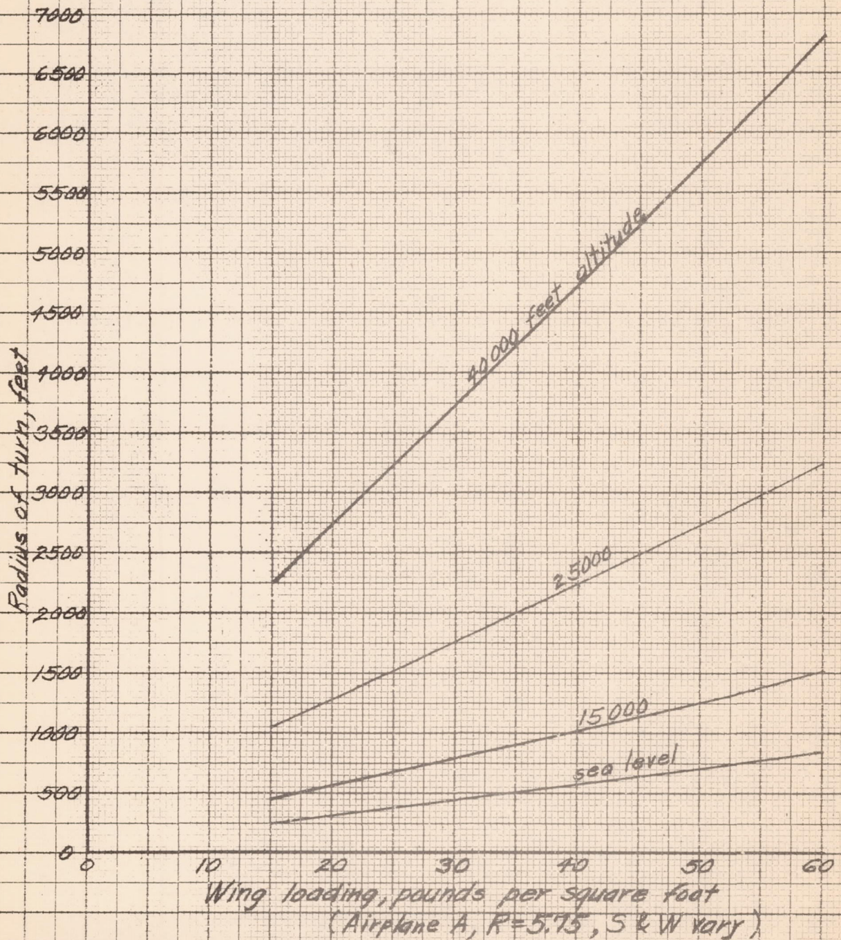
FIGURE 11 (d) EFFECT OF WING LOADING ON RADIUS OF TURN
