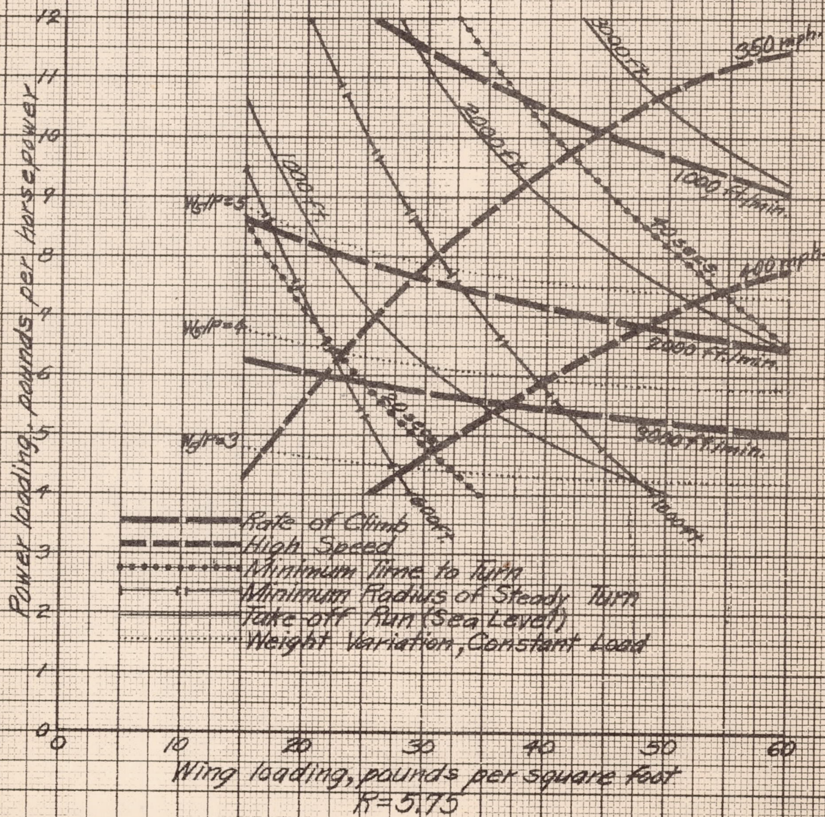
FIGURE 1(b) - COMPOSITE SELECTION CHART - 15,000 FEET ALTITUDE
