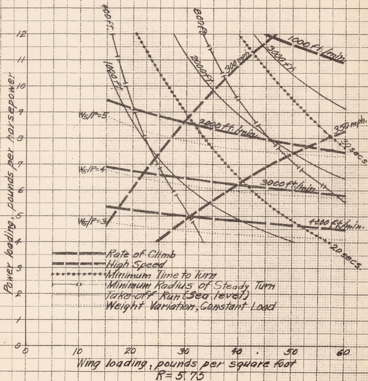
FIGURE 1(a) - COMPOSITE SELECTION CHART - SEA LEVEL
