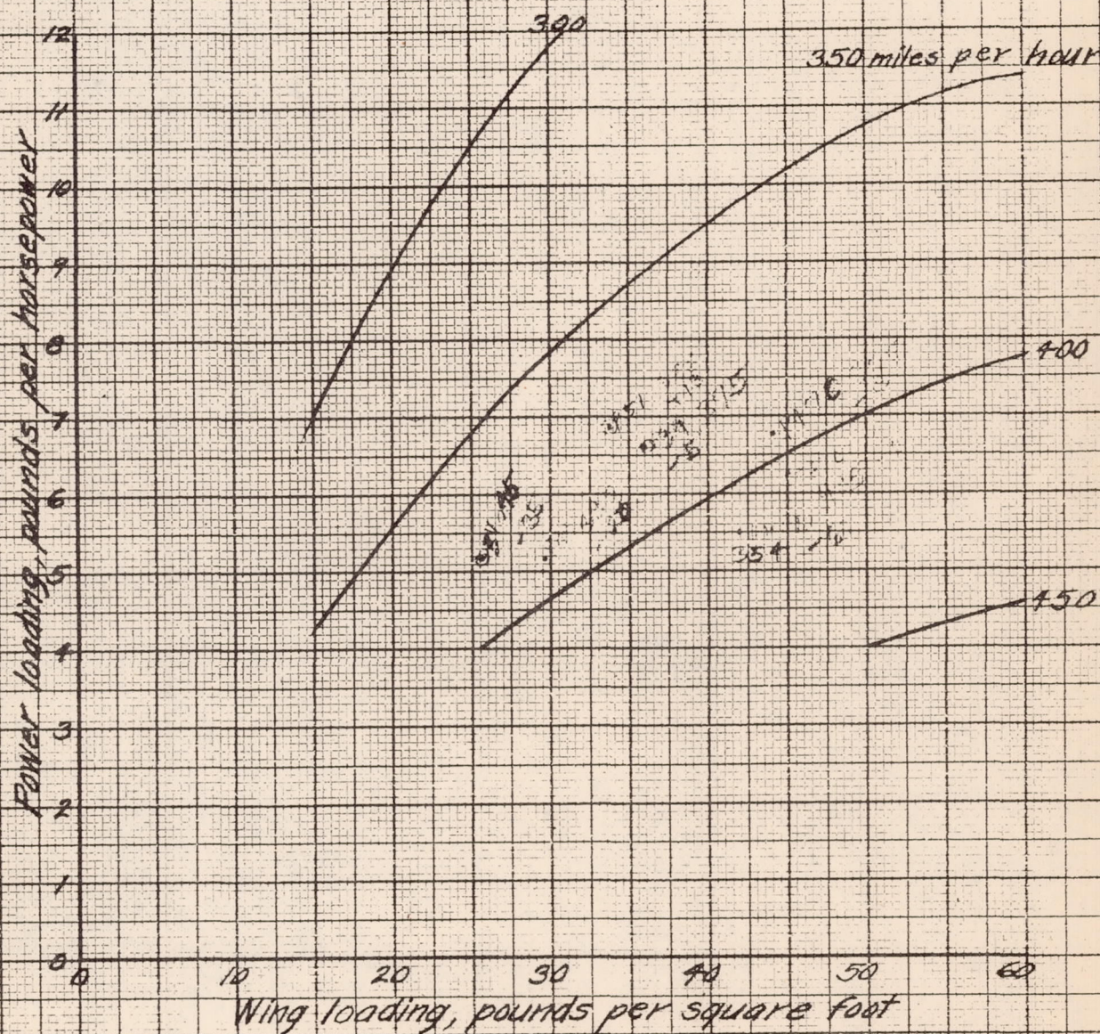
FIGURE 4(b) - HIGH SPEED AT 15000 FEET ALTITUDE
