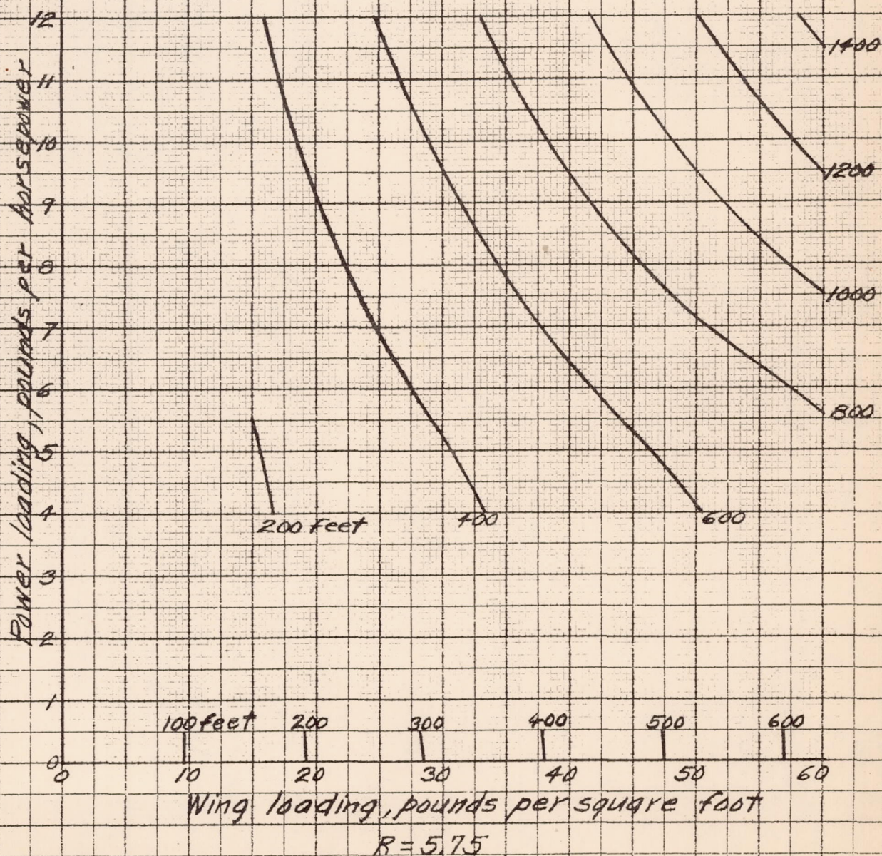
FIGURE 5(a) - RADIUS OF TURN AT SEA LEVEL
