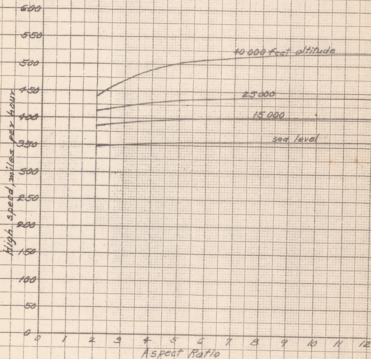
FIGURE 10(d) - EFFECT OF ASPECT RATIO ON HIGH SPEED
