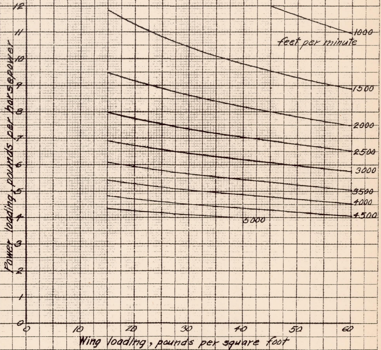
FIGURE 3(a) - RATE OF CLIMB AT SEA LEVEL
