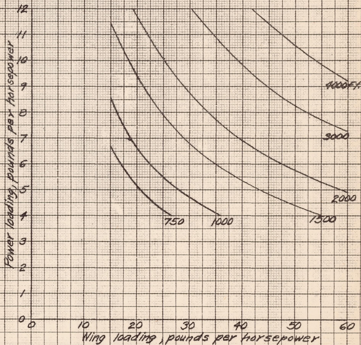
FIGURE 2(b) - TAKE-OFF RUN AT 5000 FEET ALTITUDE
