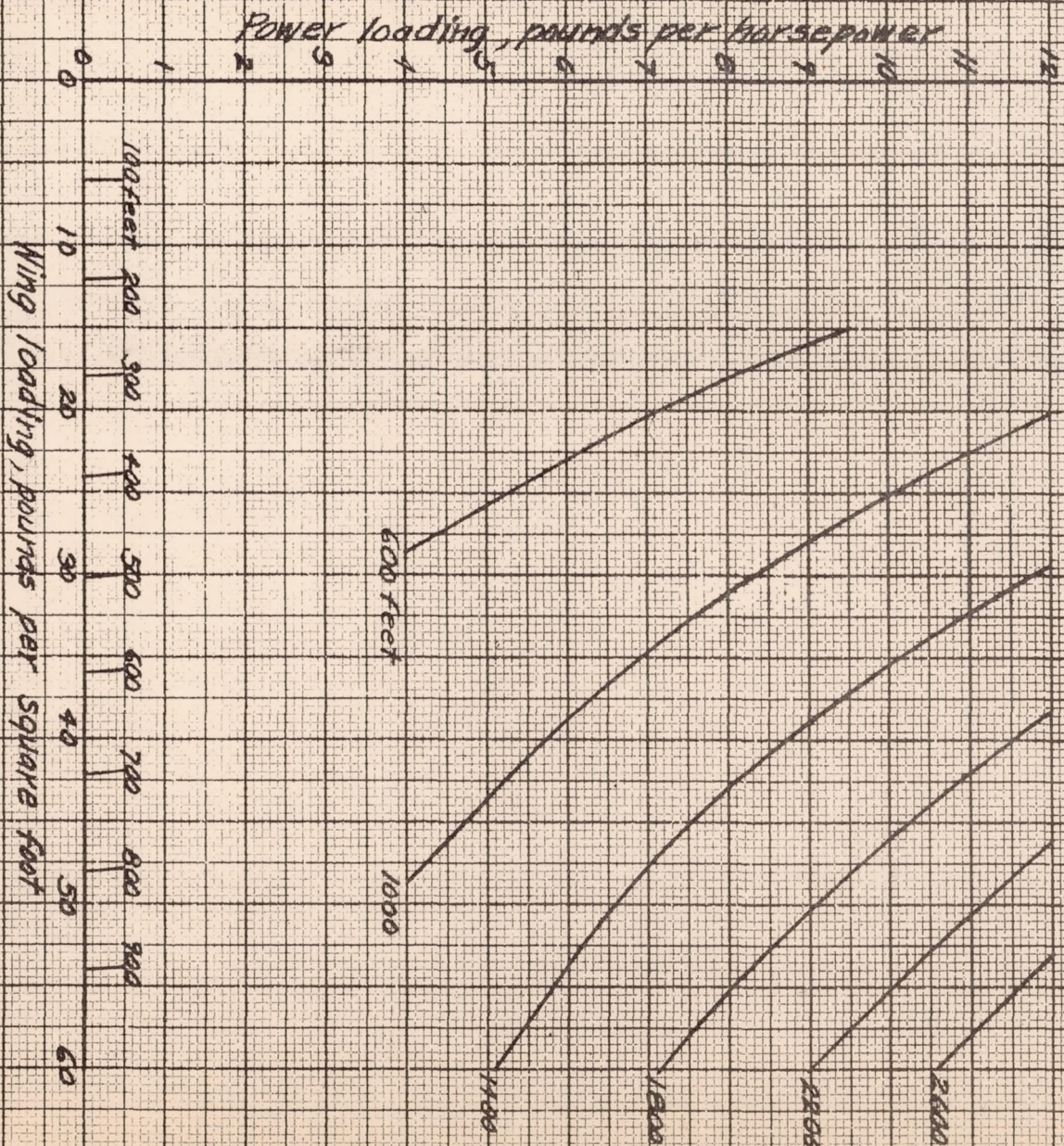
FIGURE 5(a) - RADIUS OF TURN AT 15000 FEET ALTITUDE
