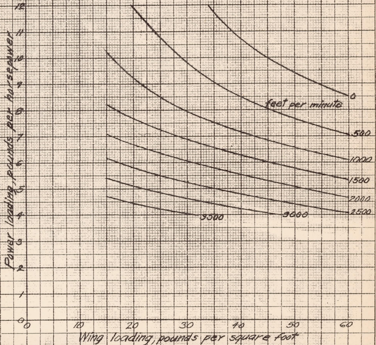
FIGURE 3(d)-RATE OF CLIMB AT 40,000 FEET ALTITUDE
