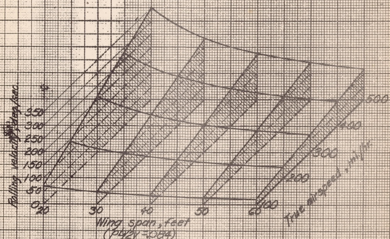
FIGURE B - ROLLING VELOCITY (HELIX ANGLE = CONSTANT)
