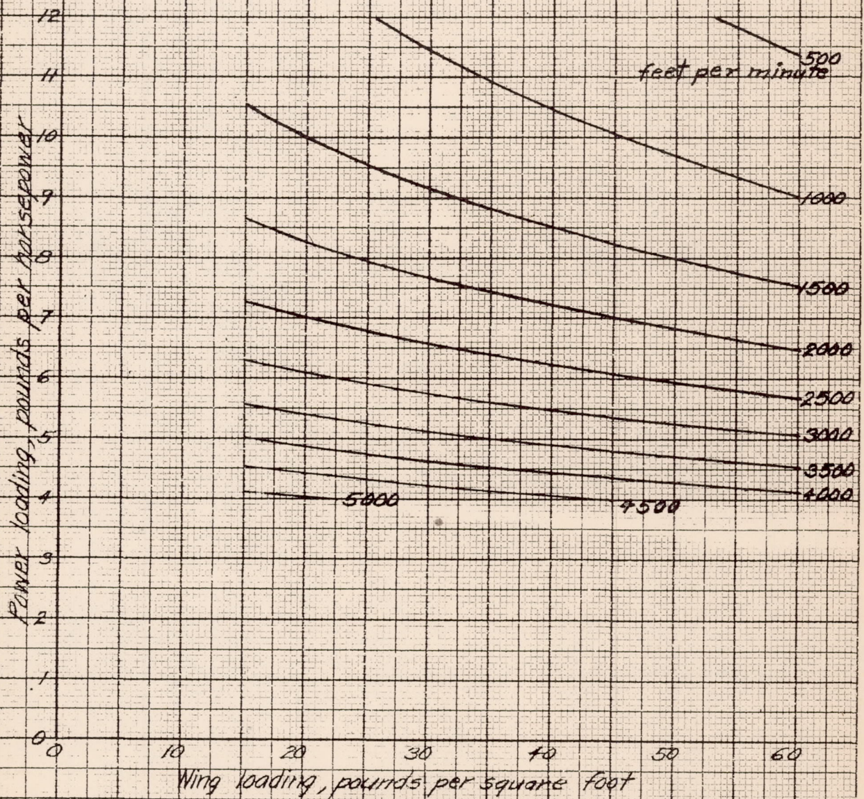
FIGURE 3b) - RATE OF CLIMB AT 15000 FEET ALTITUDE
