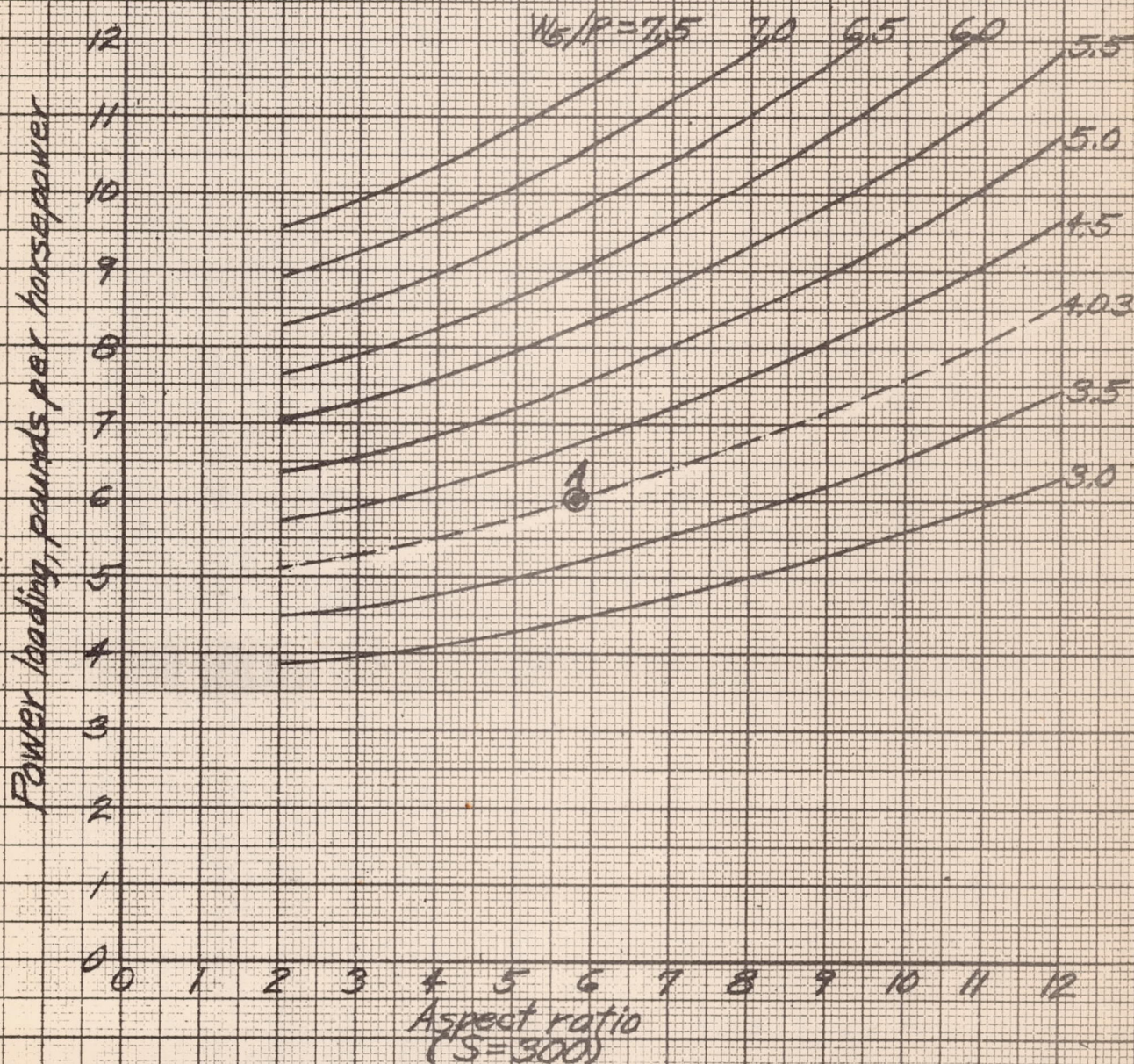
FIGURE 10(a) - EFFECT OF ASPECT RATIO ON POWER LOADING (CONSTANT LOADS)
