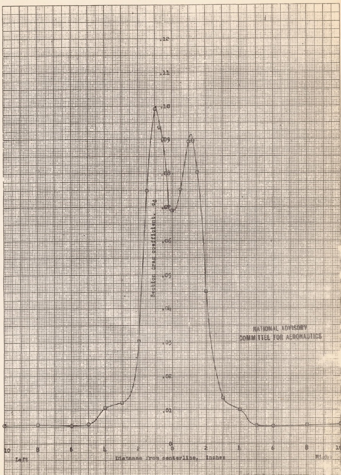
Figure 5.- Spanwise variation of section drag coefficients for the 1/40-scale wing-hull model of the Hughes-Kaiser Cargo Airplane; no wing fillets, step fairings, or roughness; incidence, 7^\circ ; model lift coefficient C_{L_M} = 0.182 ; R, 22.5 \times 10^6 . Test, TDT 325.
