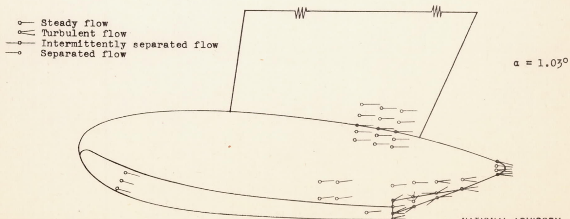
Figure 10.- Tuft observations of the 1/10-scale float-strut model for the Hughes-Kaiser Cargo Airplane; step in float afterbody; float incidence 0^\circ to wing chord; R, 7.0 \times 10^6 . Test, TDT 389.
