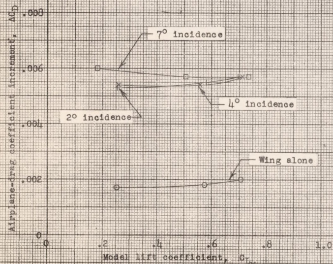
(a) Wing-hull model without wing fillets, step fairings or roughness.
