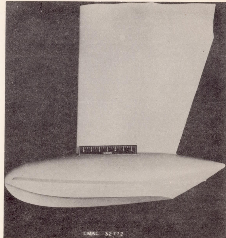
(b) View showing float-strut with spray strip and cove.
