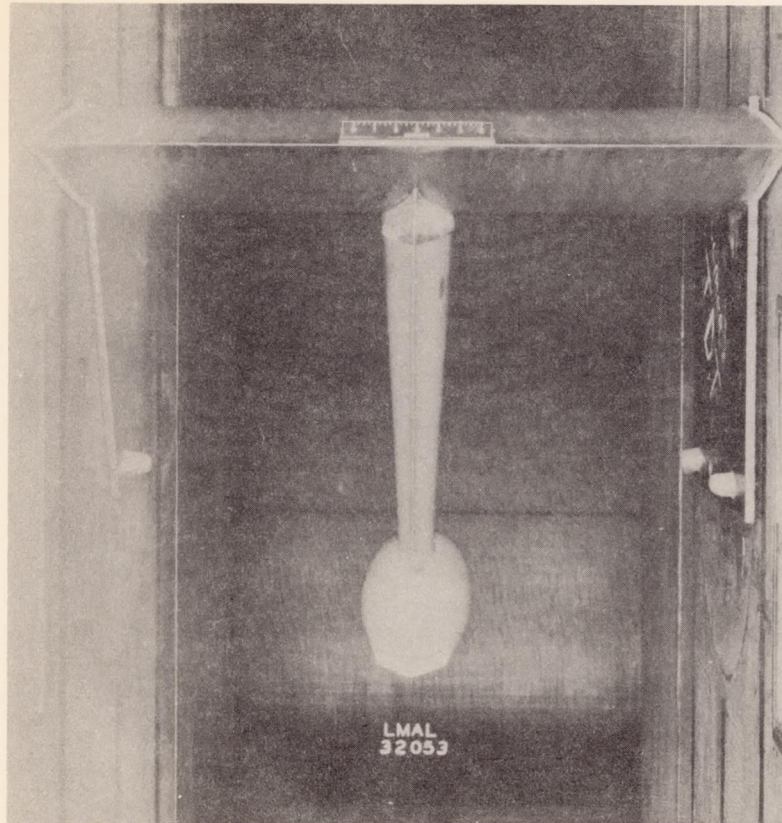
(a) Float-strut model attached to 36-inch-chord airfoil and installed in the tunnel.
