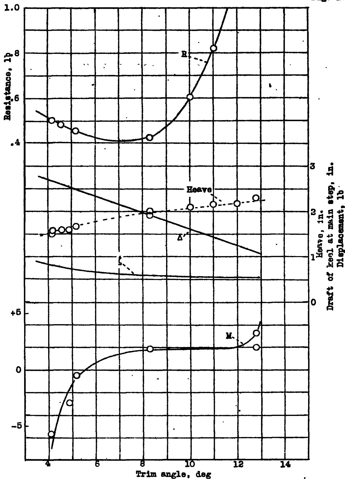
Figure 15.- Model 294-9, steady-state characteristics, equilibrium for assumed aerodynamic characteristics. V_m = 21.18 fps, H_2SO_4 .
