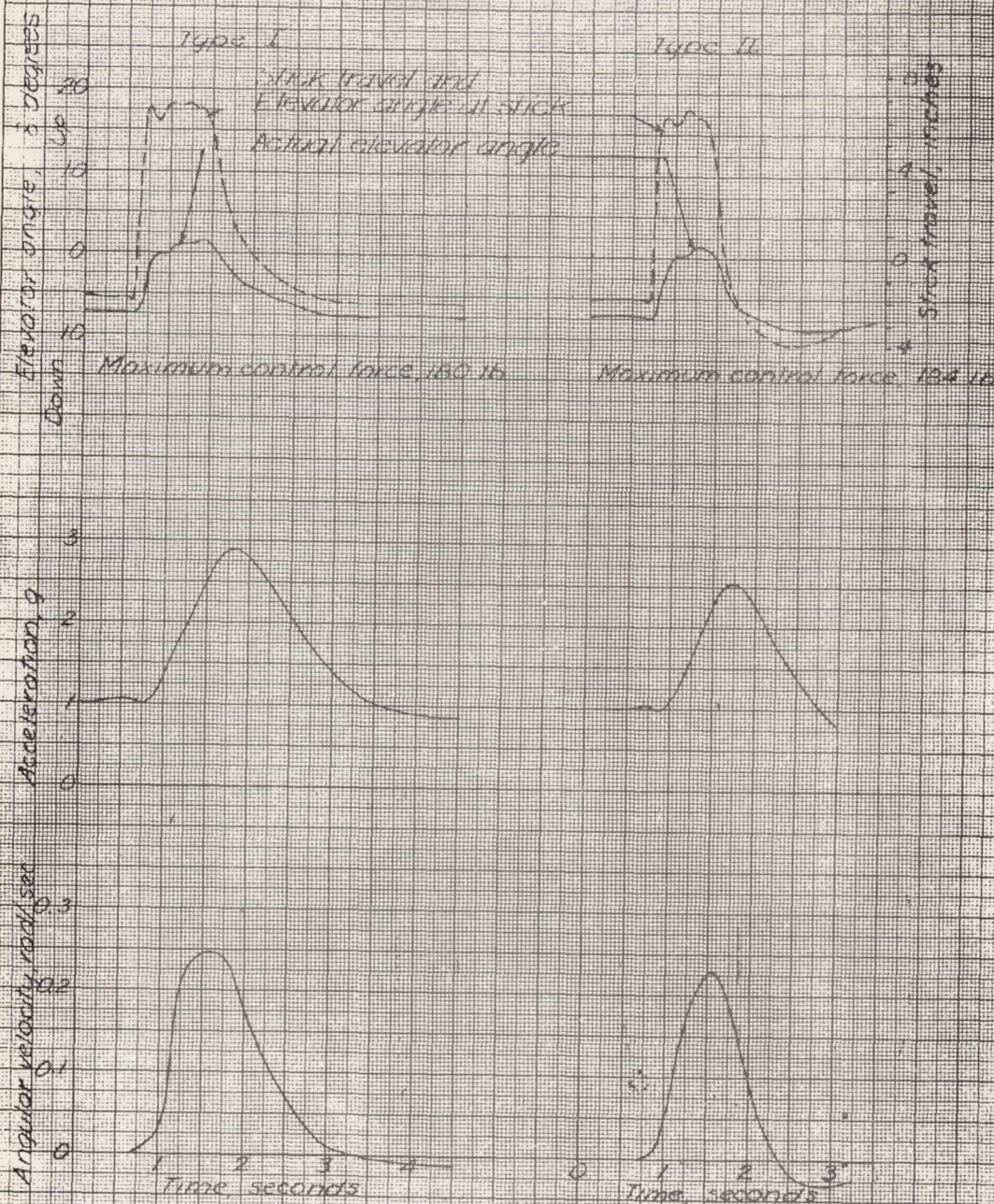
Figure 14-Variations of measured quantities obtained on the PBM-3 airplane for two types of pull-ups, c.g. at 26% MAC, initial airspeed 219 mph (ind.)
