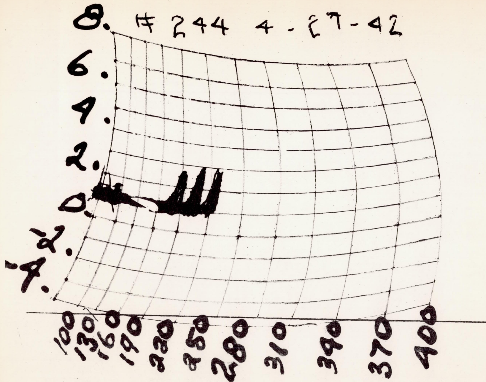
Figure 9.- V-G records obtained in 24 pull-ups on PBM-3 airplane.
