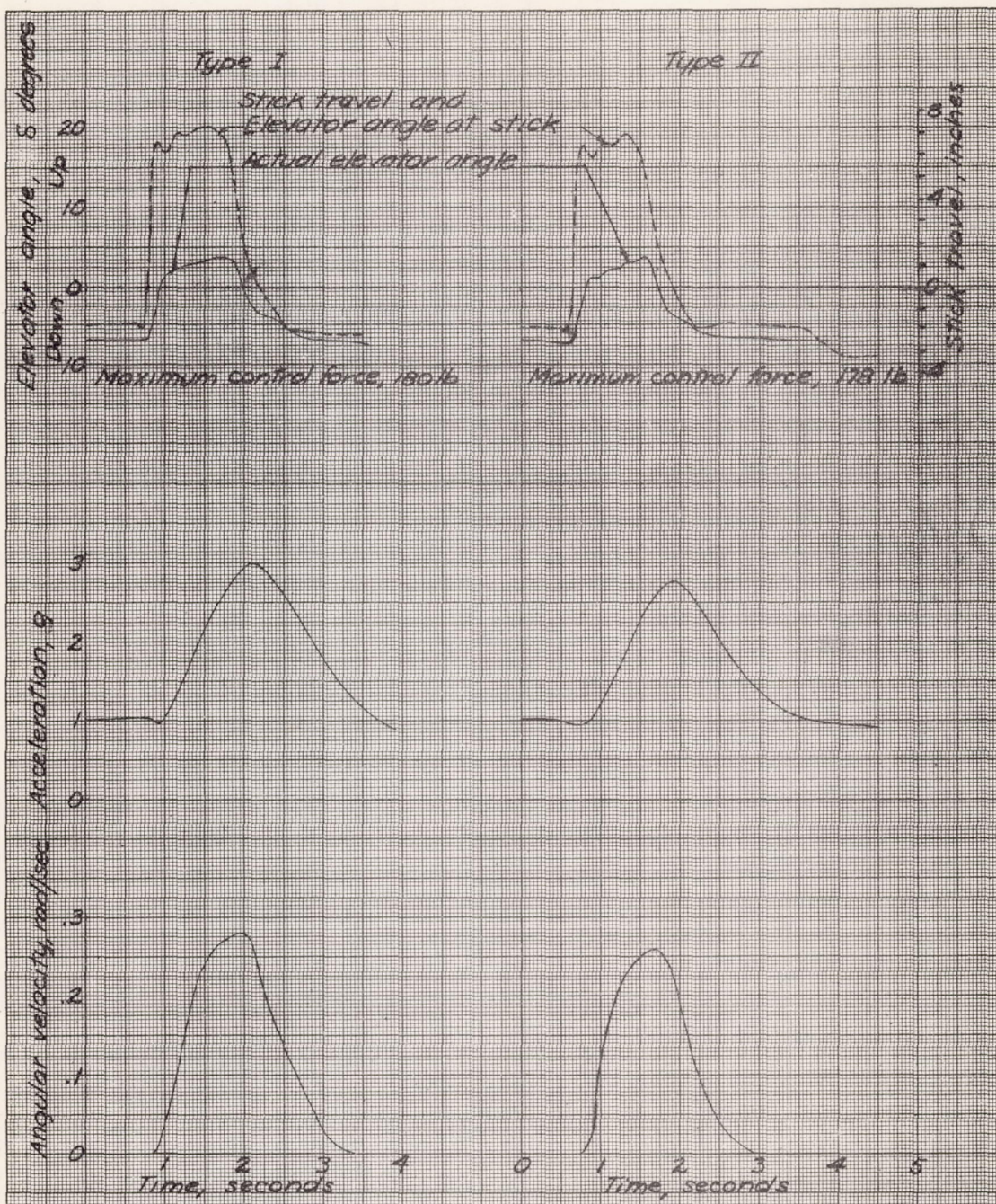
Figure 12.- Variations of measured quantities obtained on the PBM-3 airplane for two types of pull-ups. c.g. at 26% MAC, initial airspeed-201 mph (ind.)
