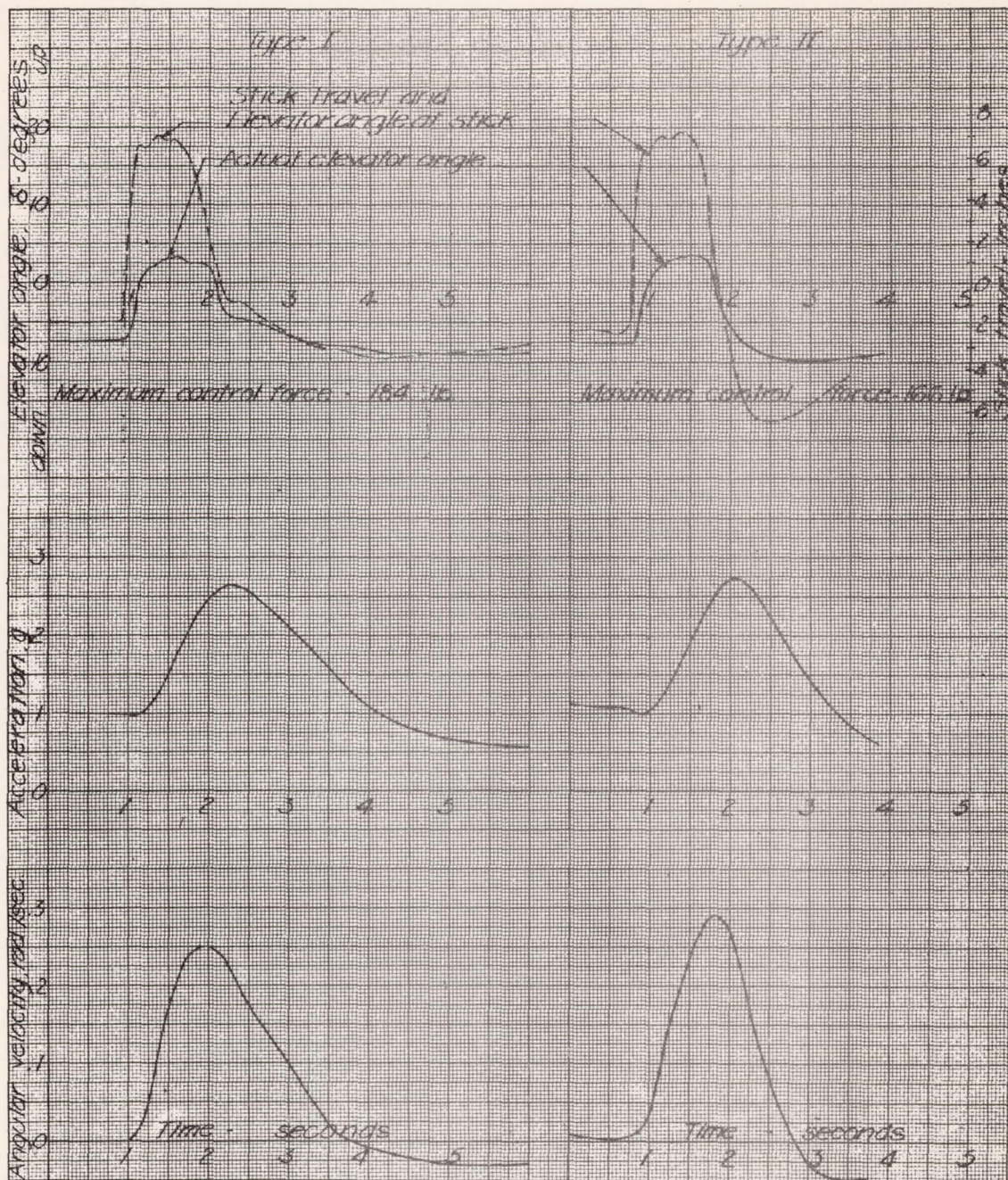
Figure 16.- Variations of measured quantities obtained on the PBM-3 airplane for two types of pull-ups. c.g. at 50% MAC, initial airspeed - 184 mph. (and)
