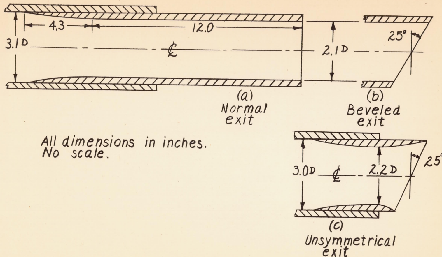
Figure 2.- Details of nozzles used to determine the effect of exit bevel on jet inclination. Tests in still air.
