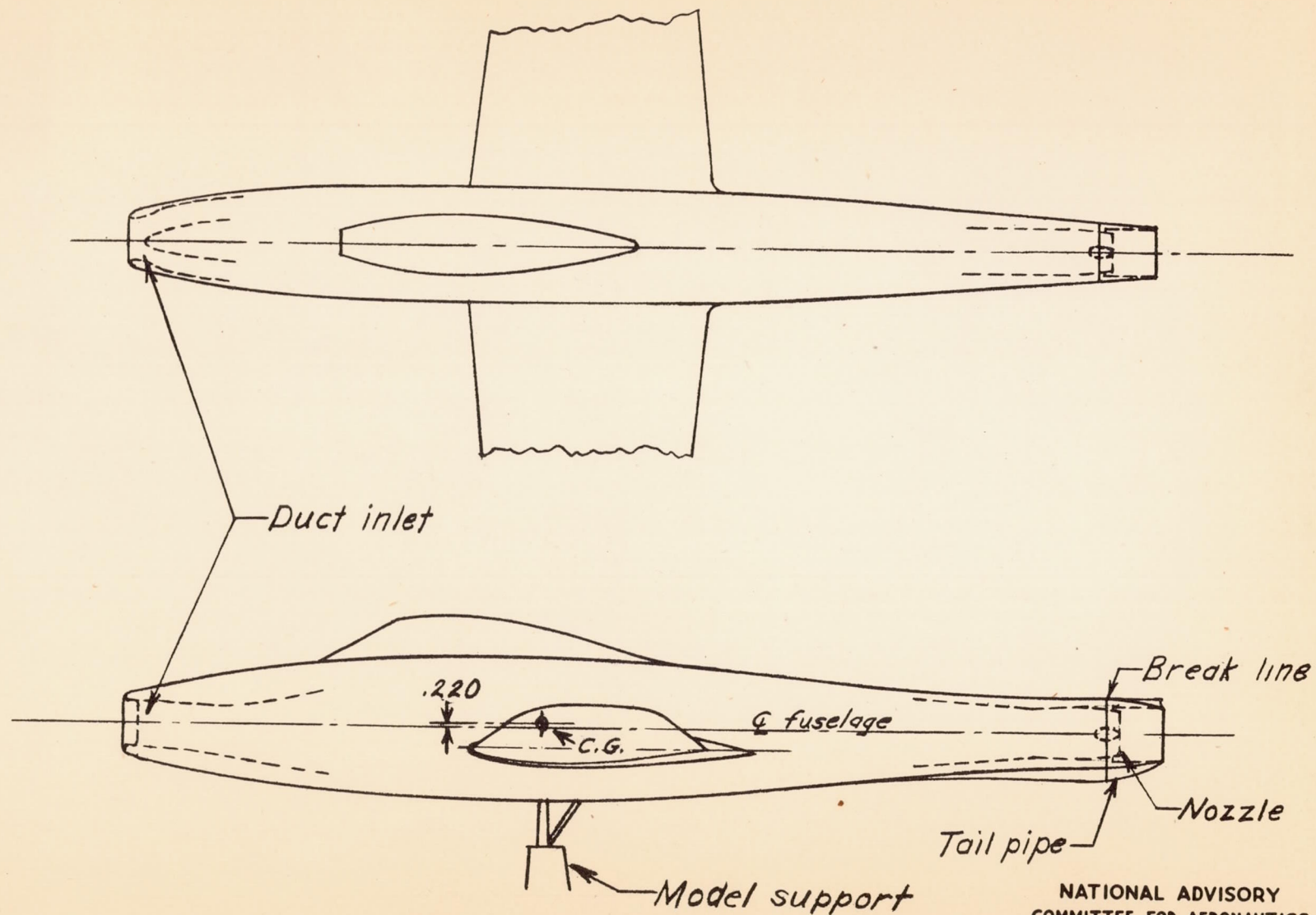
Figure 6.-Model used for tests in 7-by 10-foot tunnel.
