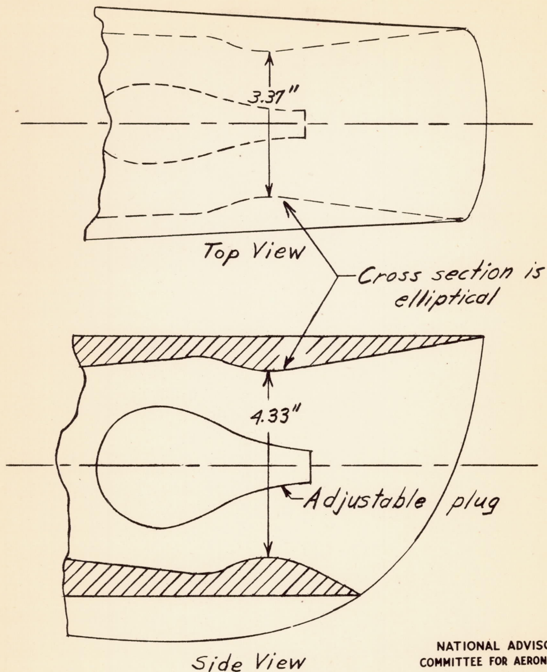
Figure 7.- Original nozzle on complete wind-tunnel model.
