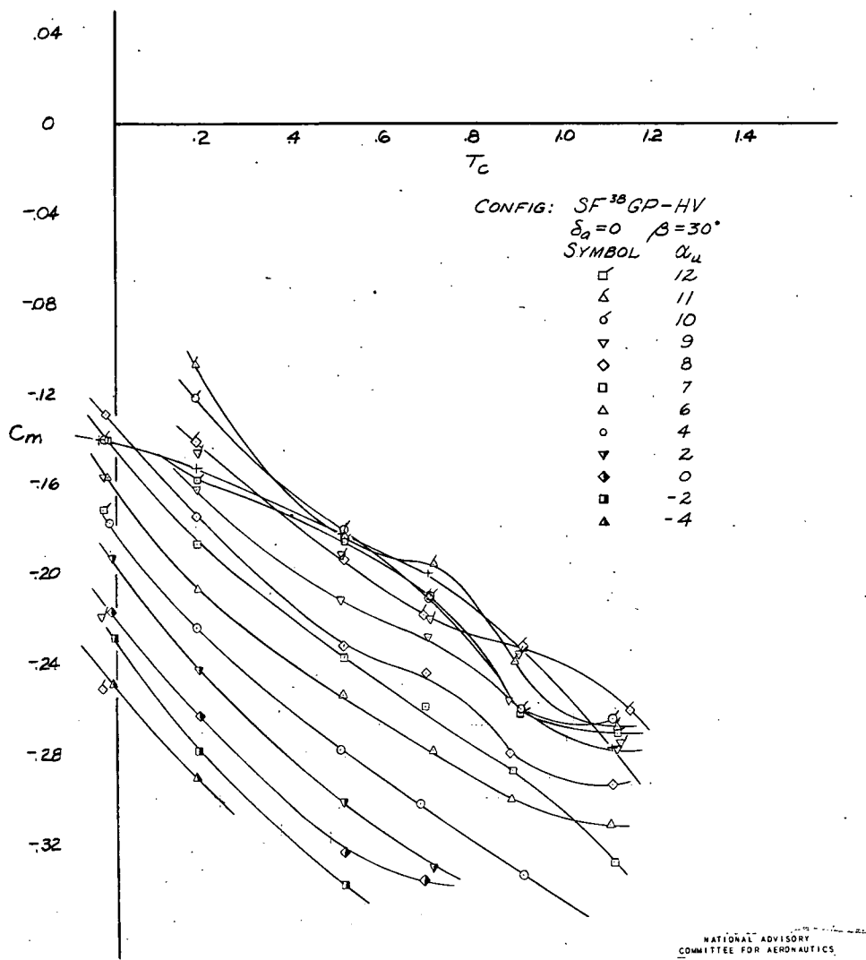
FIGURE 29B.- CHARACTERISTICS IN PITCH OF THE TEST MODEL. TAIL OFF. FLAPS 38°, GEAR EXTENDED, T_c VARIABLE
