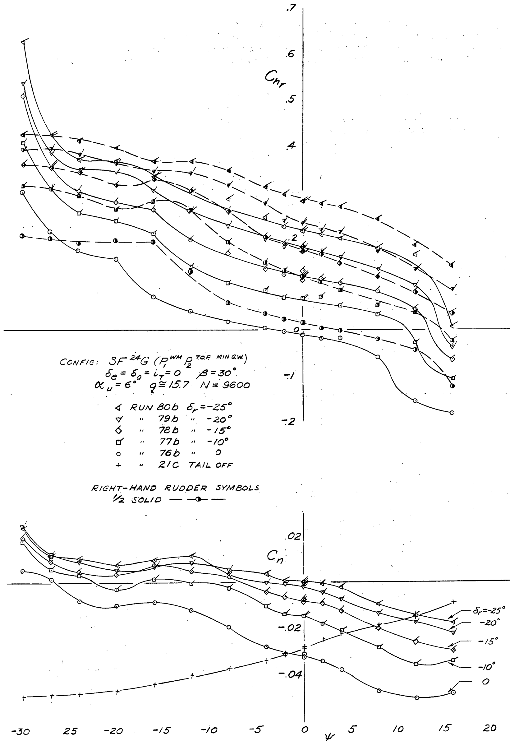
FIGURE 49.— VARIATION OF YAWING MOMENT AND RUDDER HINGE-MOMENTS WITH ANGLE OF YAW FOR THE TEST MODEL. FLAPS DEFLECTED 24^\circ ; GEAR EXTENDED, LEFT-HAND MOTOR WINDMILLING, RIGHT-HAND MOTOR TAKE-OFF POWER, GROSS WEIGHT 21,380 LBS.
