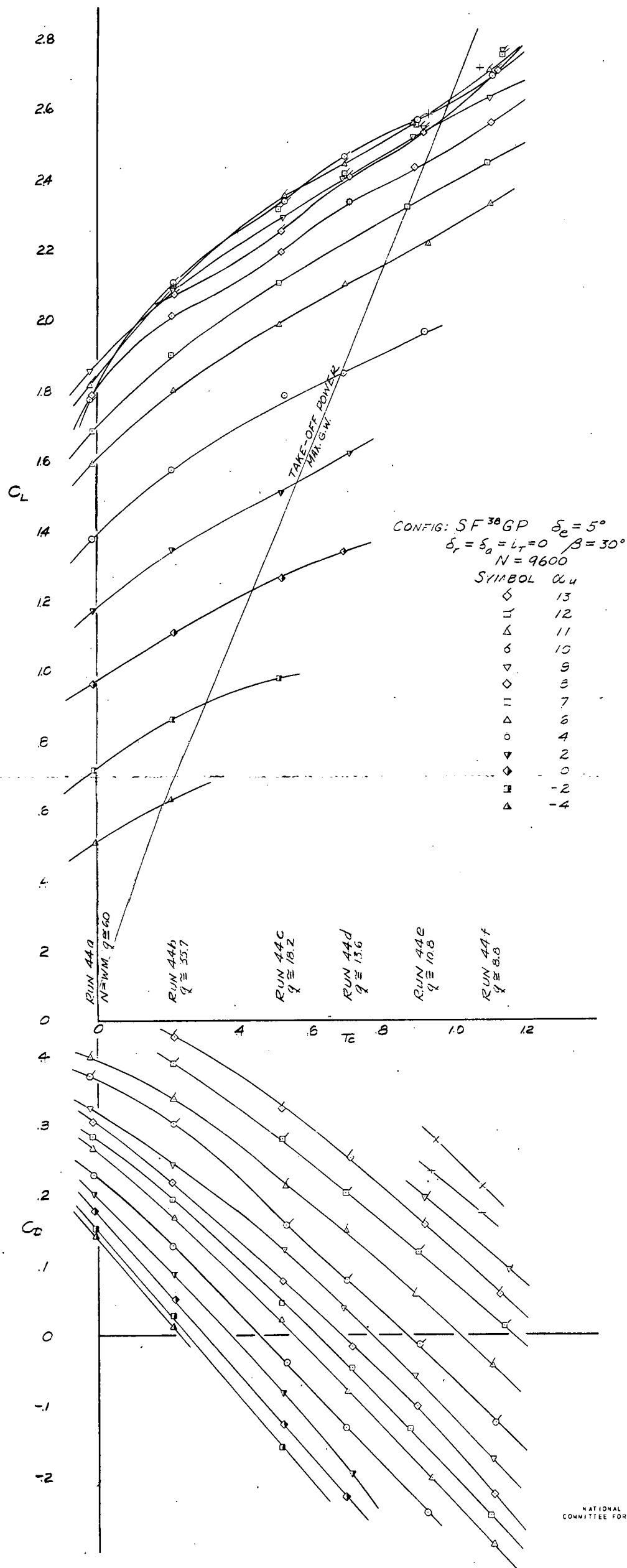
FIGURE 28A-CHARACTERISTICS IN PITCH OF THE TEST MODEL WITH ELEVATOR DEFLECTED 5^\circ . FLAPS 30^\circ , GEAR EXTENDED, T_c VARIABLE.
