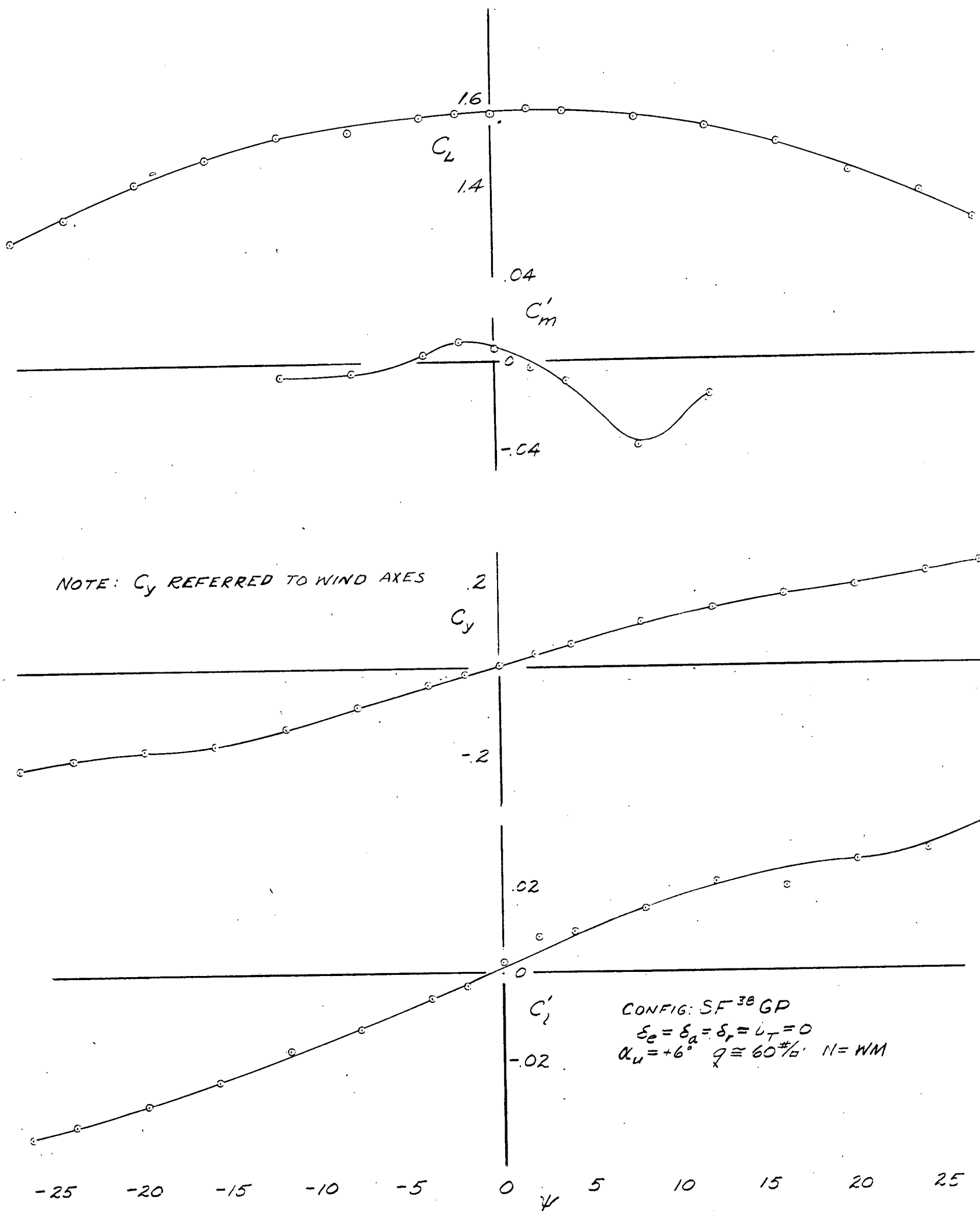
FIGURE 41.- VARIATION OF C_L , C_m' , C_y AND C_i' WITH ANGLE OF YAW FOR THE TEST MODEL. FLAPS 38^\circ , GEAR EXTENDED, PROPELLERS WINDMILLING.
