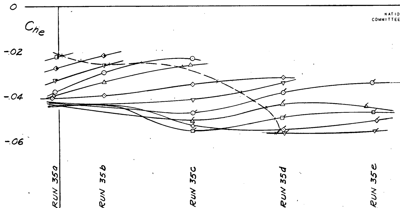
FIGURE 22B: CHARACTERISTICS IN PITCH OF THE TEST MODEL WITH ELEVATOR DEFLECTED +5^\circ . FLAPS AND GEAR RETRACTED, T_c VARIABLE.
