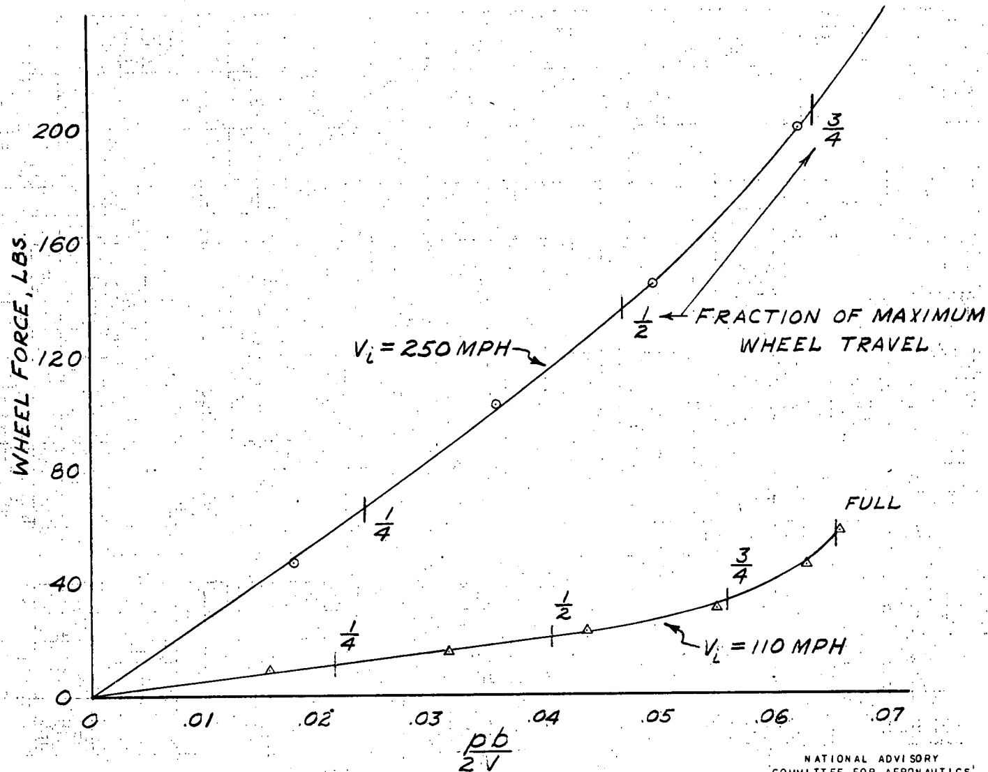
FIGURE 11.- VARIATION OF WHEEL FORCE WITH pb/2V . RUDDER LOCKED
