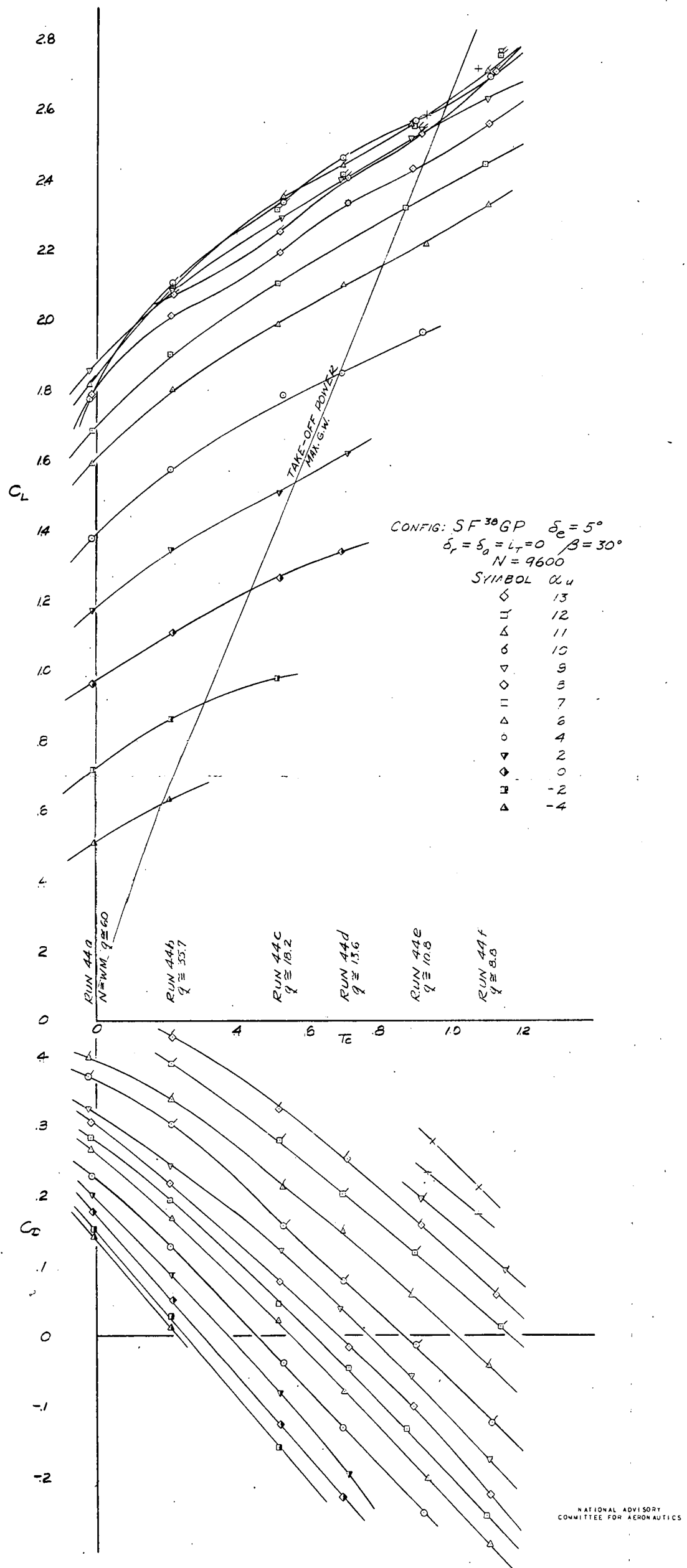
FIGURE 28A-CHARACTERISTICS IN PITCH OF THE TEST MODEL WITH ELEVATOR DEFLECTED 5^\circ , FLAPS 30^\circ , GEAR EXTENDED, T_c VARIABLE.
