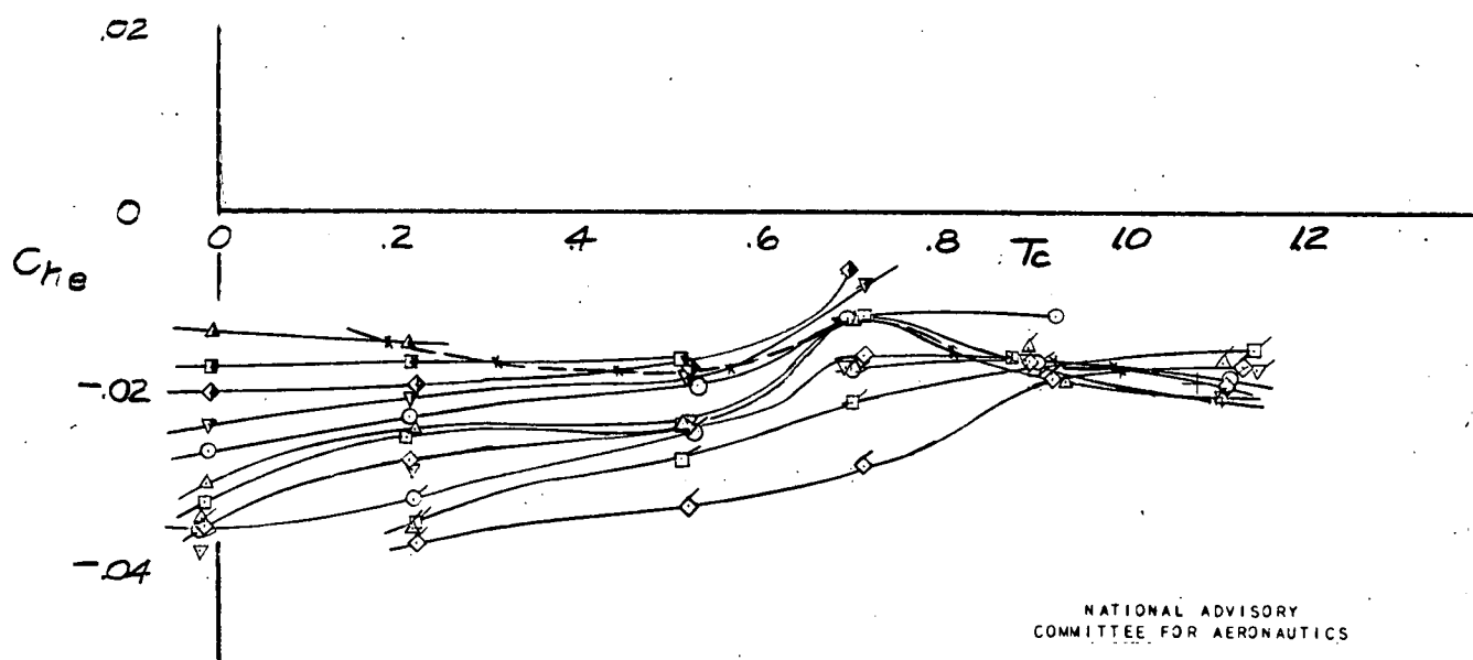
FIGURE 28B: CHARACTERISTICS IN PITCH OF THE TEST MODEL WITH ELEVATOR DEFLECTED 5^\circ , FLAPS 38^\circ , GEAR EXTENDED, T_c VARIABLE.
