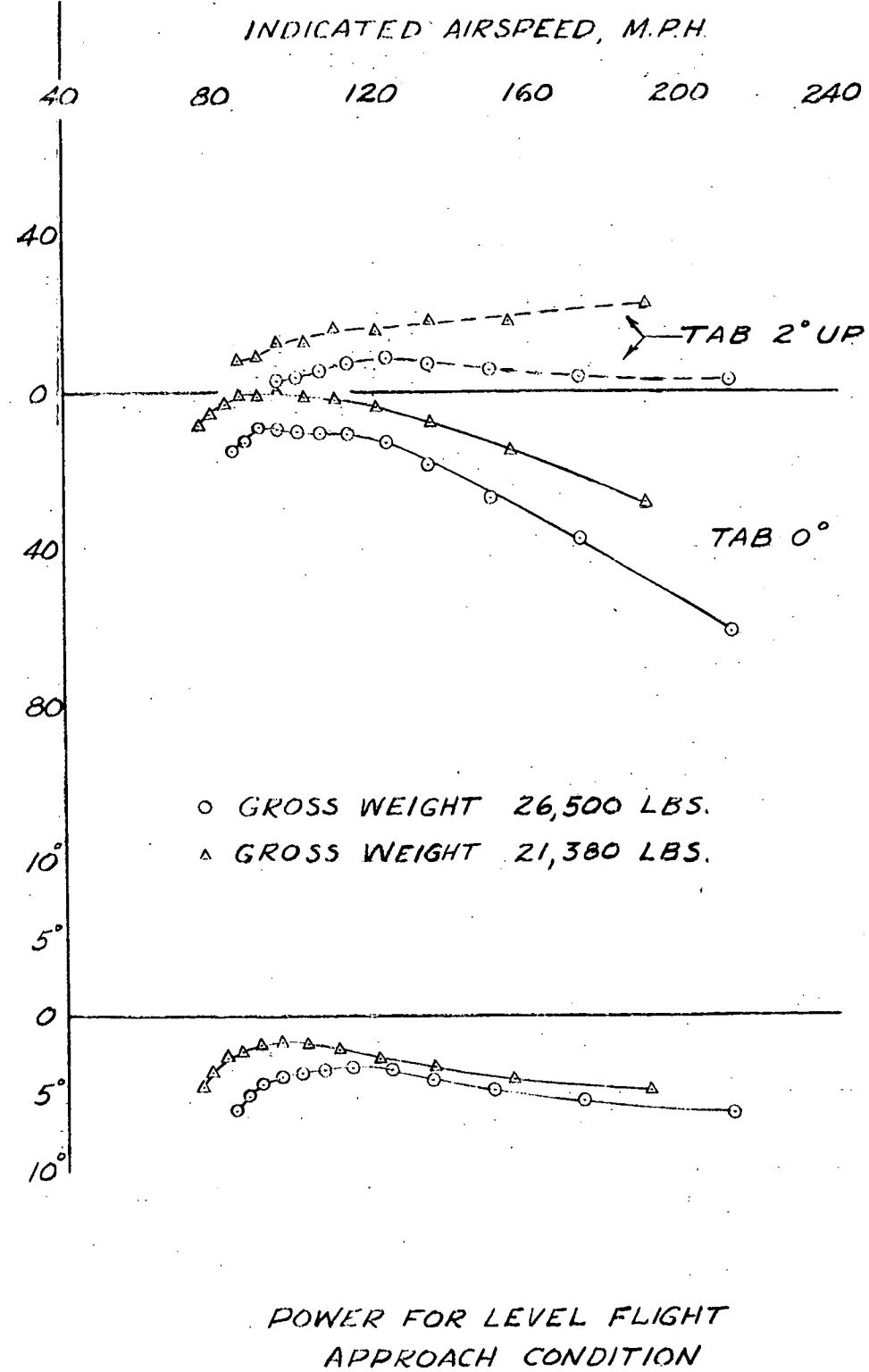
NATIONAL ADVISORY COMMITTEE FOR AERONAUTICS FIGURE 5- VARIATION OF STICK FORCE AND ELEVATOR DEFLECTION FOR TRIM WITH INDICATED AIRSPEED. FLAPS 38°, GEAR EXTENDED.
