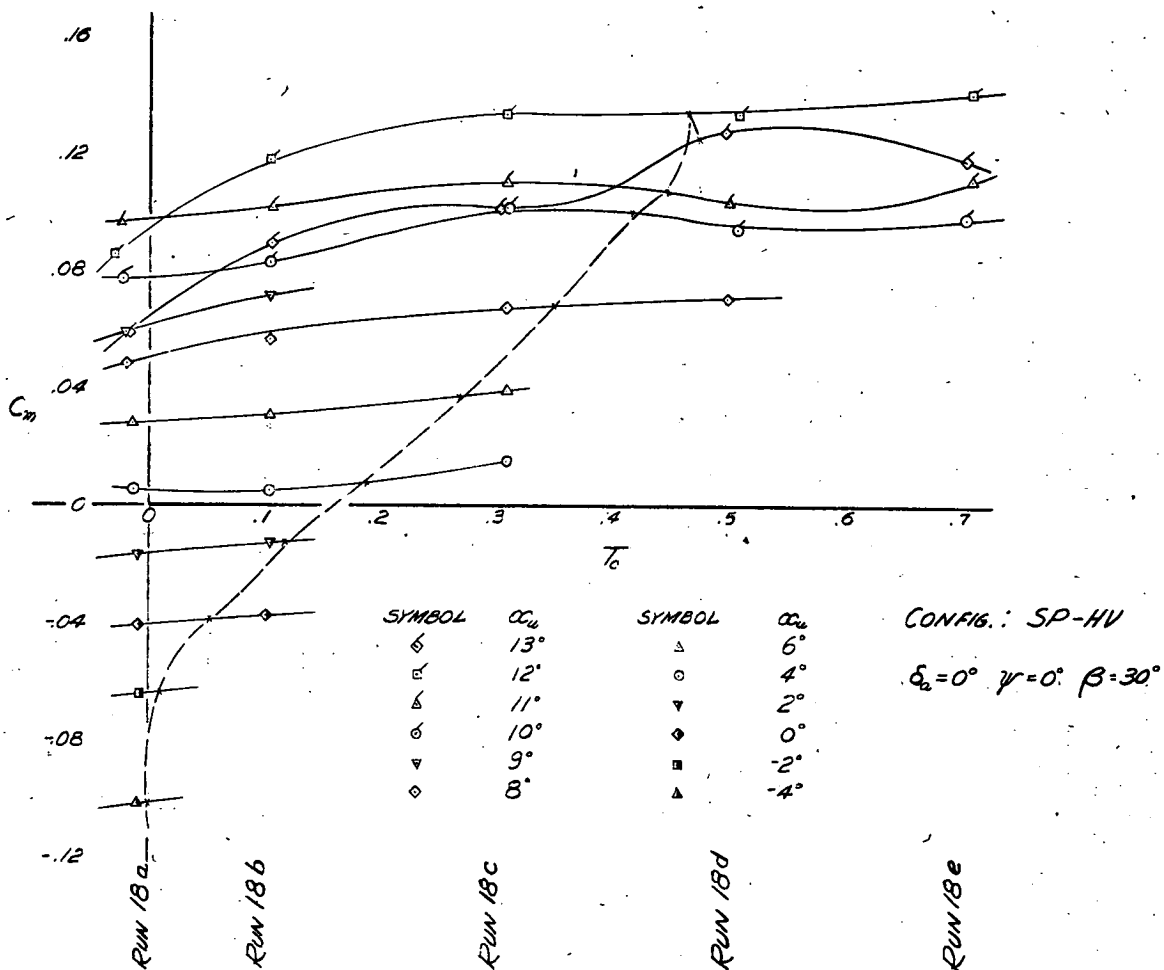
FIGURE 24-B.- CHARACTERISTICS IN PITCH OF THE TEST MODEL WITH TAIL OFF. FLAPS AND GEAR RETRACTED, T_c VARIABLE.
