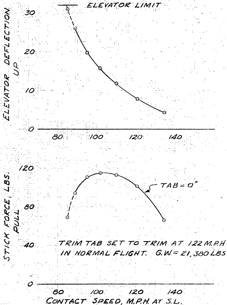
FIGURE 8- ELEVATOR DEFLECTION AND STICK FORCE TO TRIM IN THE PRESENCE OF THE GROUND VS CONTACT SPEED, FLAPS 38°, GEAR EXTENDED.
