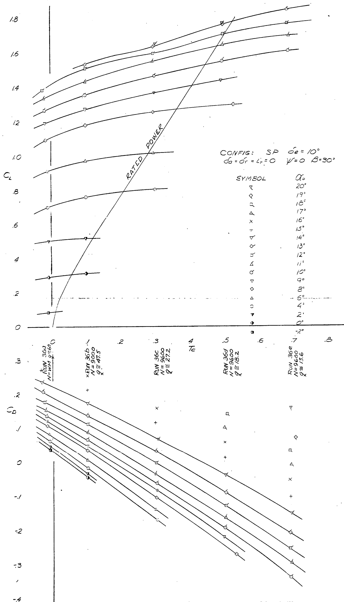
FIGURE 23A.- CHARACTERISTICS IN PITCH OF THE TEST MODEL WITH ELEVATOR DEFLECTED +10^\circ . FLAPS AND GEAR RETRACTED, T_C VARIABLE.
