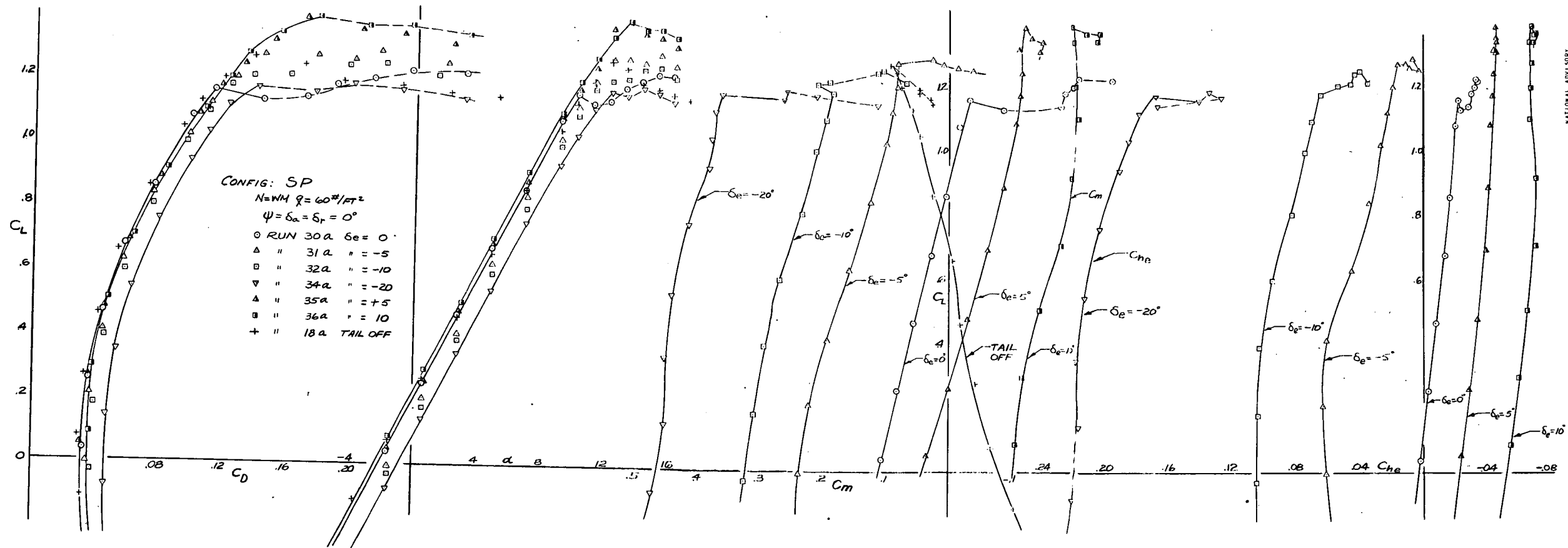
FIGURE 18.- CHARACTERISTICS IN PITCH OF THE TEST MODEL WITH ELEVATOR DEFLECTED, FLAPS AND GEAR RETRACTED, PROPELLERS WINDMILLING.
