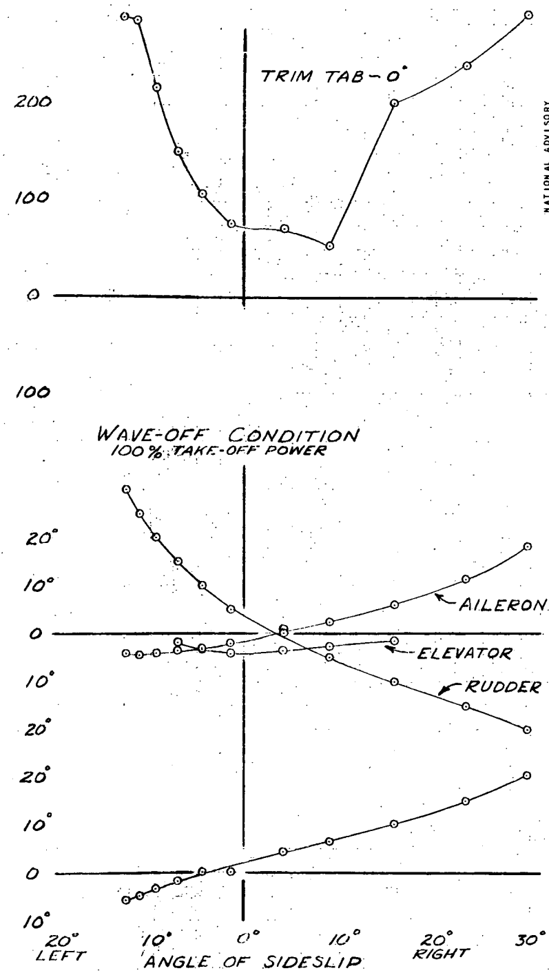
FIGURE 13-CHARACTERISTICS IN STEADY SIDESLIP. FLAPS 38°; GEAR EXTENDED, GROSS WEIGHT 26,500 LBS., INDICATED AIRSPEED 105 M.P.H.
