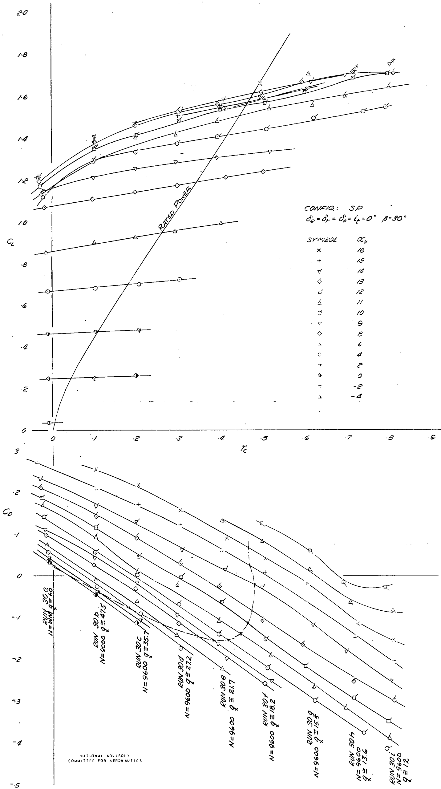
FIGURE 21A: CHARACTERISTICS IN PITCH OF THE TEST MODEL WITH ELEVATOR UNDEFLECTED. FLAPS AND GEAR RETRACTED, T_c VARIABLE
