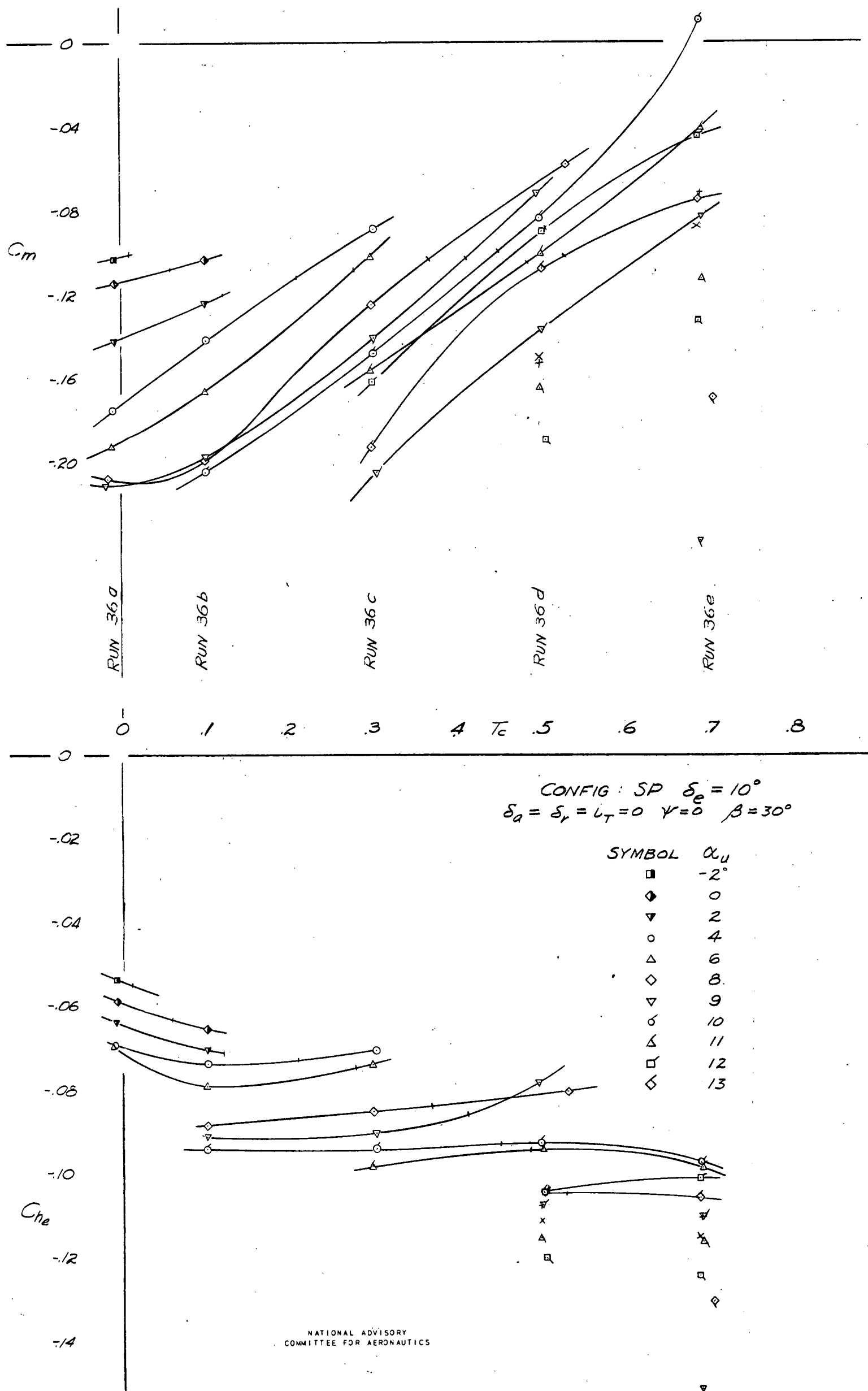
FIGURE 23B.- CHARACTERISTICS IN PITCH OF TEST MODEL WITH ELEVATOR DEFLECTED +10^\circ . FLAPS AND GEAR RETRACTED, T_c VARIABLE.
