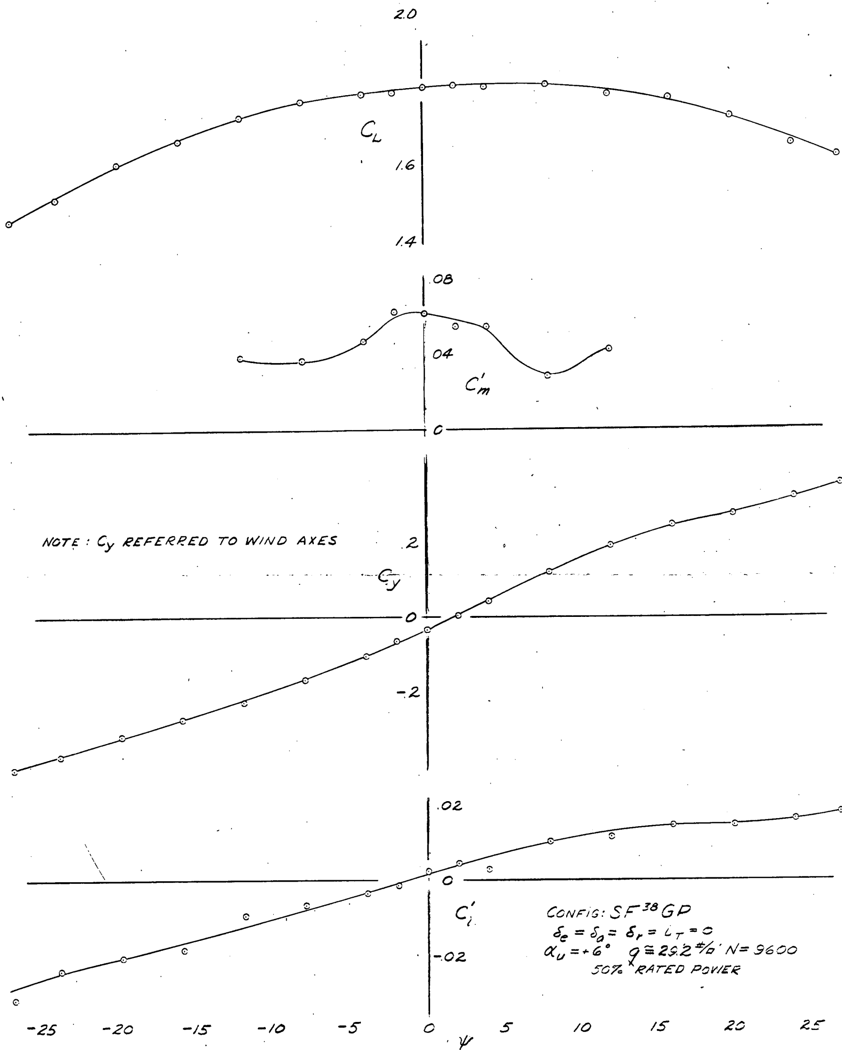
FIGURE 43.- VARIATION OF C_L , C_m' , C_y AND C_l' WITH ANGLE OF YAW FOR THE TEST MODEL. FLAPS 38^\circ , GEAR EXTENDED, 50% RATED POWER, GROSS WEIGHT 26,500 LBS.
