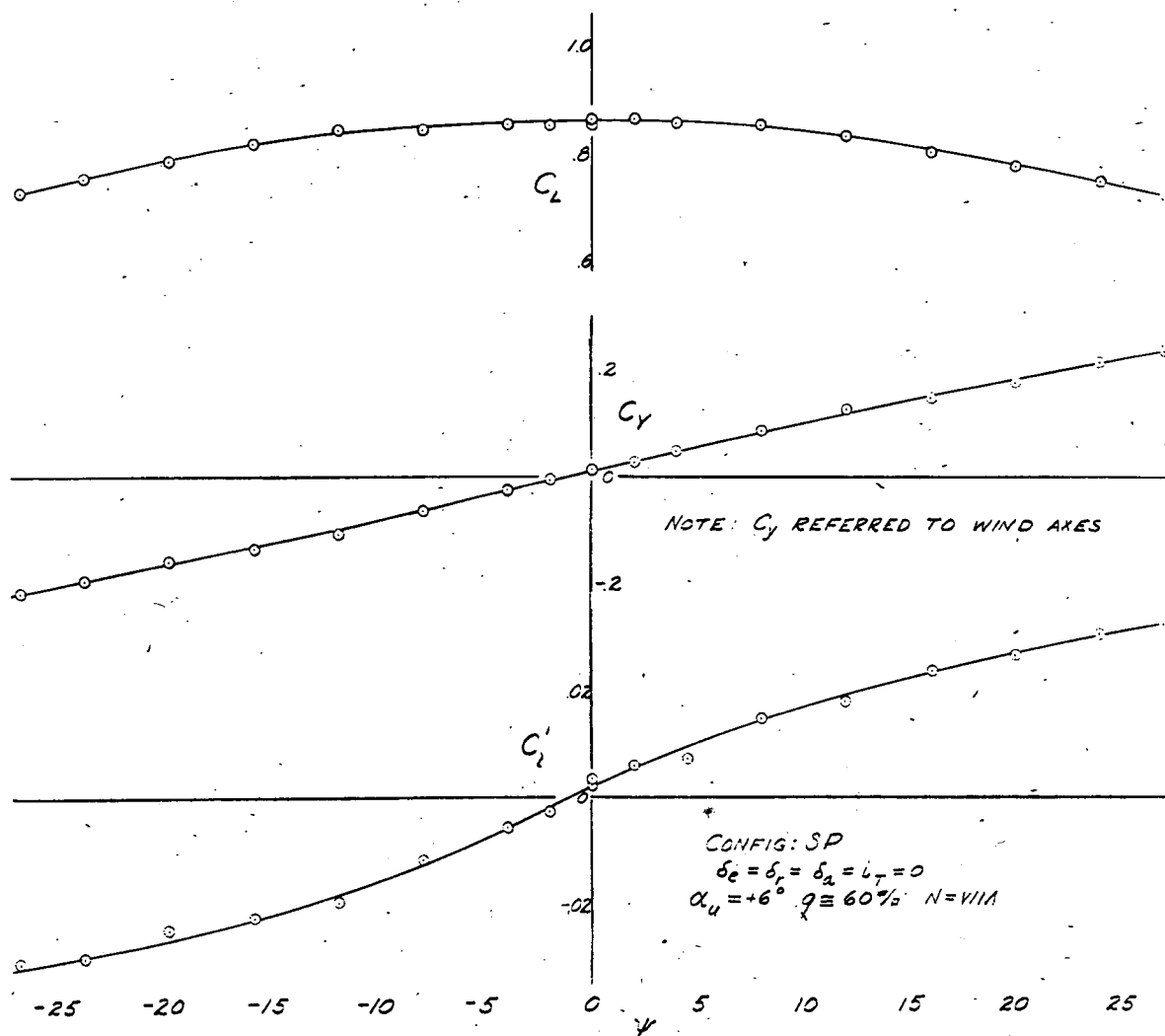
FIGURE 37.- VARIATION OF C_L , C_Y AND C_i' WITH ANGLE OF YAW FOR THE TEST MODEL. FLAPS AND GEAR RETRACTED. PROPELLERS WINDMILLING.
