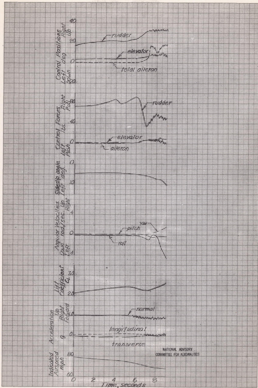
Figure 11. - Time history of a stall in the approach condition in which the pilot attempted to control the airplane through the stall. F4U airplane.
