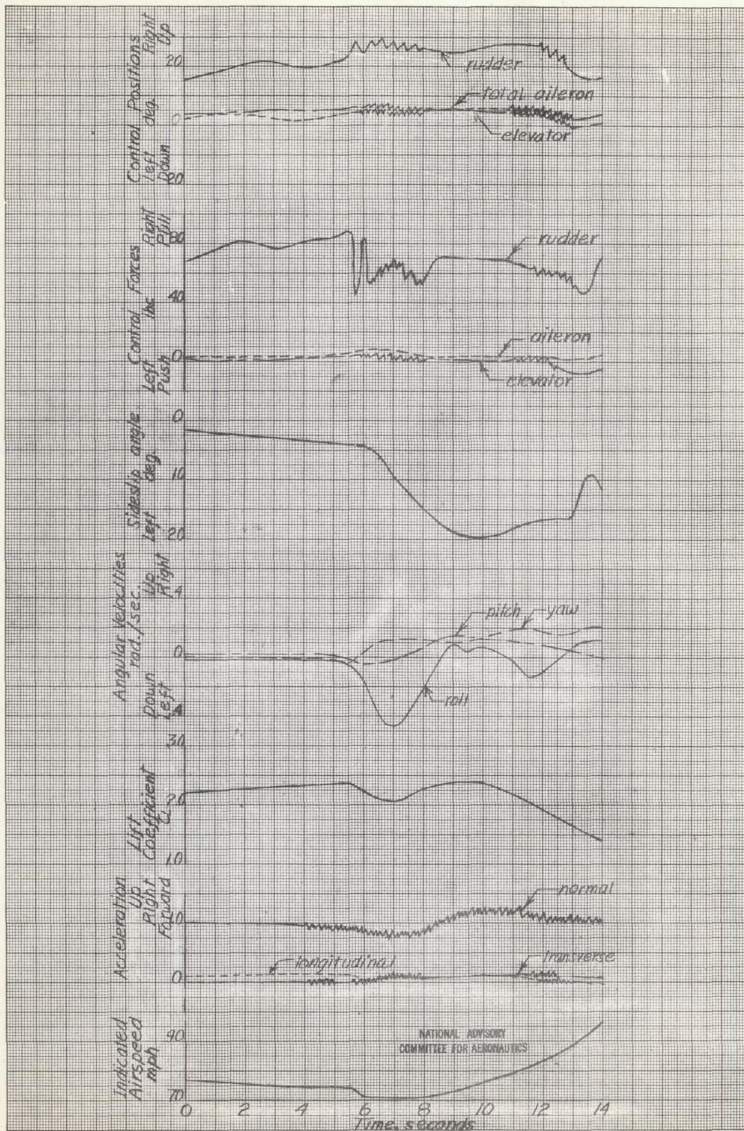
Figure 10. - Time history of a stall in the approach condition in which the pilot attempted to hold the rudder and ailerons fixed after the initial roll-off. P6F-3 airplane.
