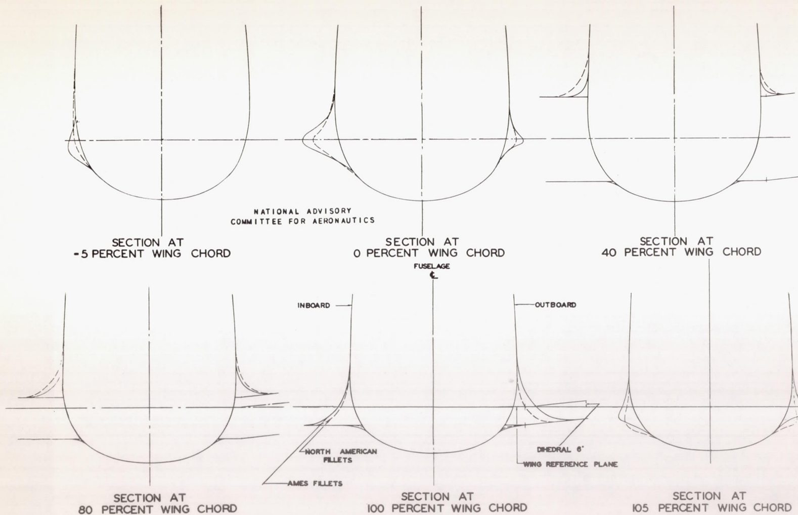
FIGURE 5:- COMPARISON OF MANUFACTURERS AND AMES FILLETS AT SEVERAL STATIONS ALONG THE WING CHORD.
